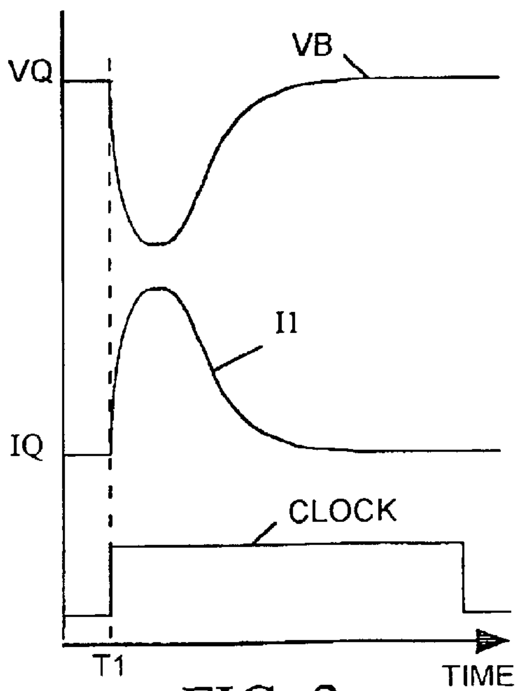
FIG. 2 (PRIOR ART)
