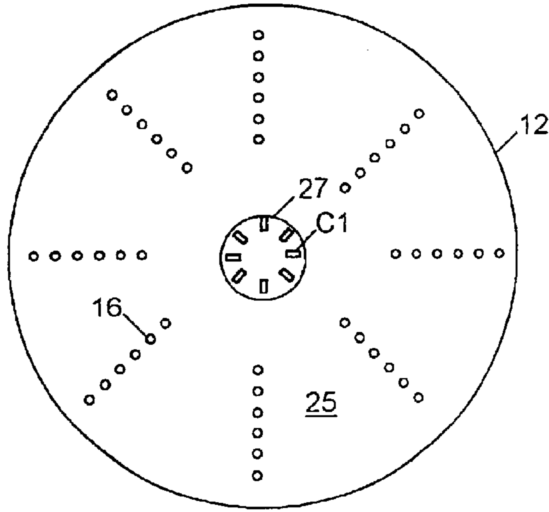
FIG. 4 (PRIOR ART)
