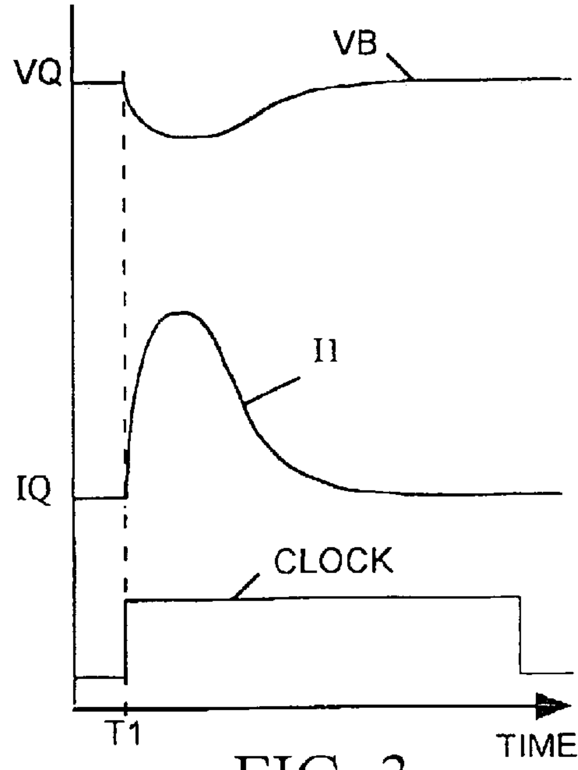
FIG. 3 (PRIOR ART)
