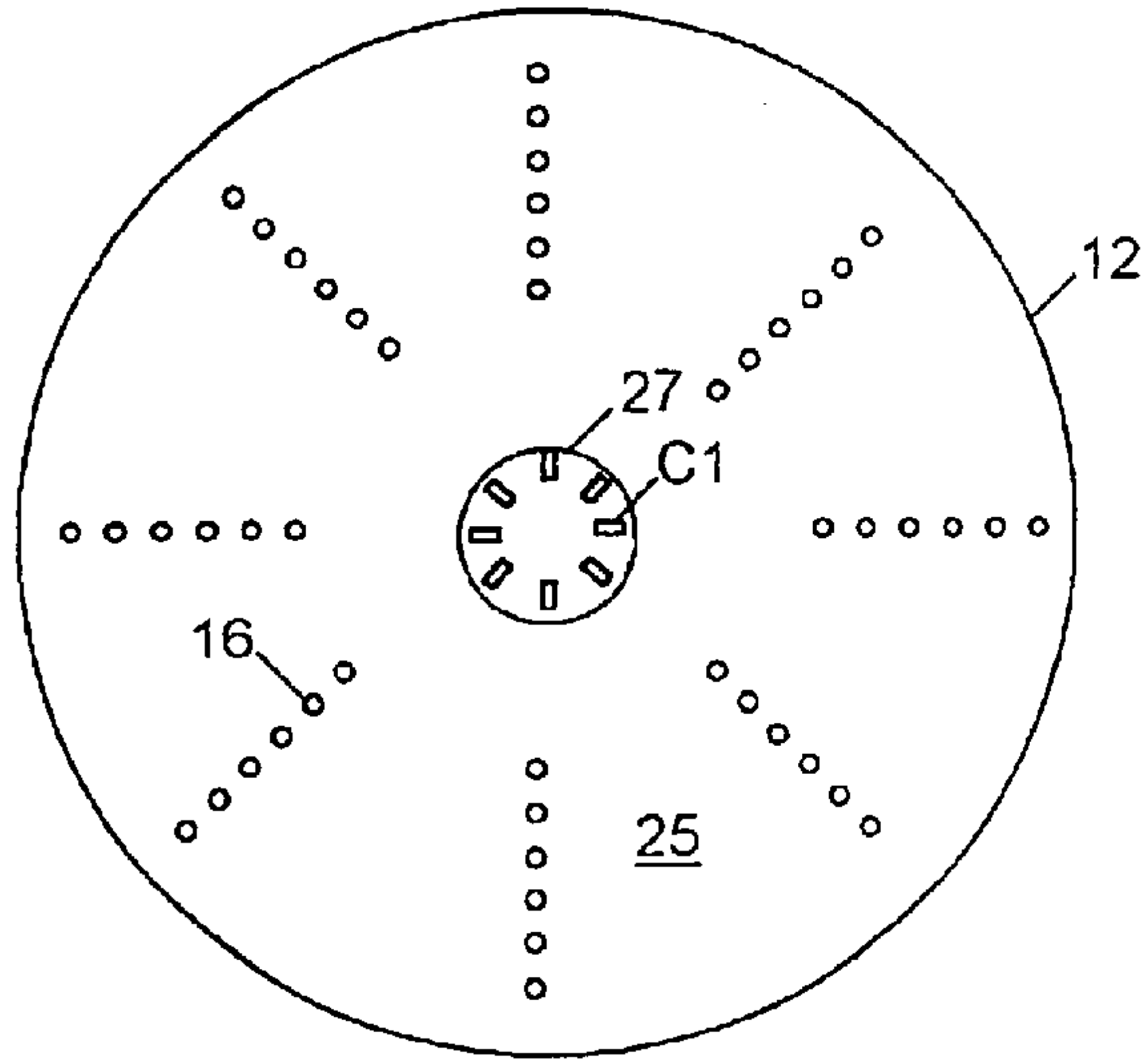
FIG. 4 (PRIOR ART)
