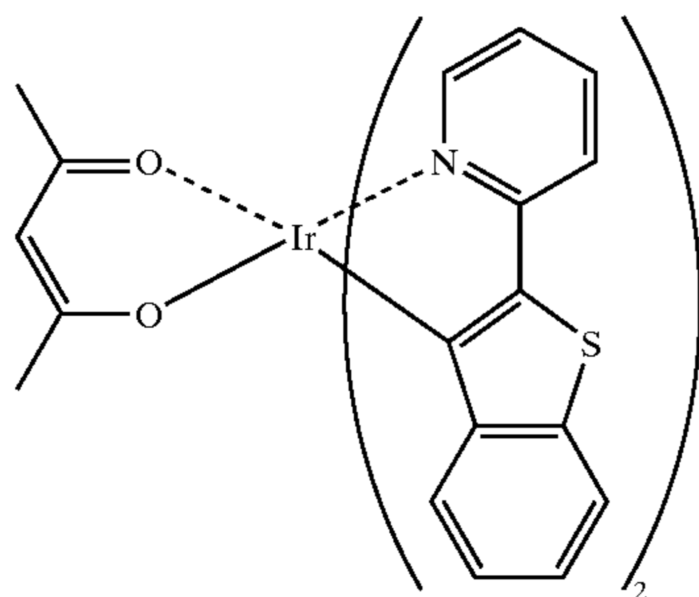
Ir(btp) 2 (acac)
