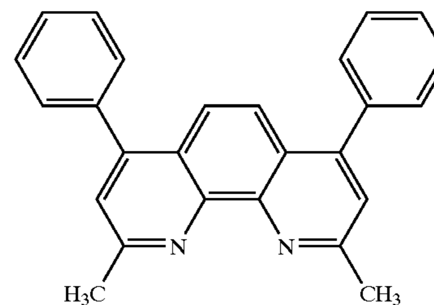
BC
