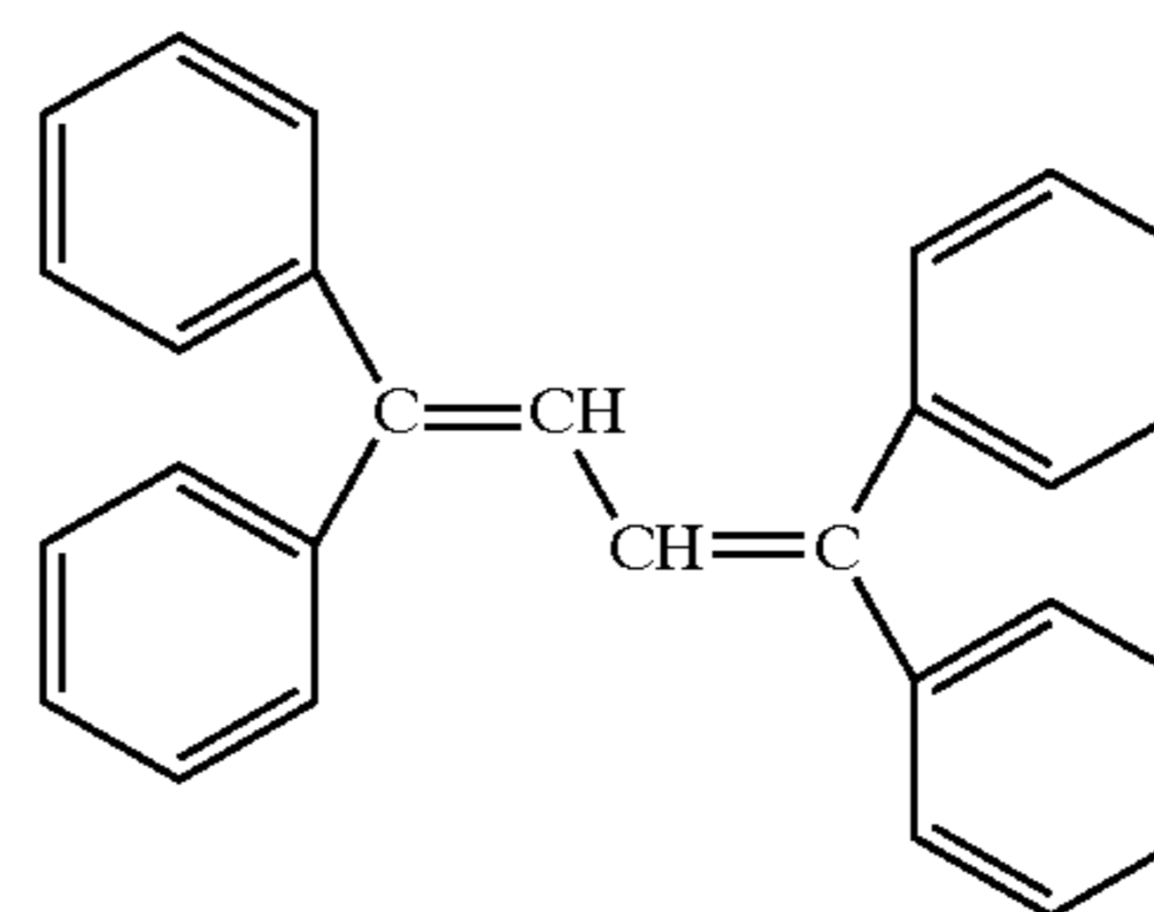
TPB
