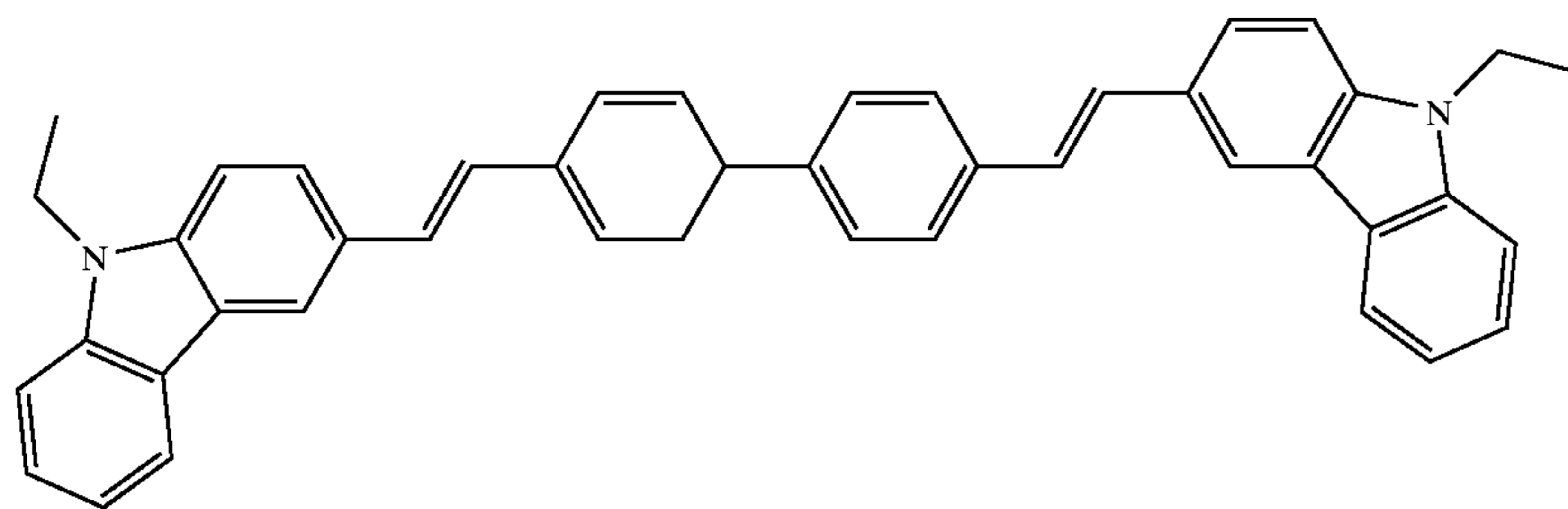
BCzVBi
