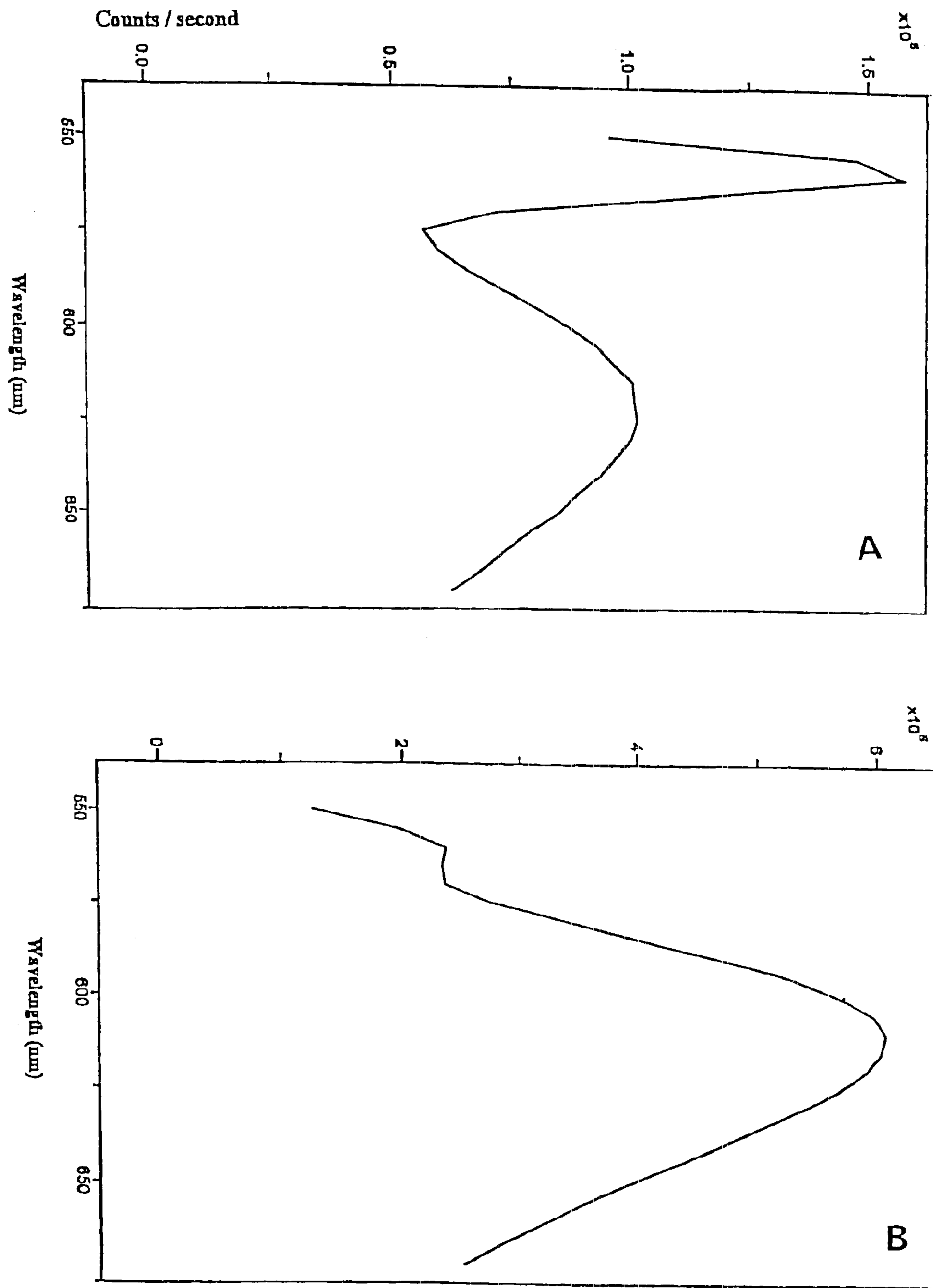
Illumination at 472 nM Figure 10
