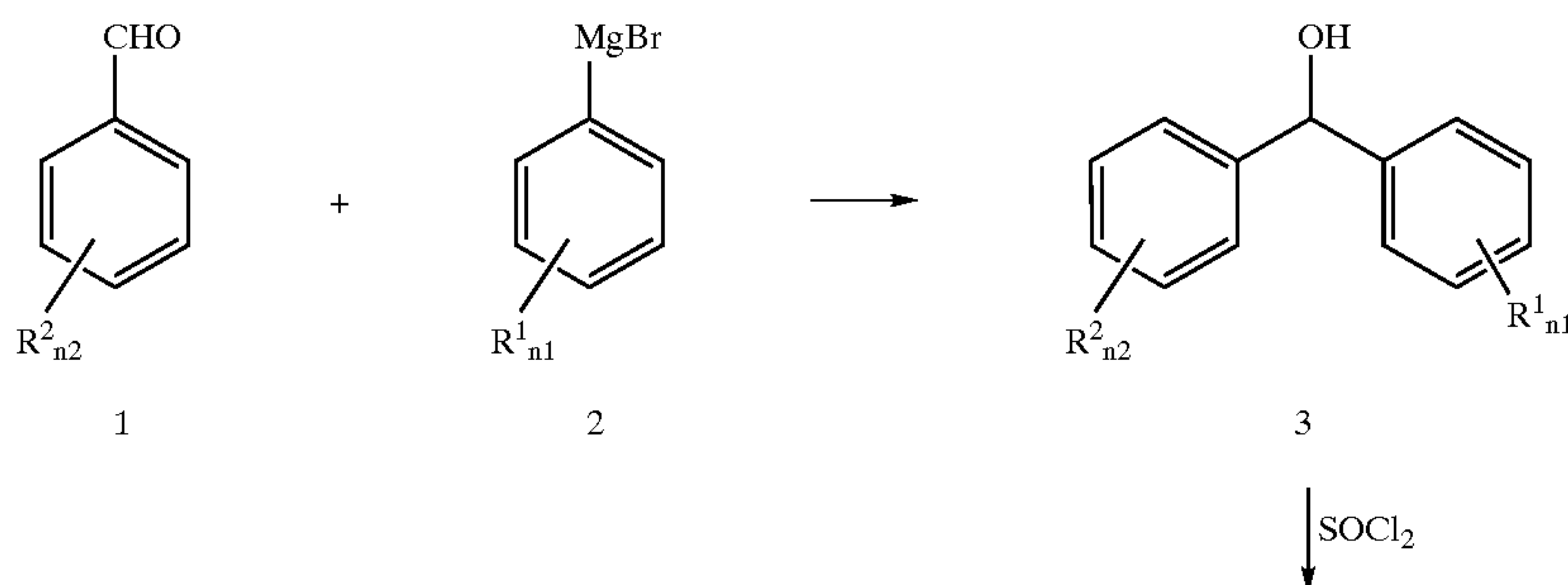
Reaction Scheme 1
