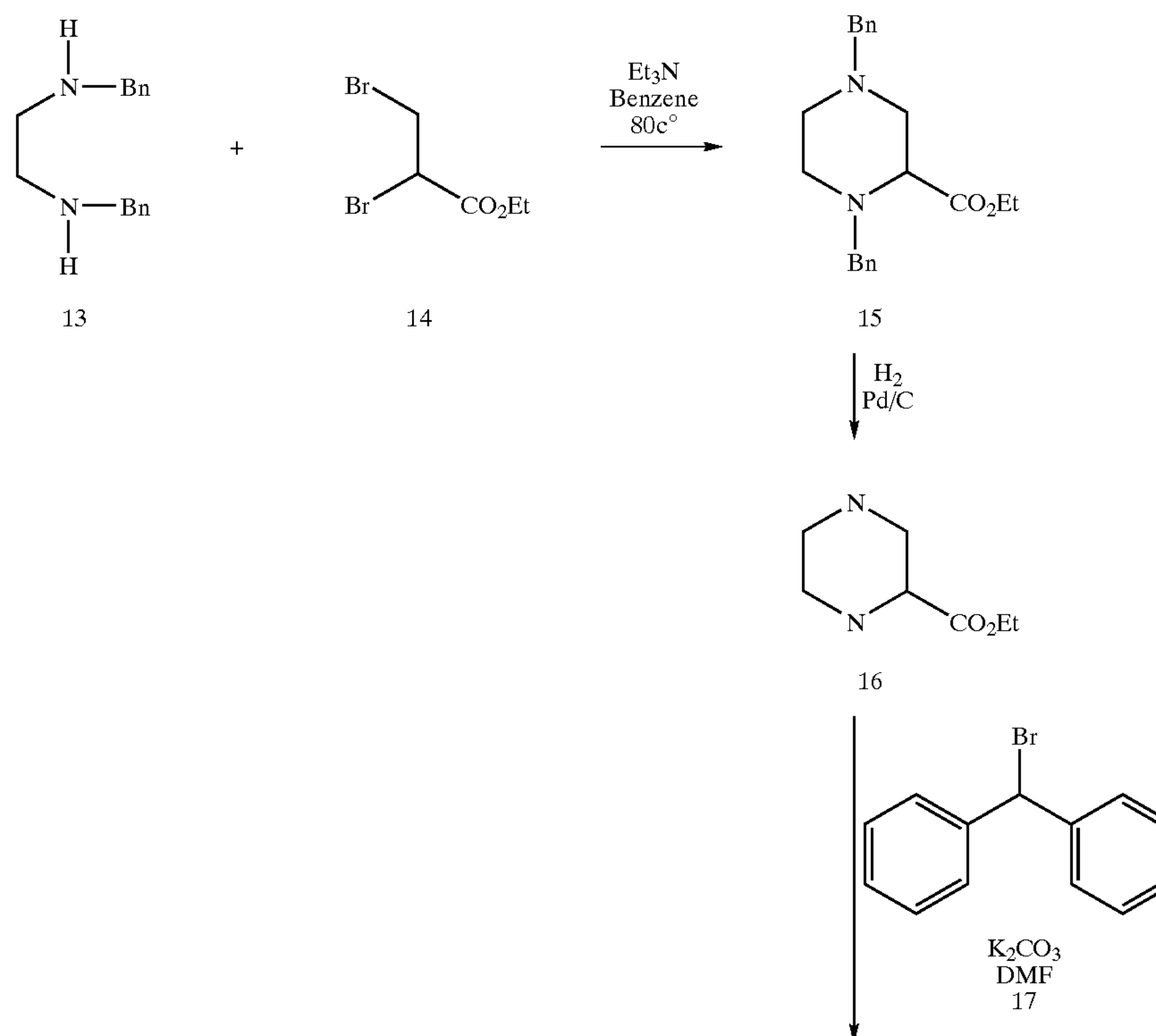
Reaction Scheme 3
