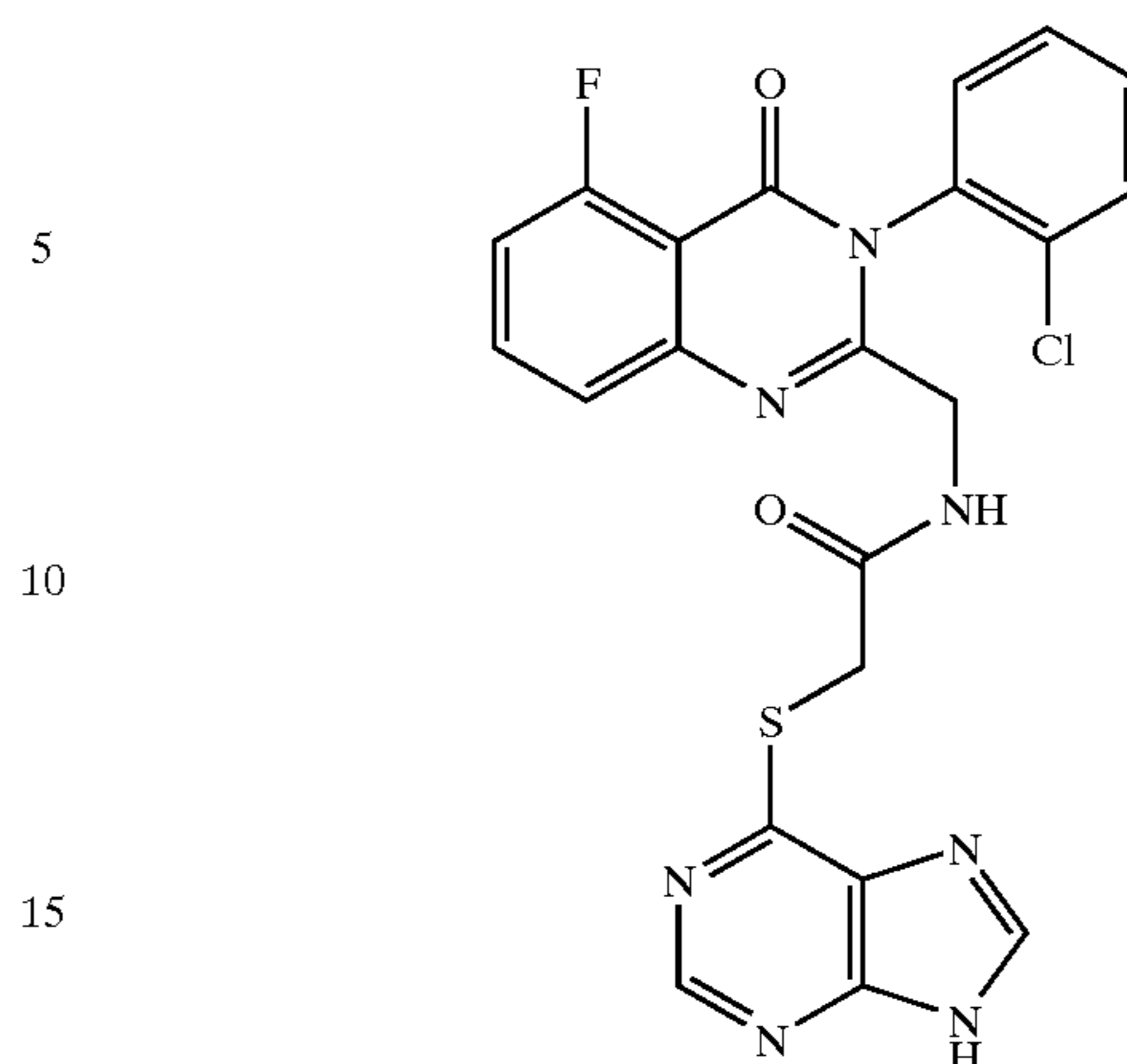
N-[3-(2-Chlorophenyl)-5-fluoro-4-oxo-3,4-dihydro-quinazolin-2-ylmethyl]-2-(9H-purin-6-ylsulfanyl)-acetamide (D-077)
