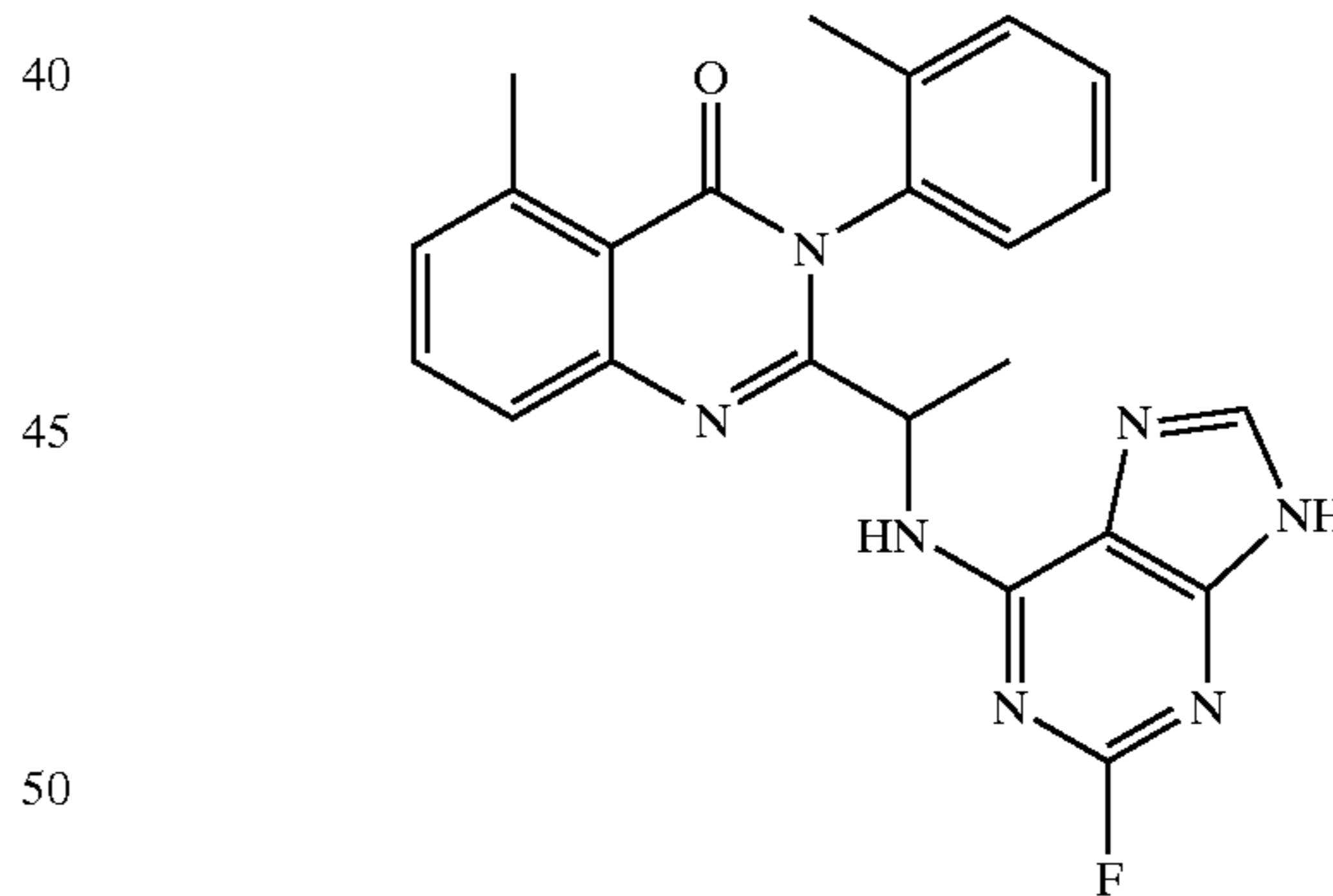
2-[1-(2-Fluoro-9H-purin-6-ylamino)ethyl]-5-methyl-3- o -tolyl-3H-quinazolin-4-one (D-080)
