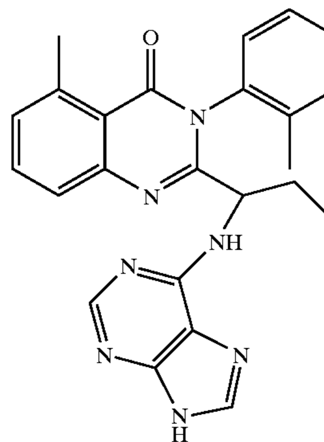
5-Methyl-2-(1-(9H-purin-6-ylamino)propyl)-3-o-tolyl-3H-quinazolin-4-one (D-081b)
