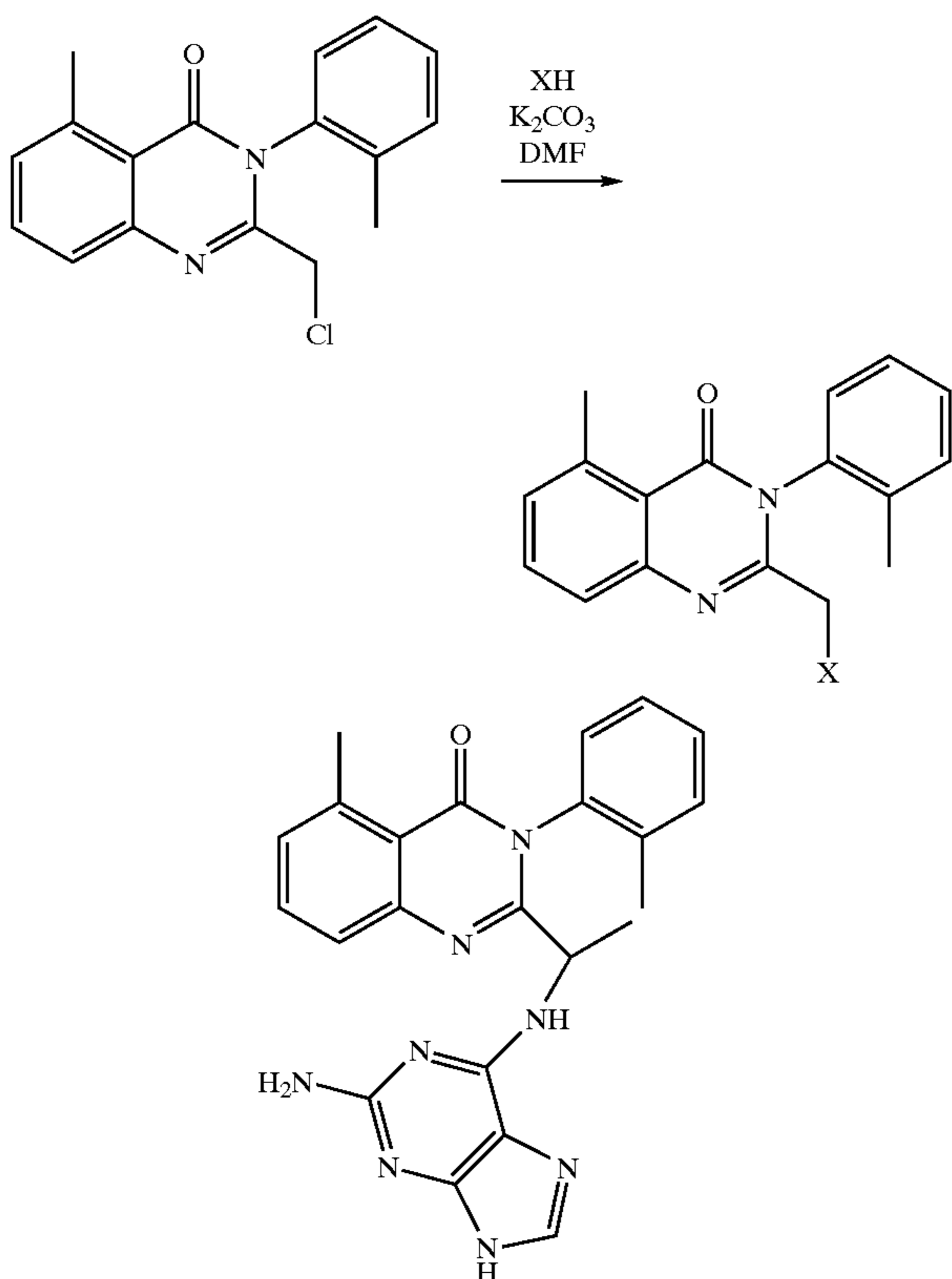
2-(1-(2-Amino-9H-purin-6-ylamino)ethyl)-5-methyl-3-o-tolyl-3H-quinazolin-4-one (D-081a)
