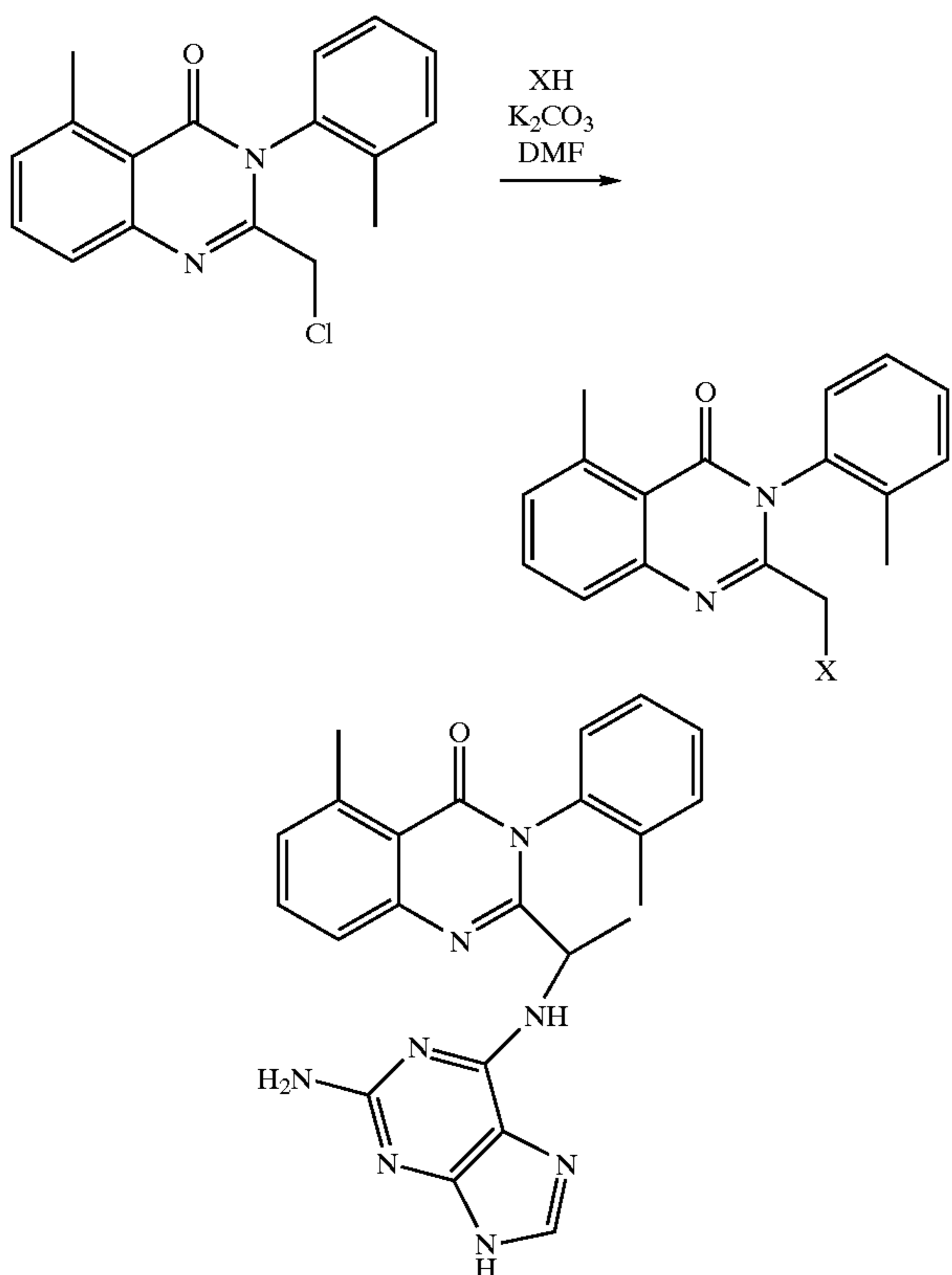
2-(1-(2-Amino-9H-purin-6-ylamino)ethyl)-5-methyl-3-o-tolyl-3H-quinazolin-4-one (D-081a)
