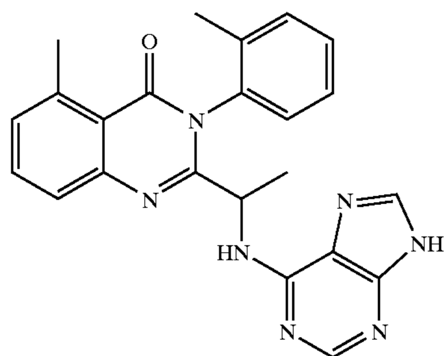
5-Methyl-2-[1-(9H-purin-6-ylamino)ethyl]-3-o-tolyl-3H-quinazolin-4-one (D-081)
