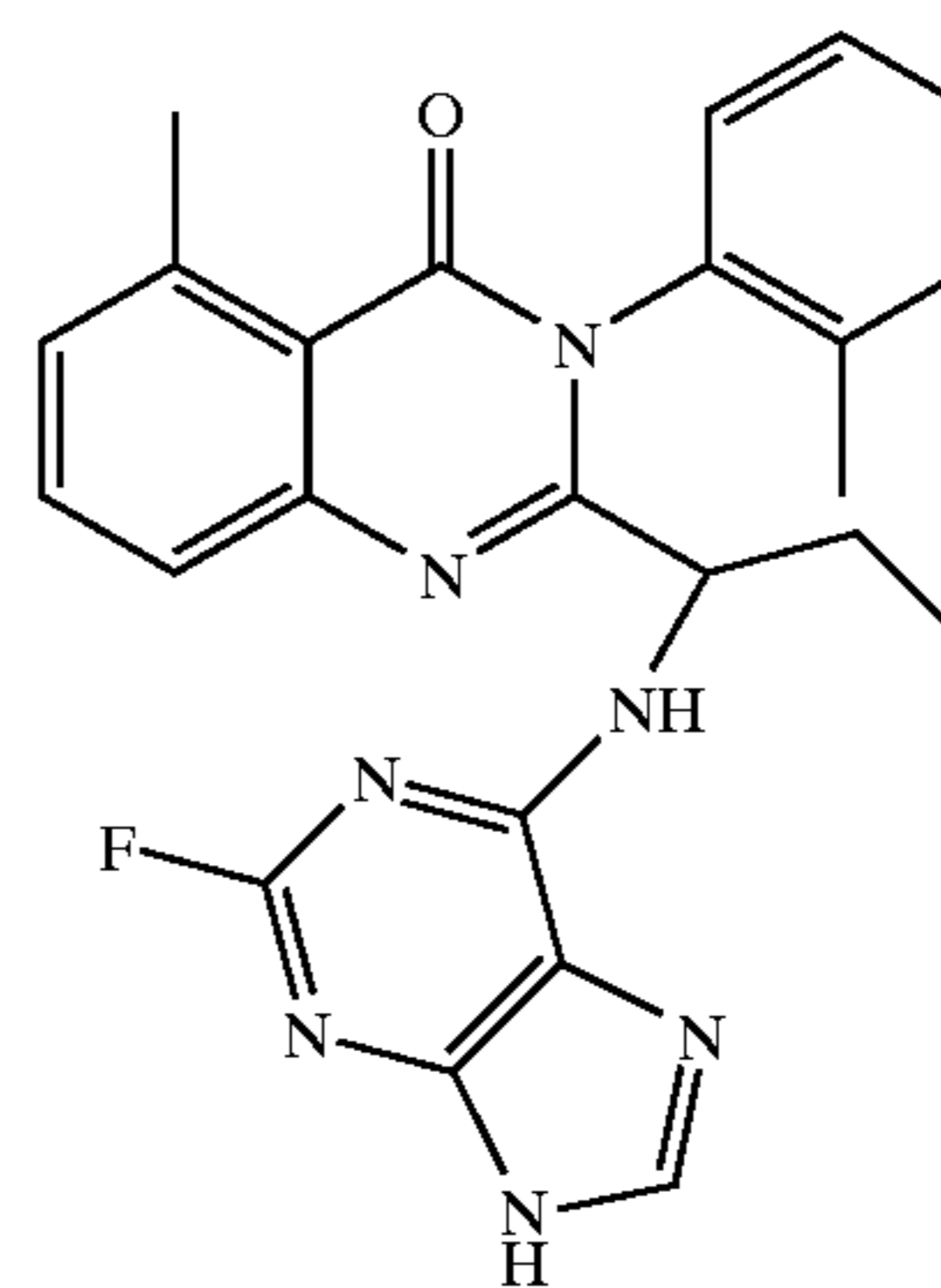
2-(1-(2-Fluoro-9H-purin-6-ylamino)propyl)-5-methyl-3-o-tolyl-3H-quinazolin-4-one (D-081c)
