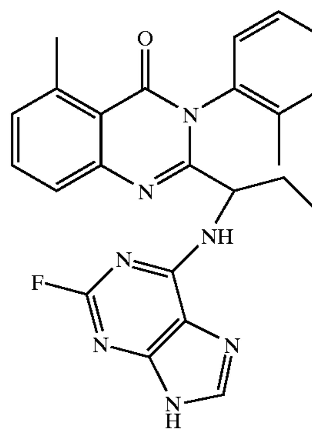
2-(1-(2-Fluoro-9H-purin-6-ylamino)propyl)-5-methyl-3-o-tolyl-3H-quinazolin-4-one (D-081c)
