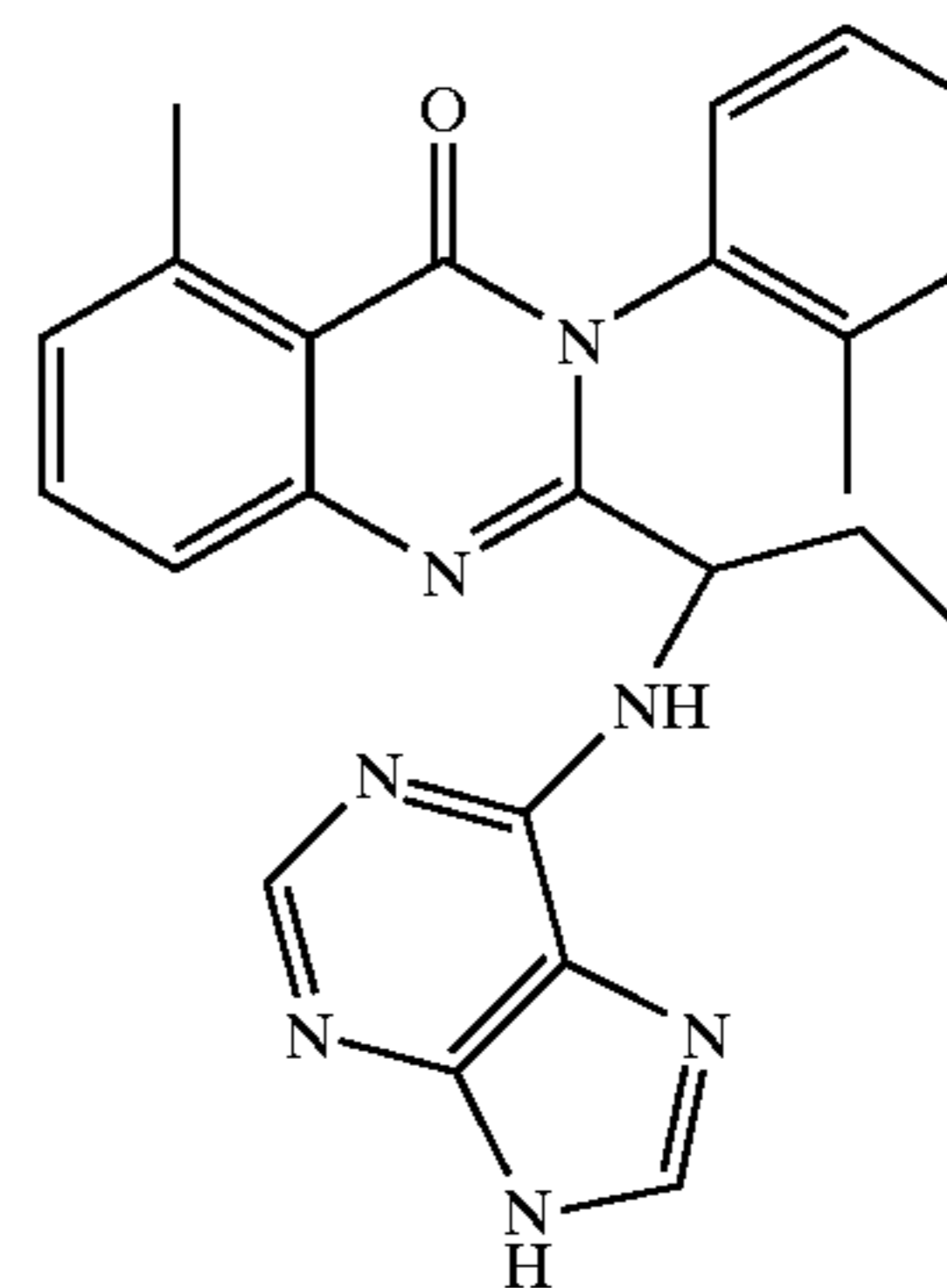
5-Methyl-2-(1-(9H-purin-6-ylamino)propyl)-3-o-tolyl-3H-quinazolin-4-one (D-081b)
