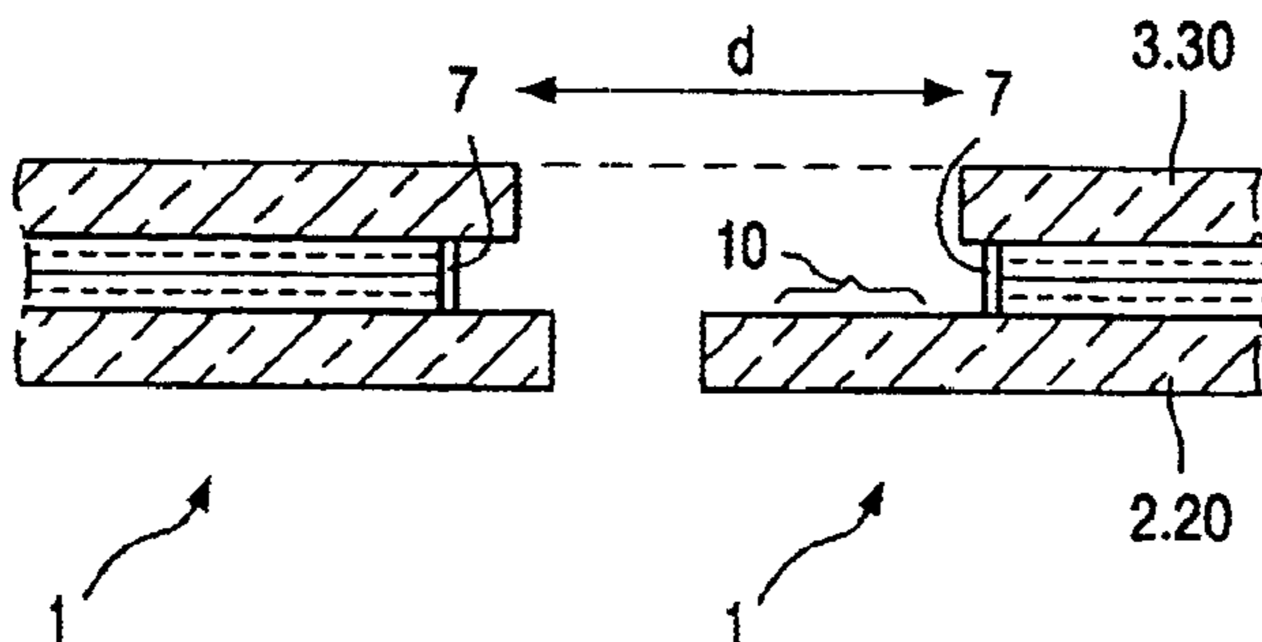
FIG. 3 PRIOR ART
