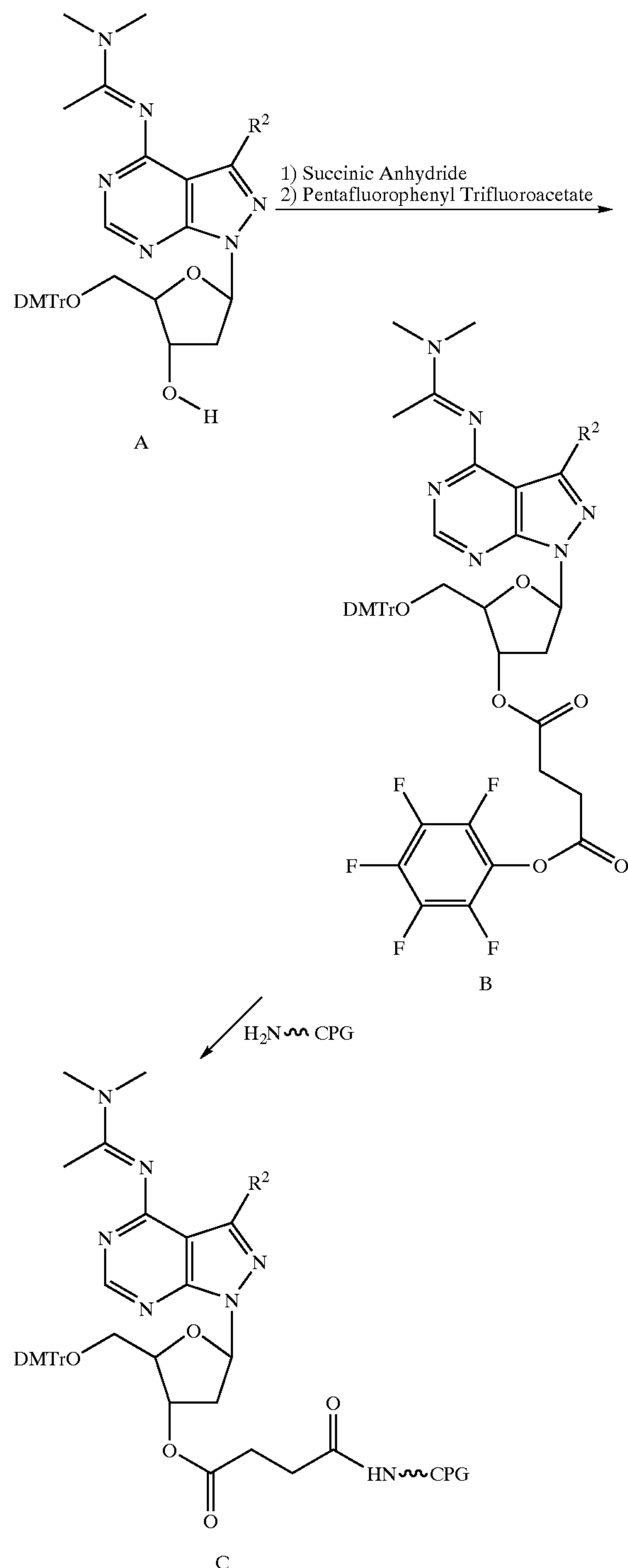
Reaction Scheme 10
