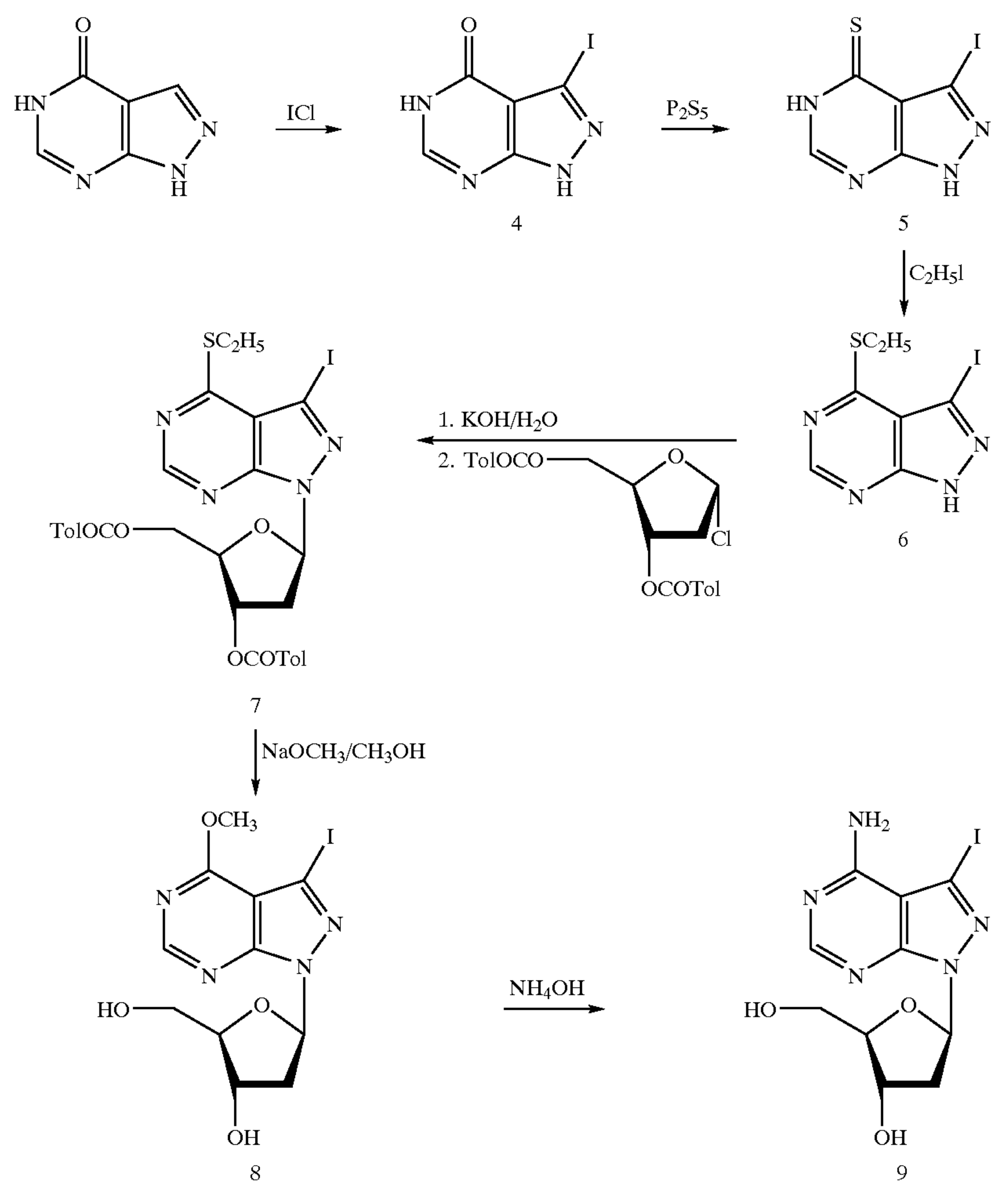
Reaction Scheme 2
