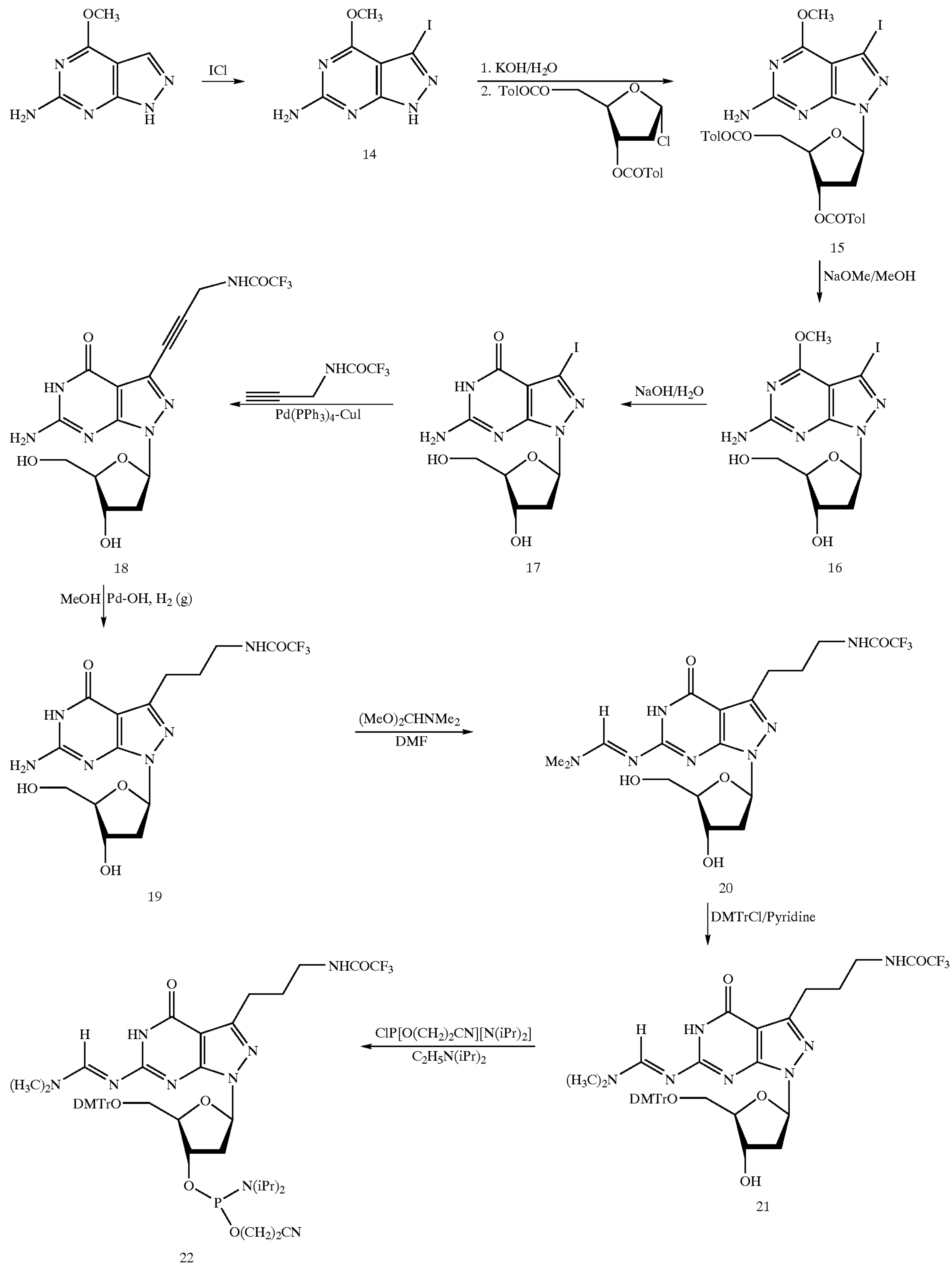
Reaction Scheme 4
