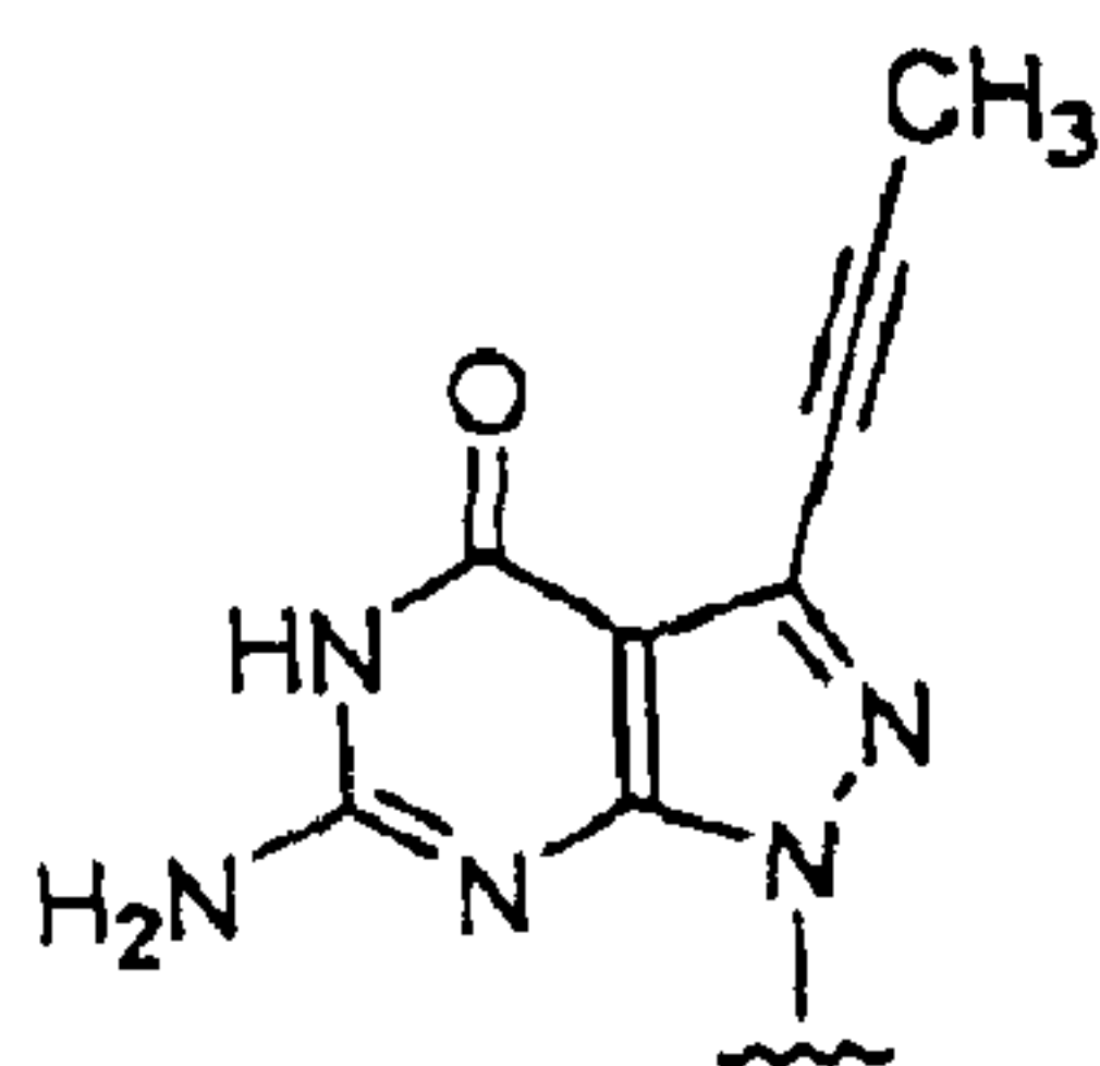
PPPG
