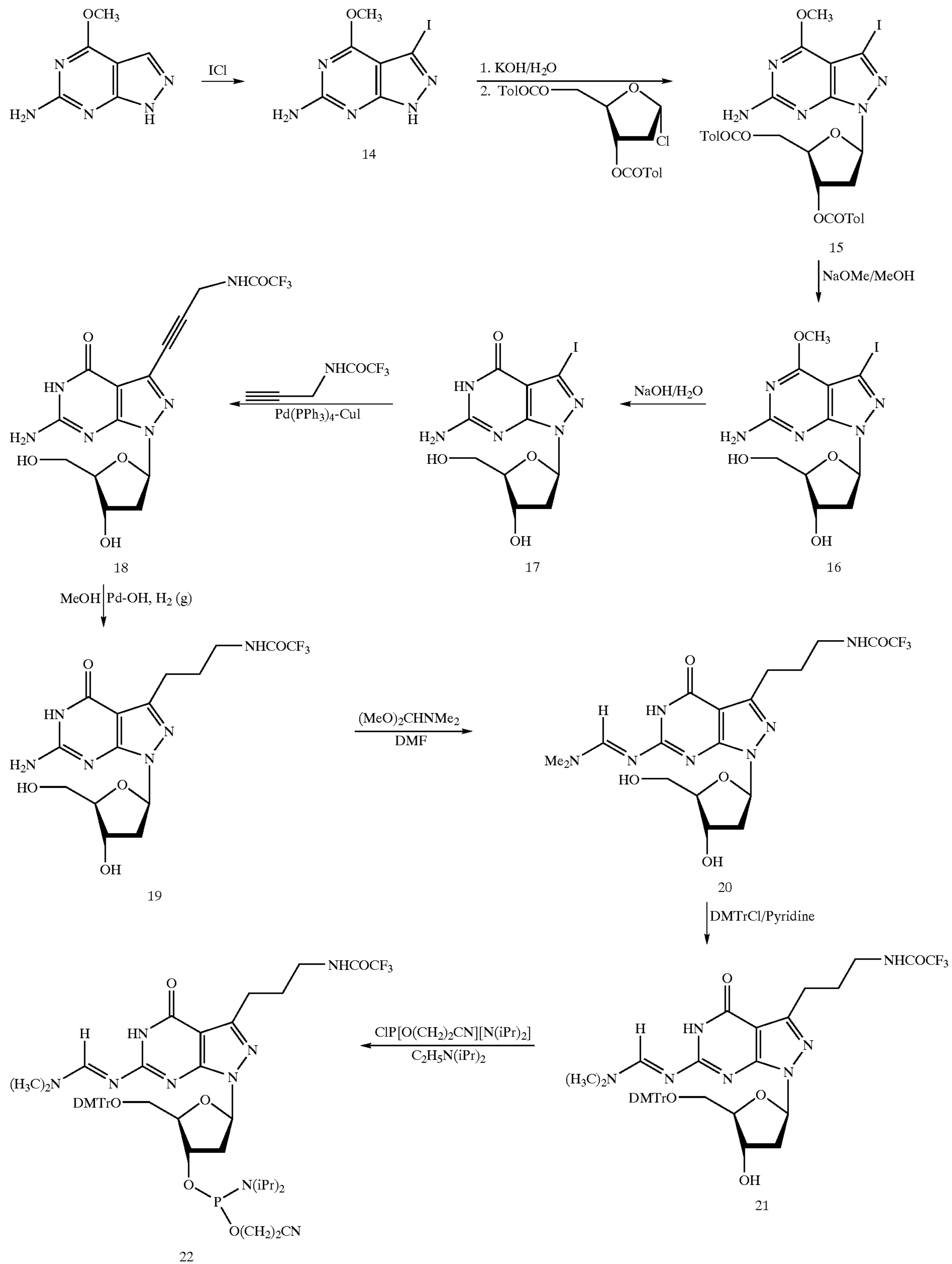
Reaction Scheme 4
