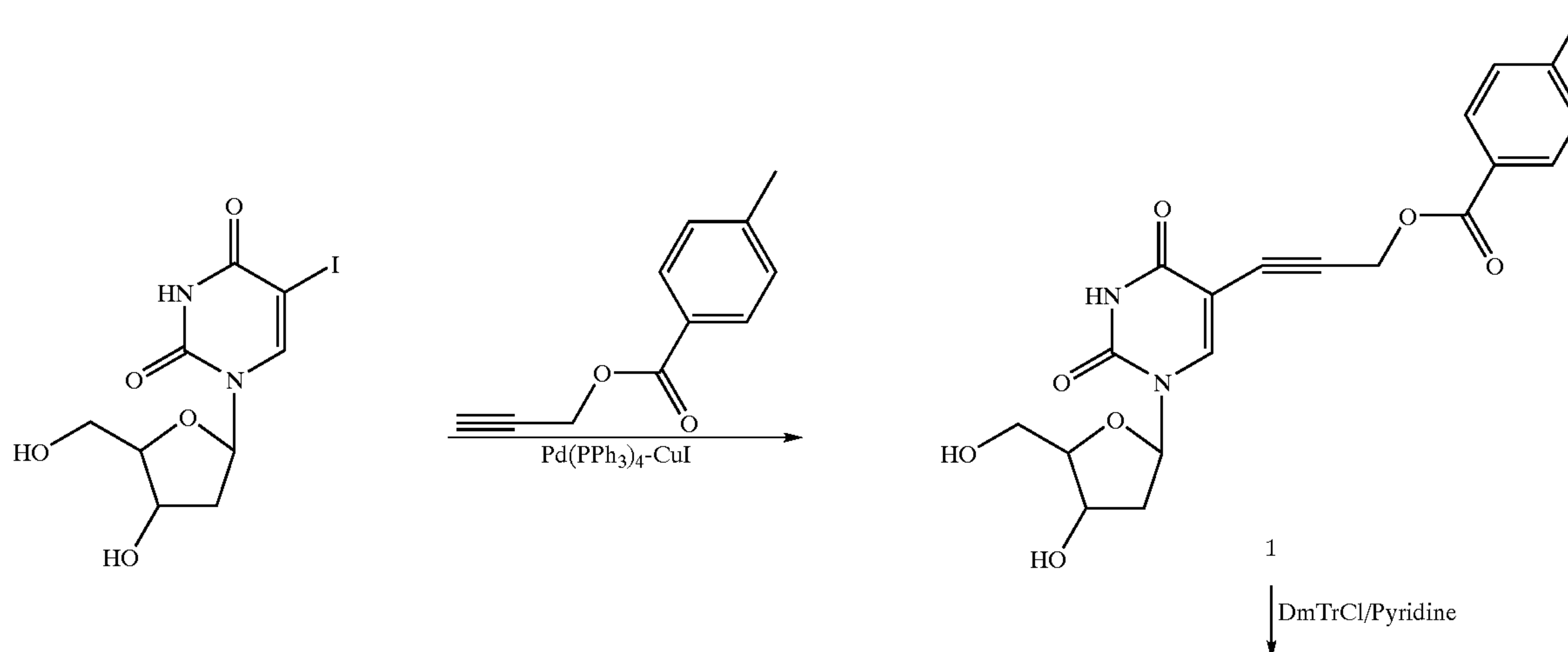
Reaction Scheme 1
