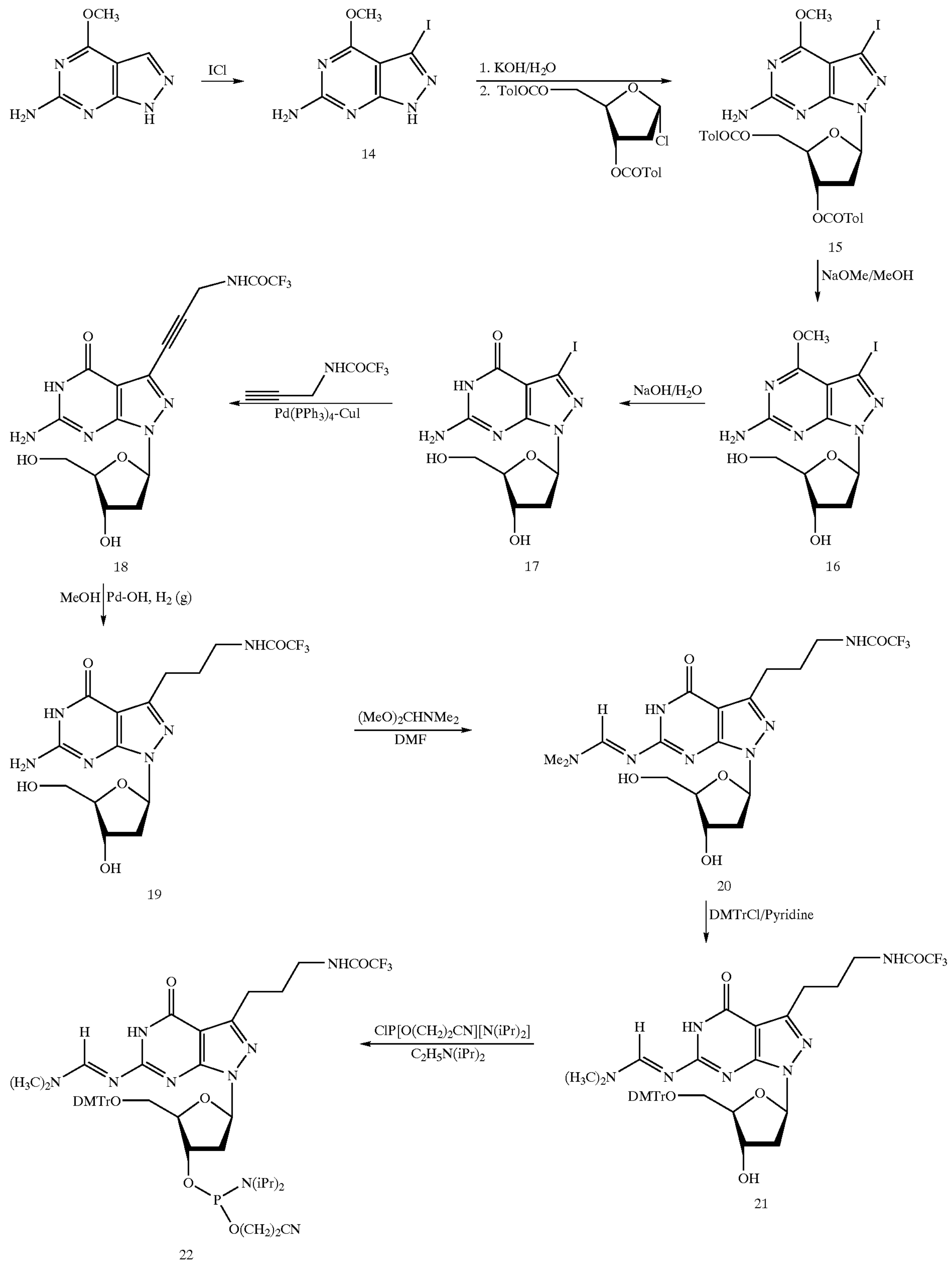
Reaction Scheme 4
