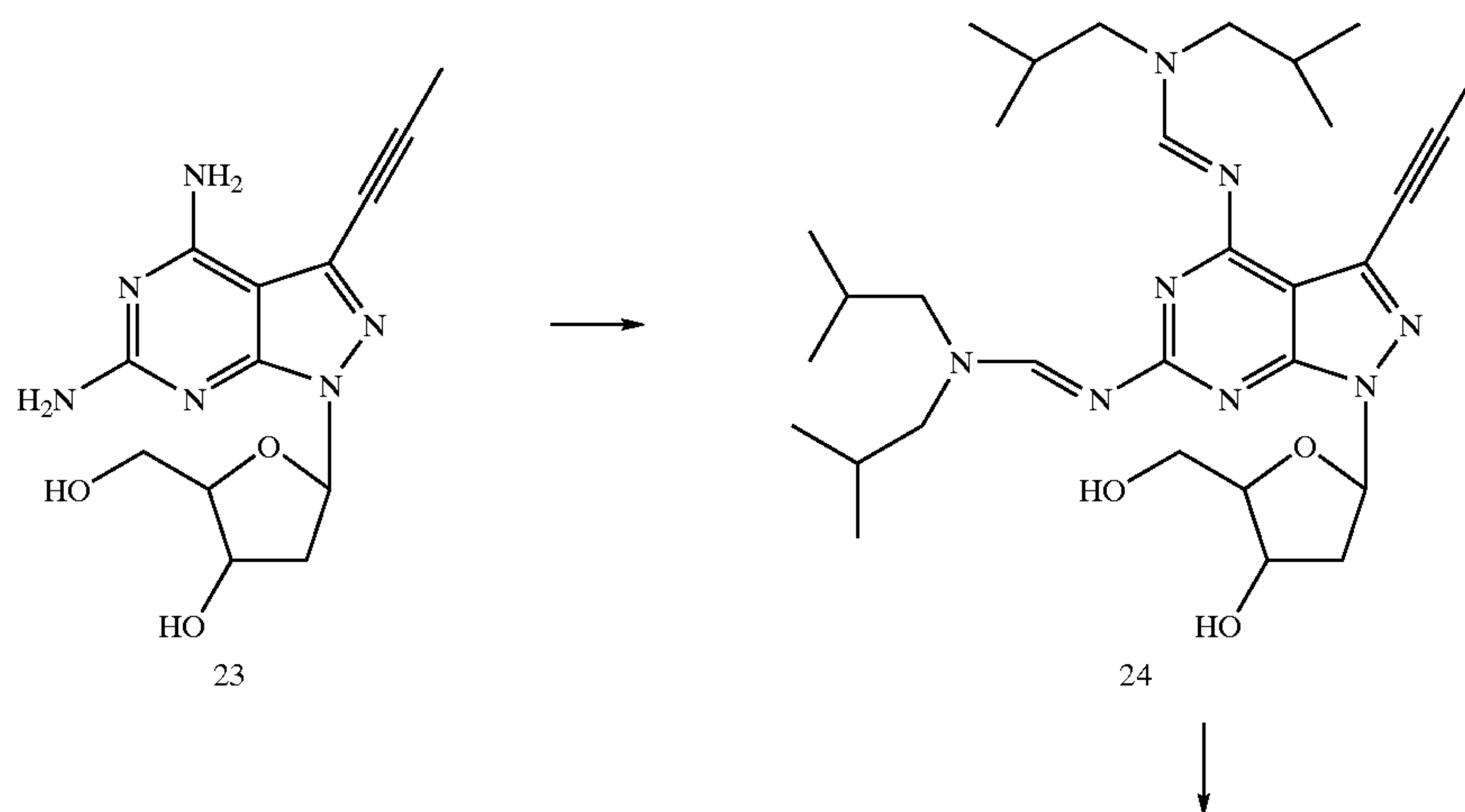
Reaction Scheme 5
