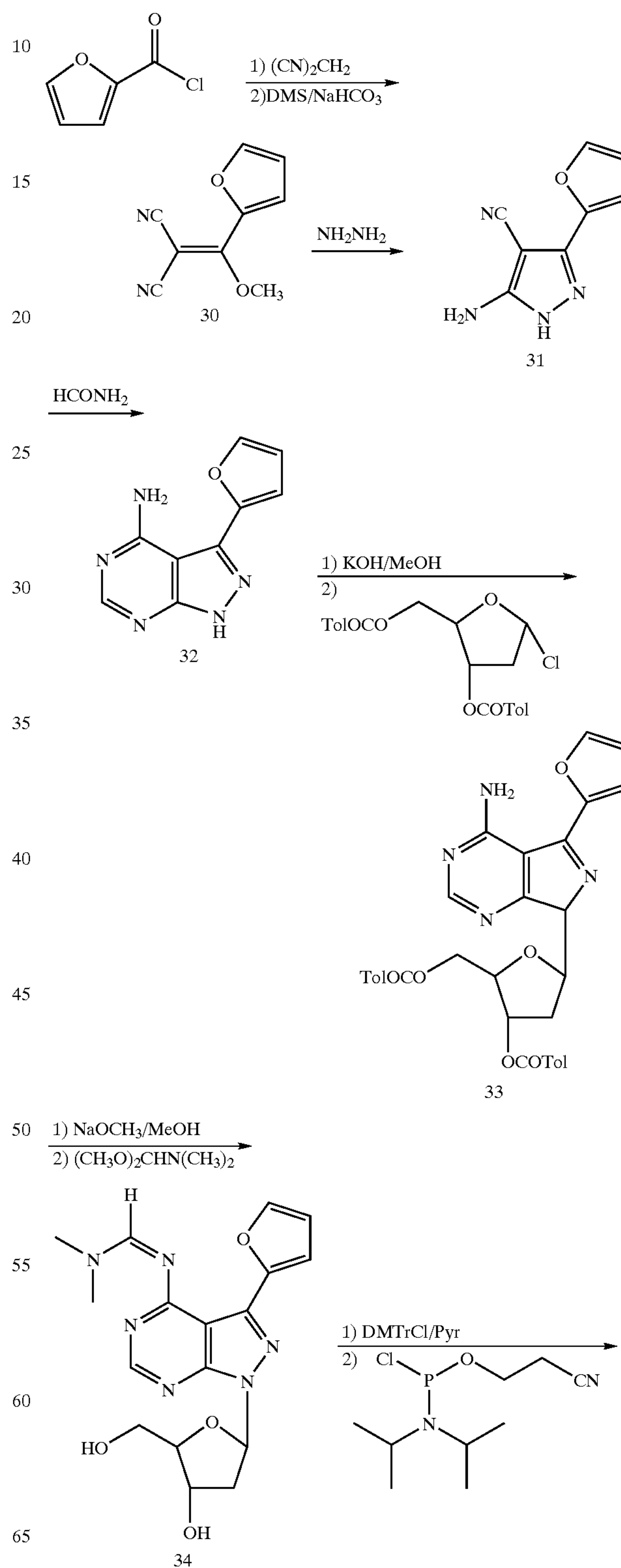
Reaction Scheme 8
