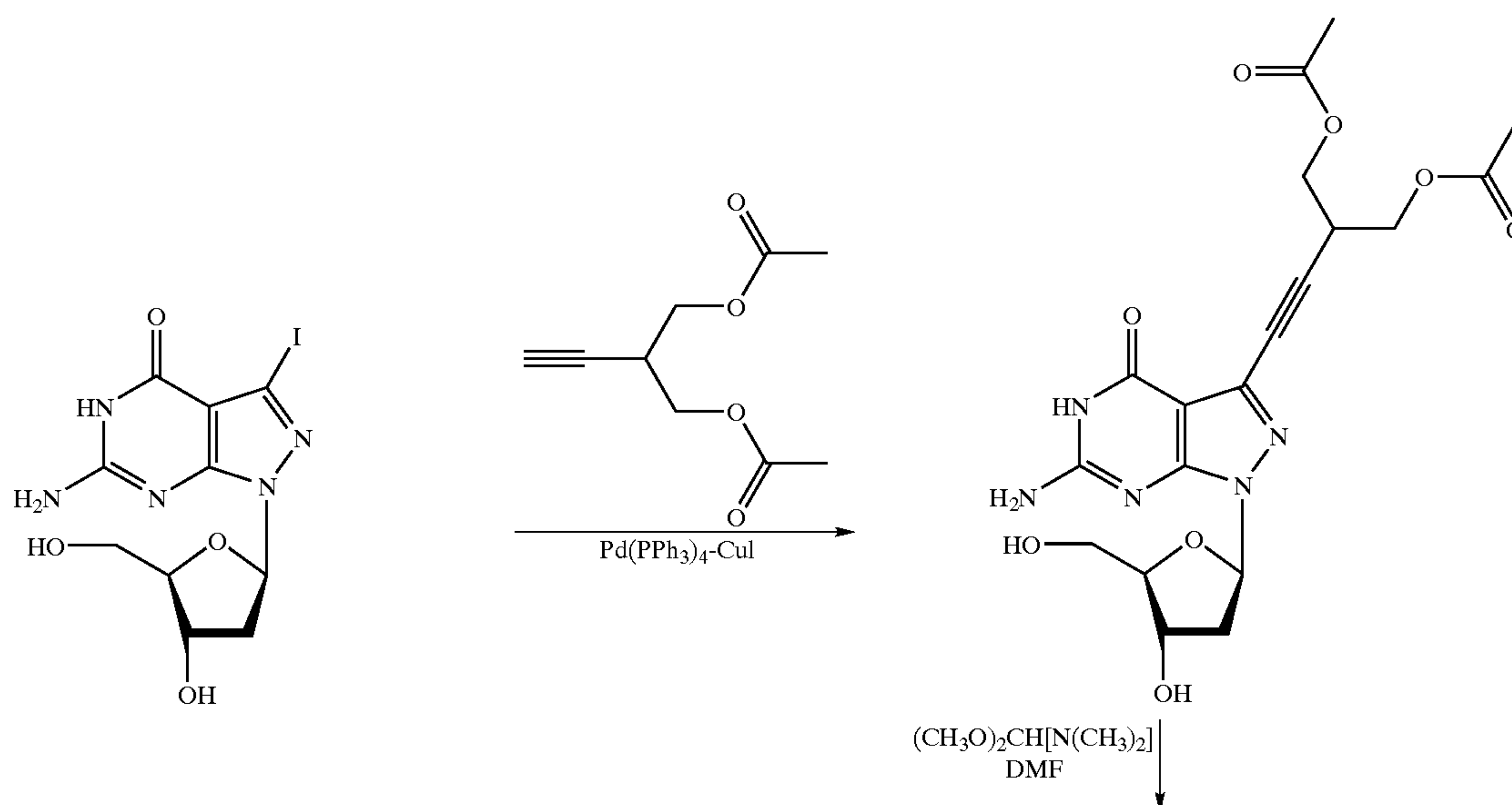
Reaction Scheme 6
