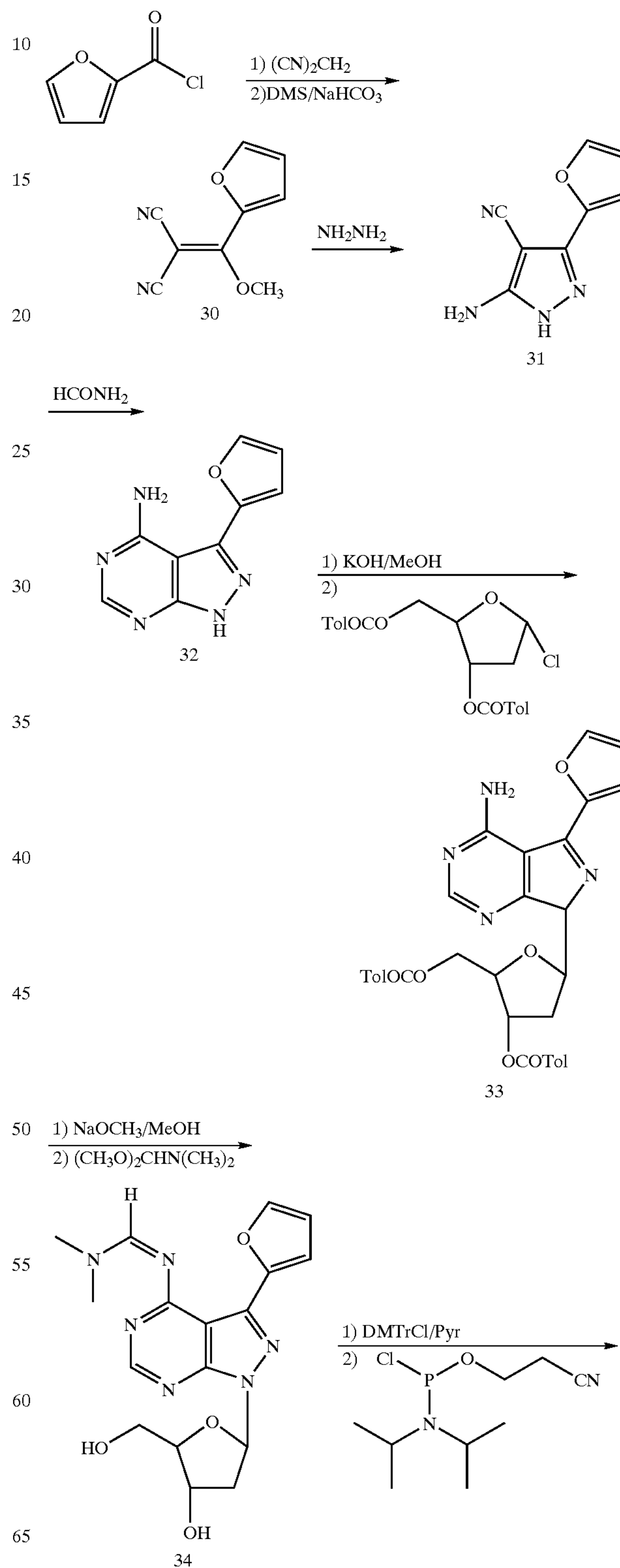
Reaction Scheme 8
