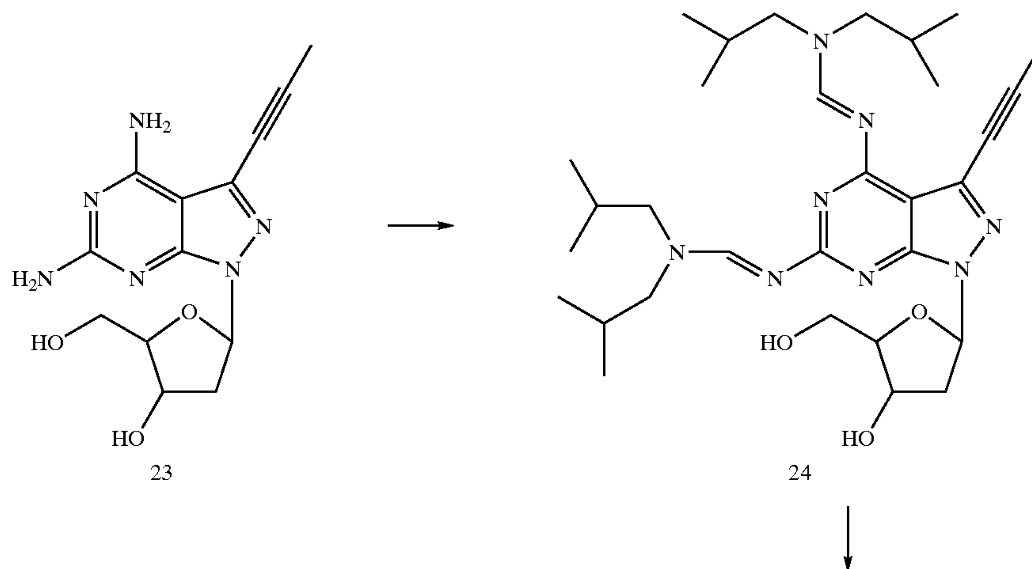
Reaction Scheme 5
