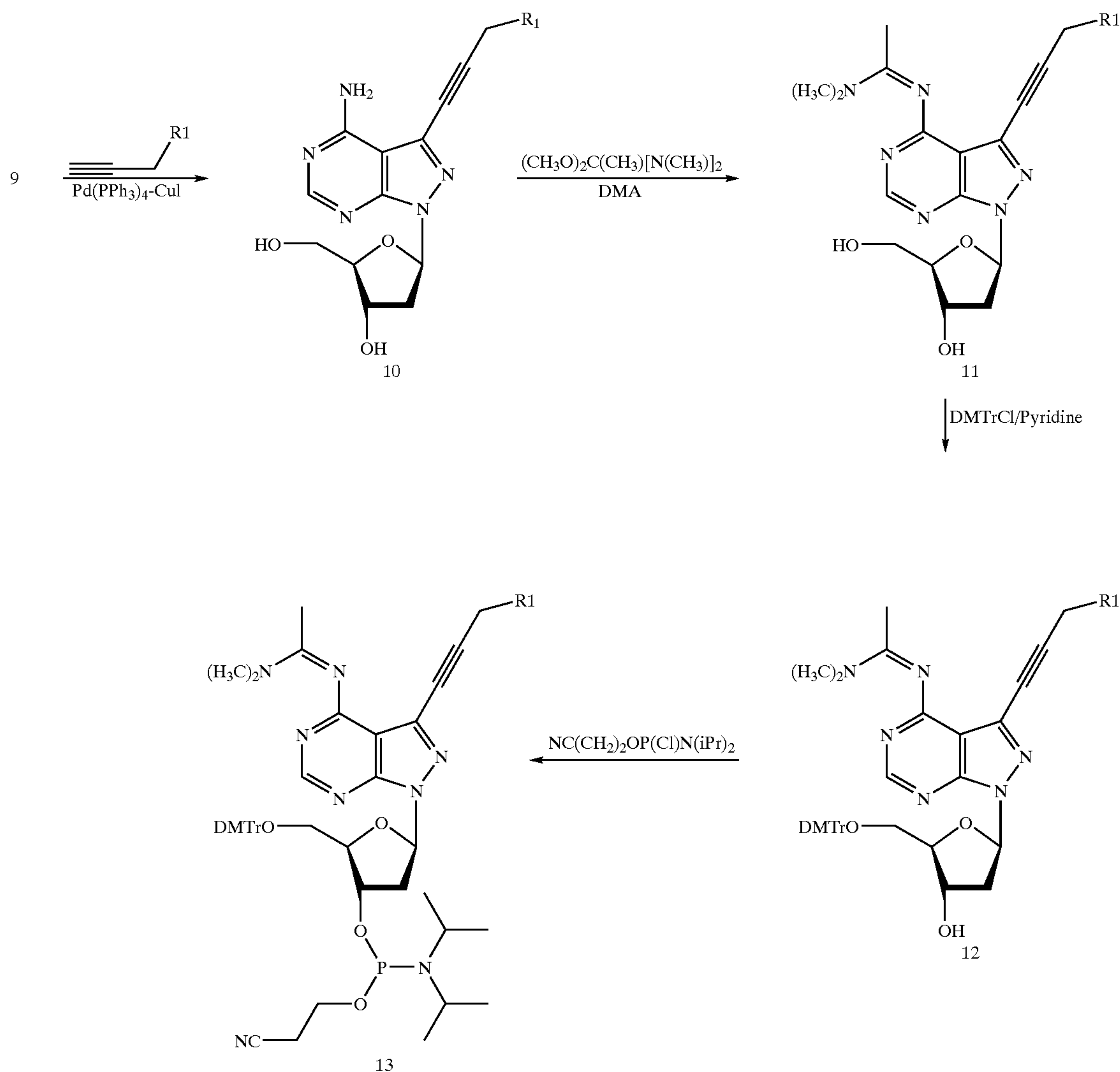
Reaction Scheme 3
