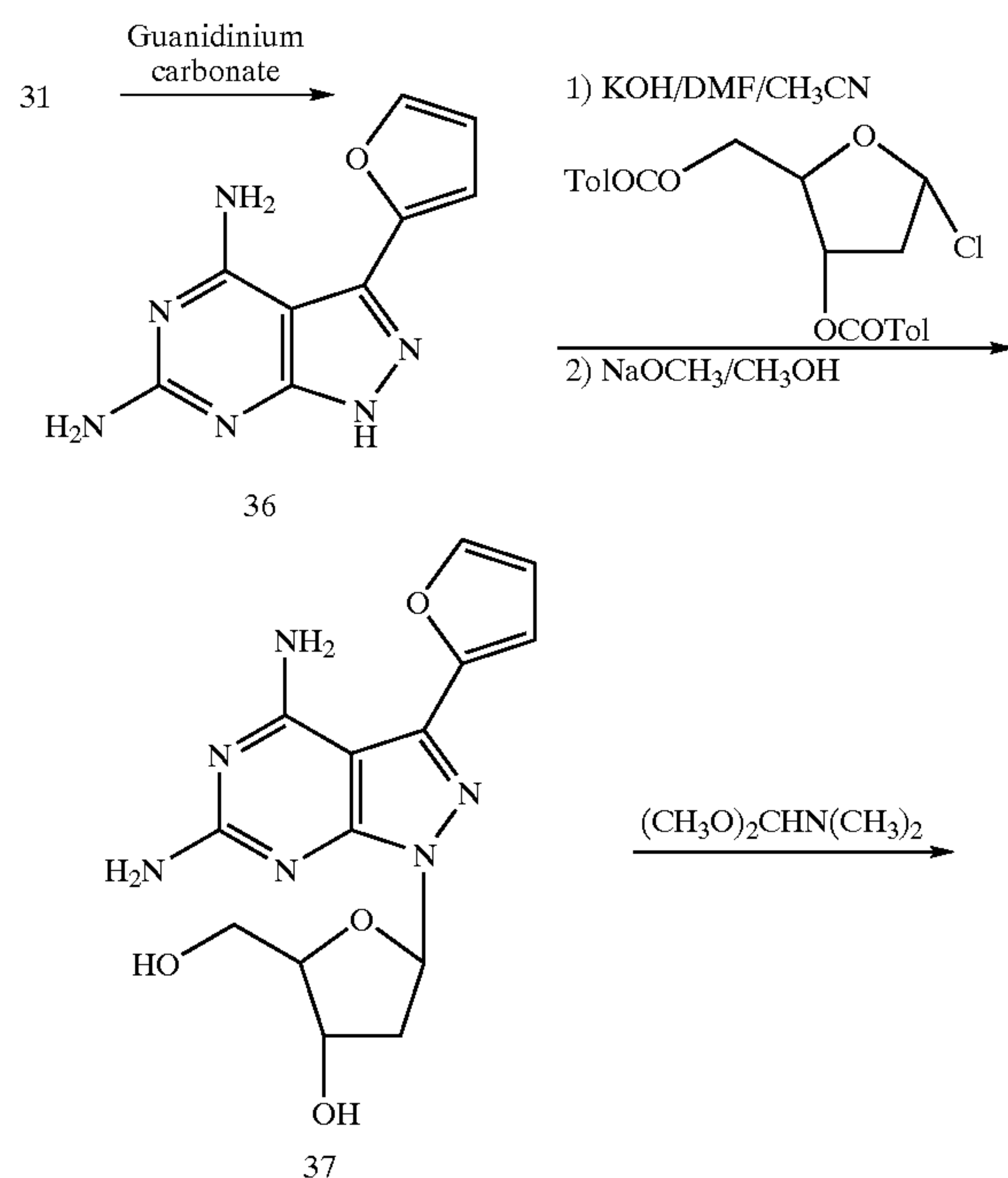
Reaction Scheme 9
