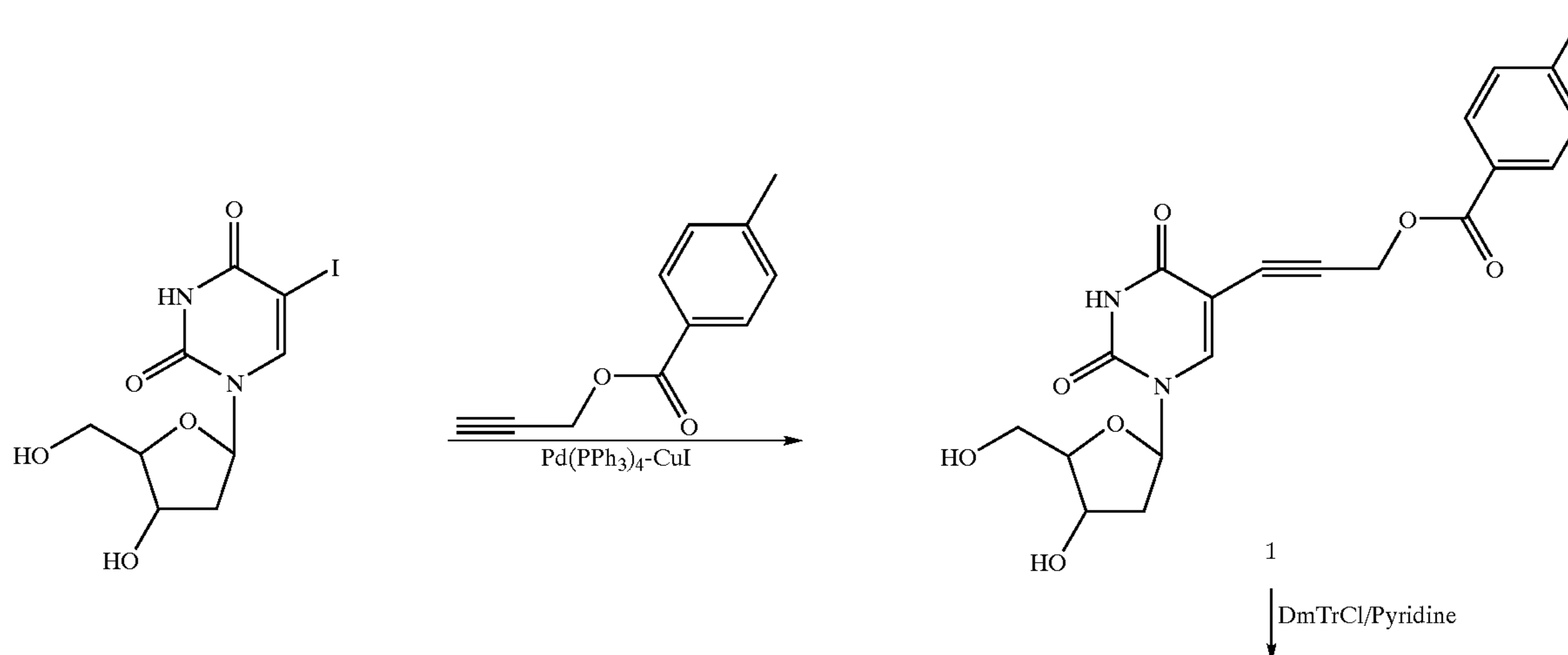
Reaction Scheme 1
