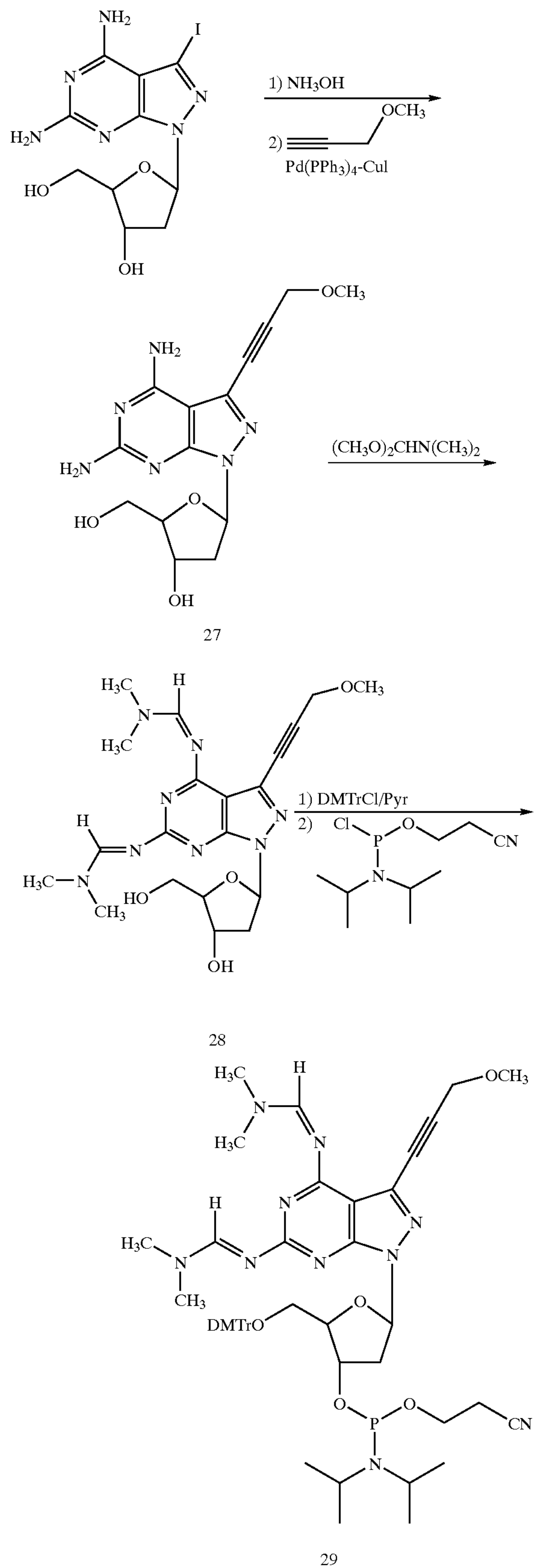
Reaction Scheme 7
