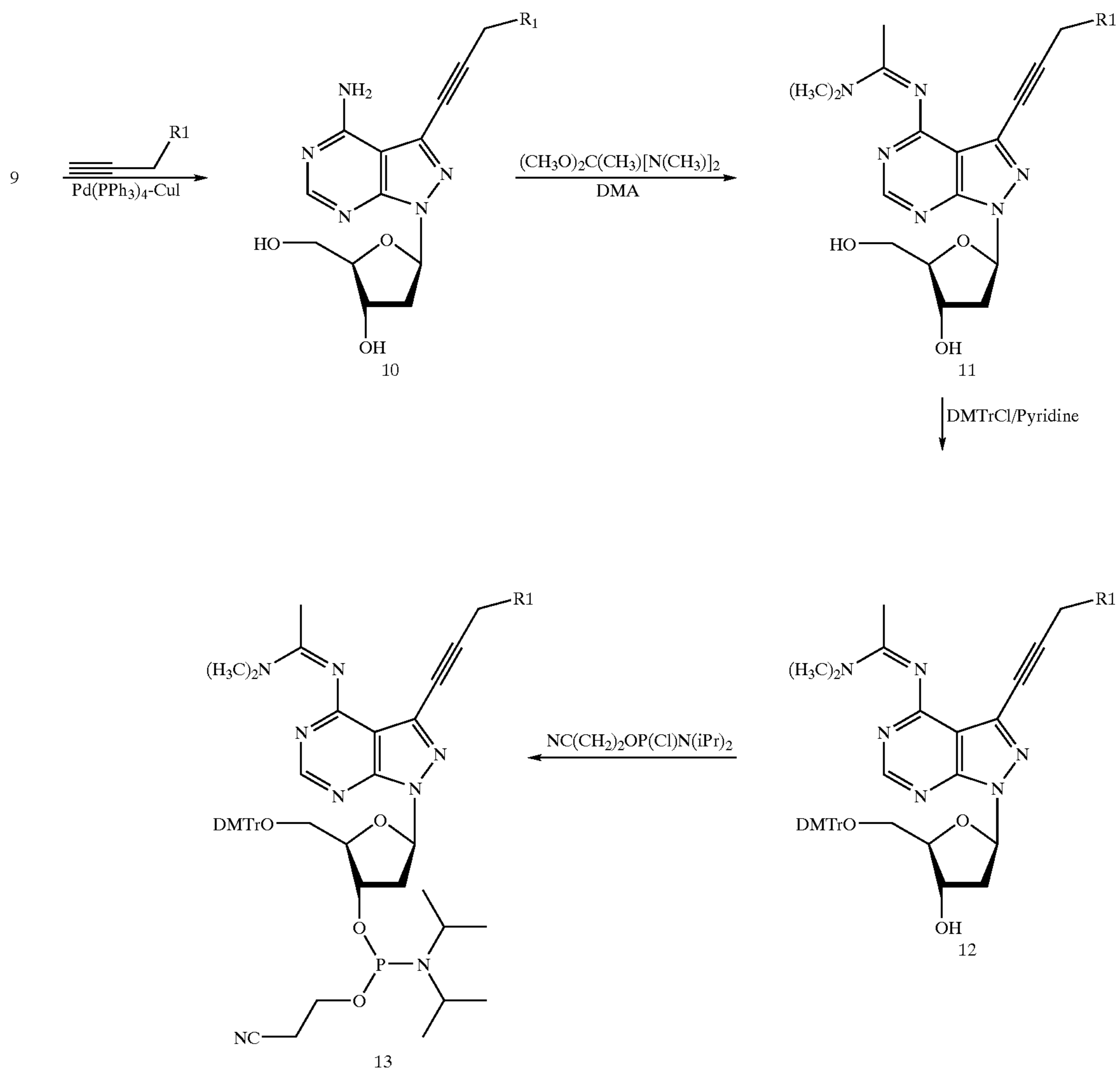
Reaction Scheme 3
