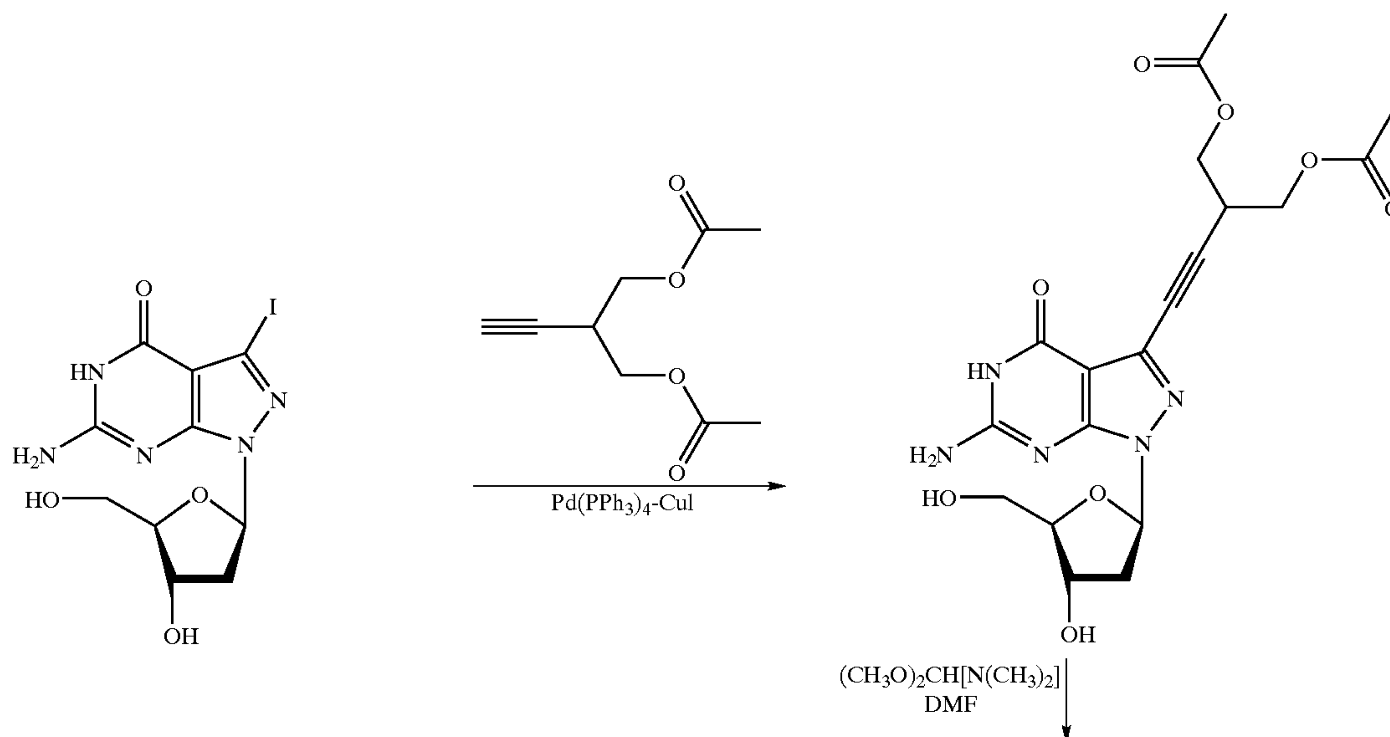
Reaction Scheme 6
