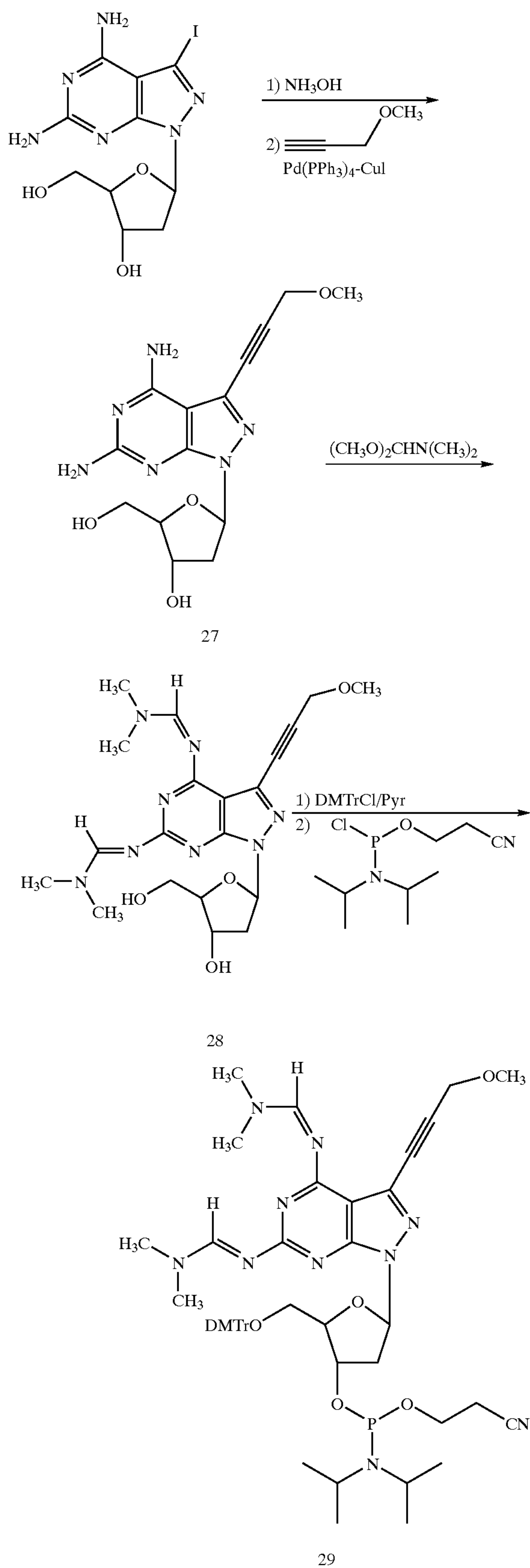
Reaction Scheme 7
