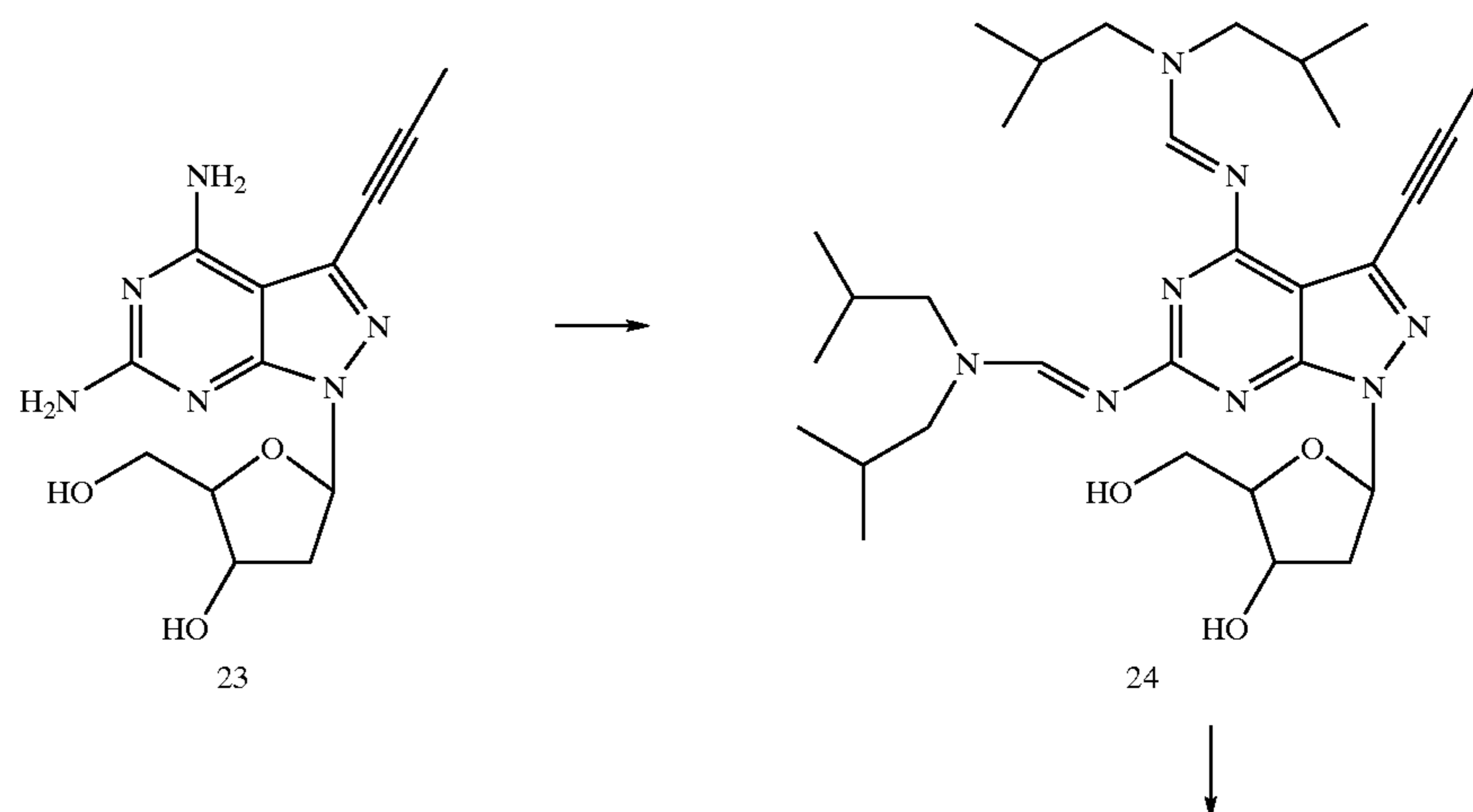
Reaction Scheme 5
