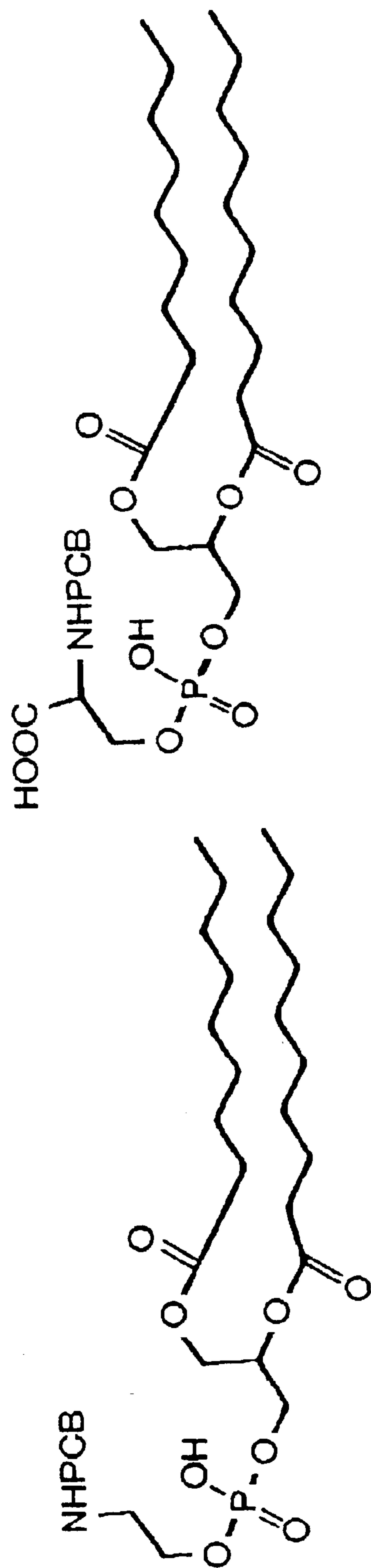
PCB-Phosphatytense (PCB-PS)
