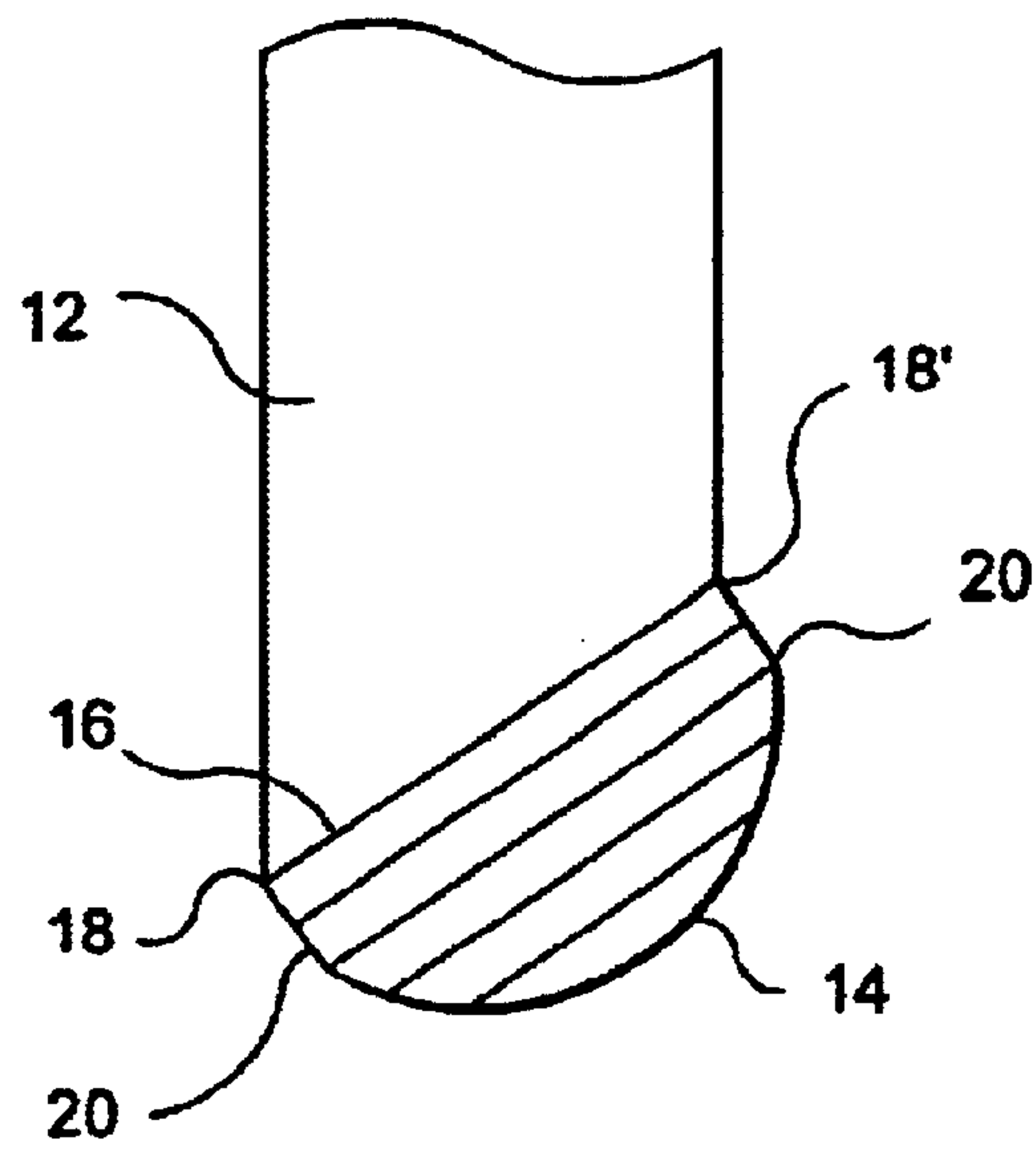
FIG. 2 PRIOR ART
