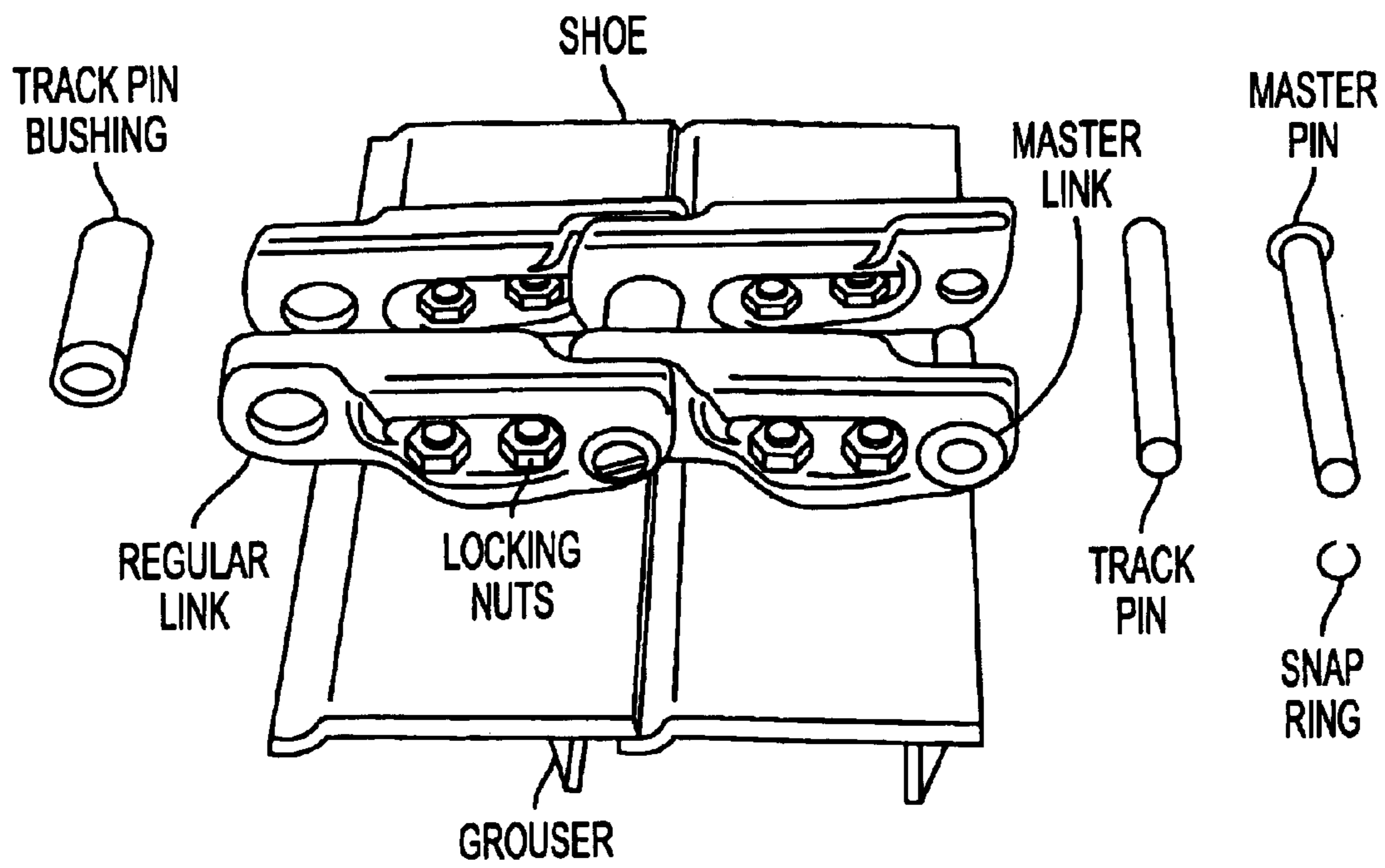
FIG. 1 (PRIOR ART)
