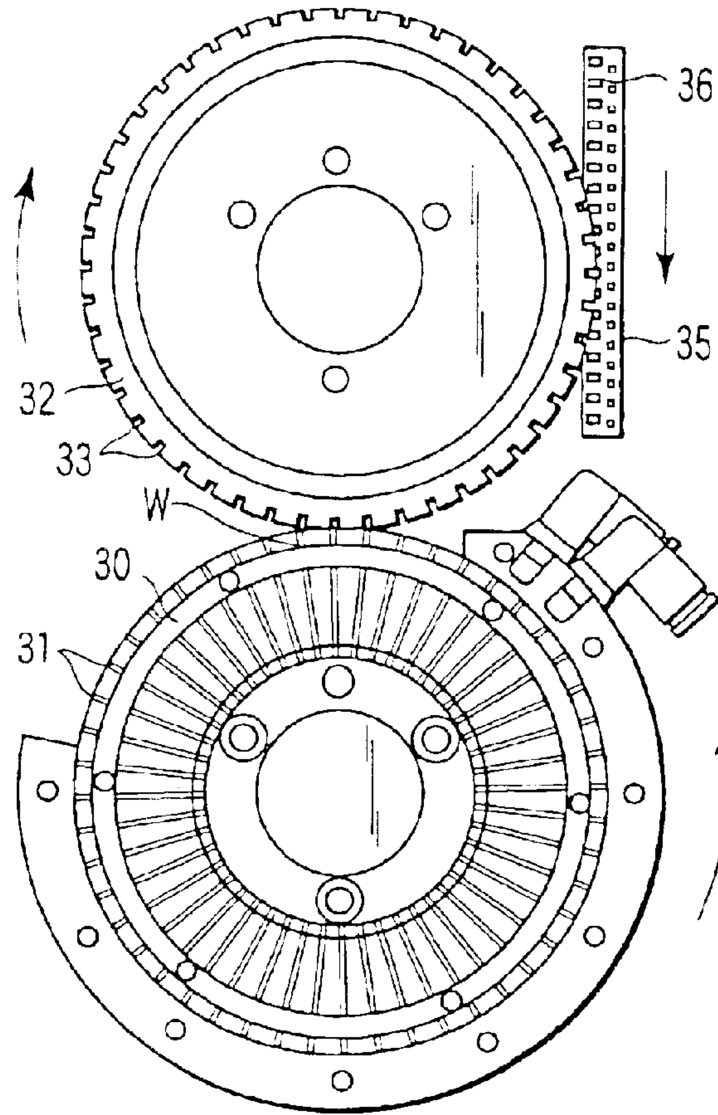
FIG. 6 PRIOR ART
