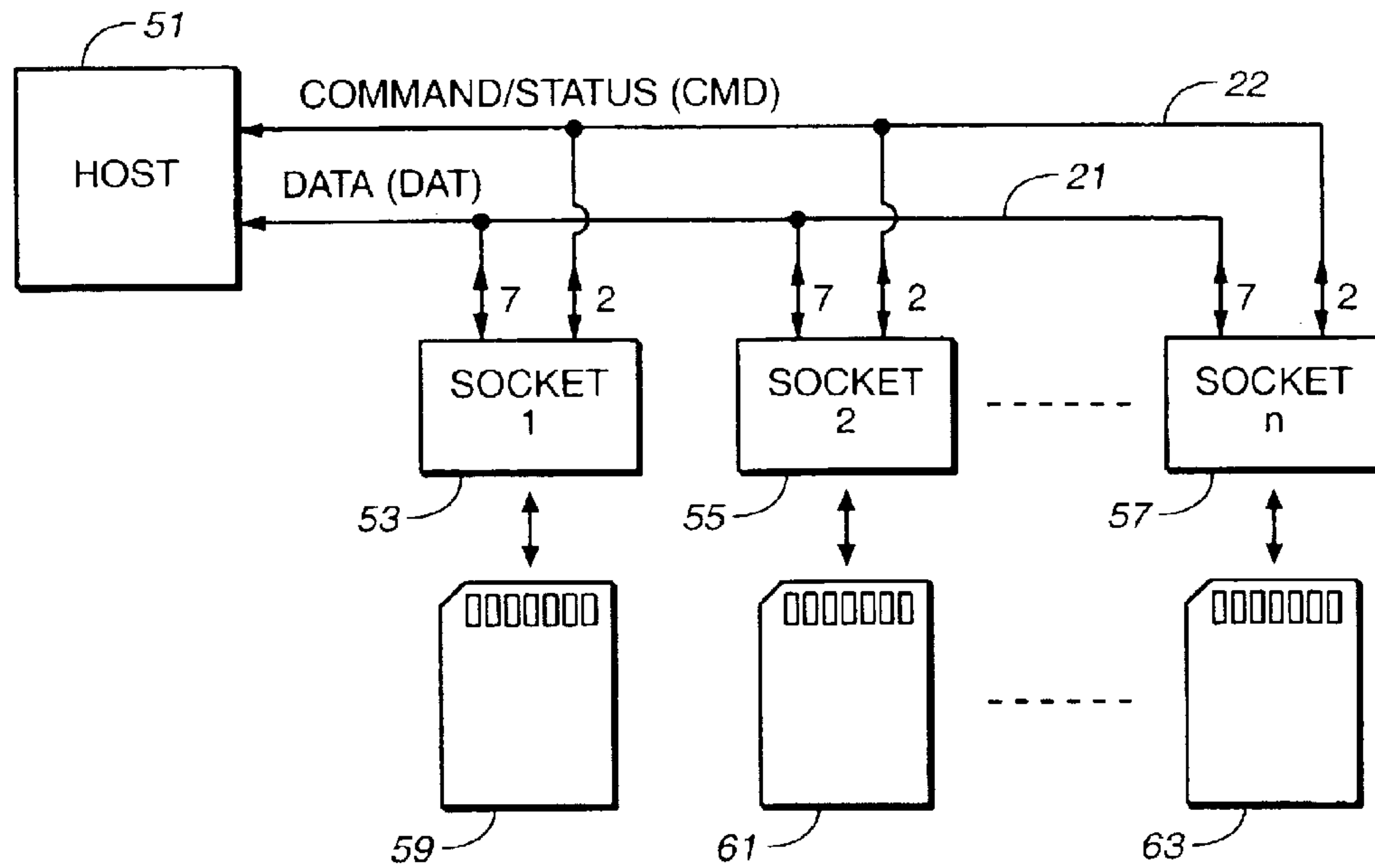
FIG. 3 (PRIOR ART)
