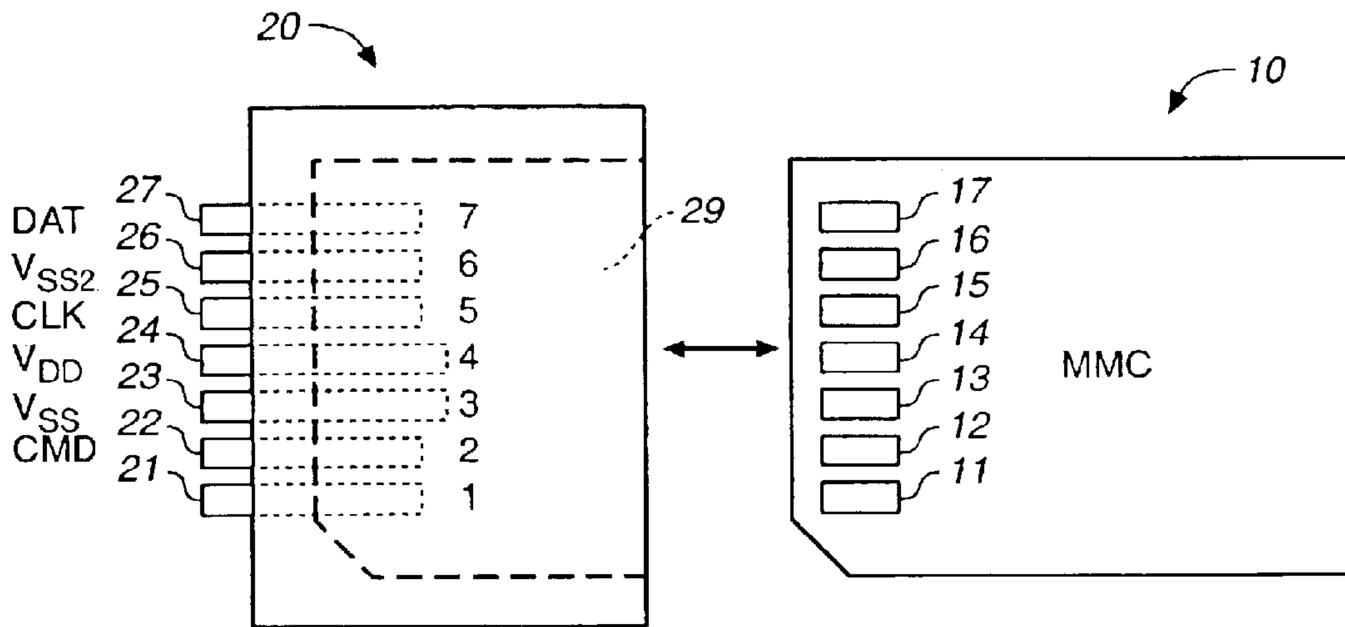
FIG. 1 (PRIOR ART)
