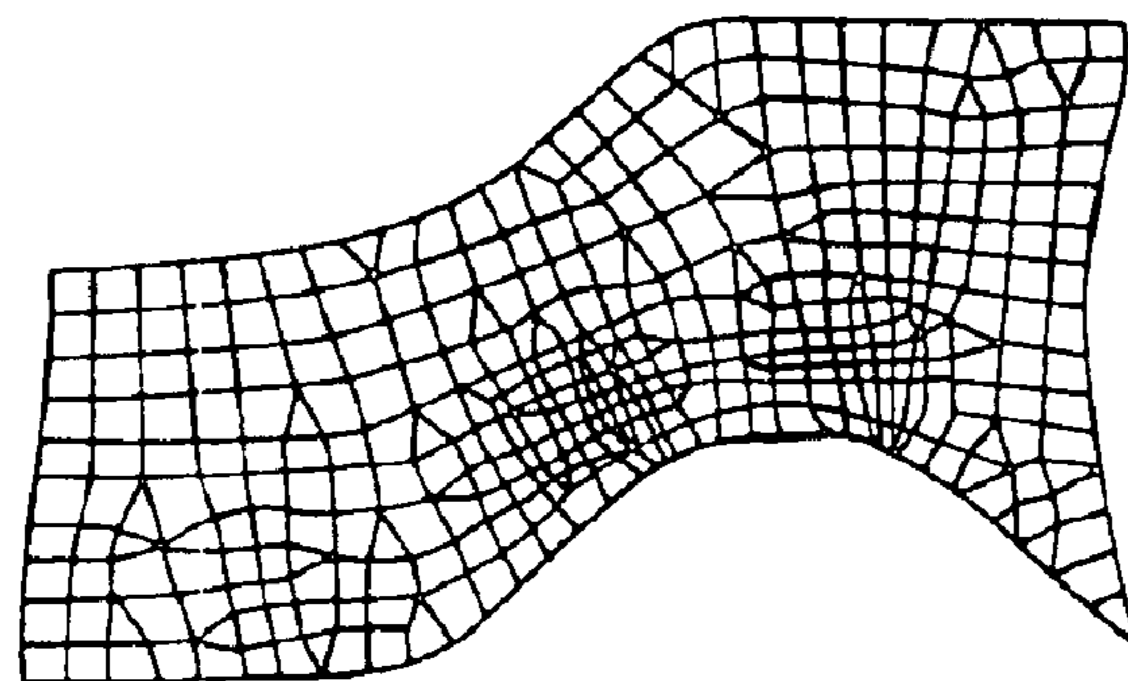
GENERATED MESH FIG. 12d
