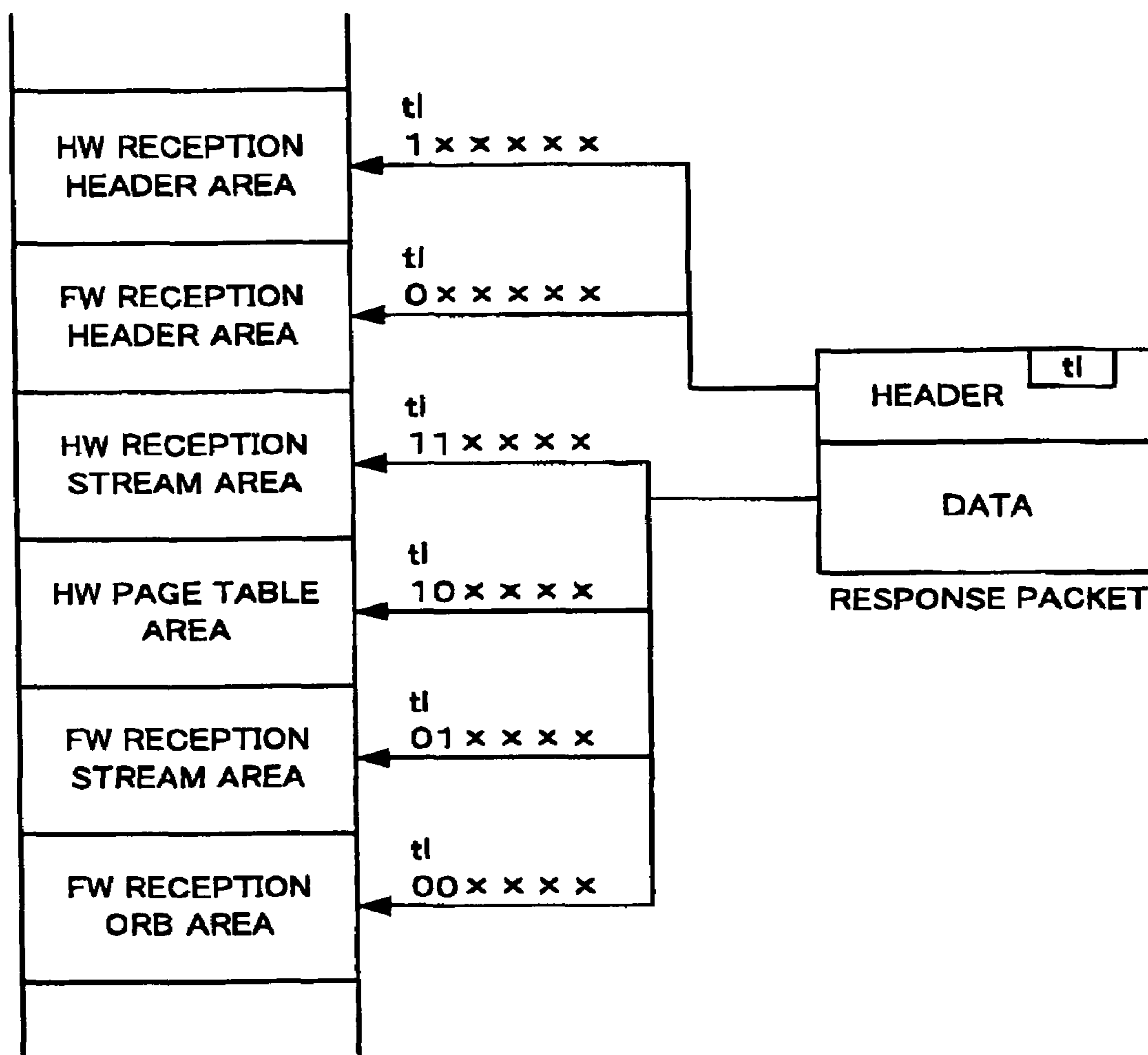
RAM (PACKET STORAGE MEANS)
