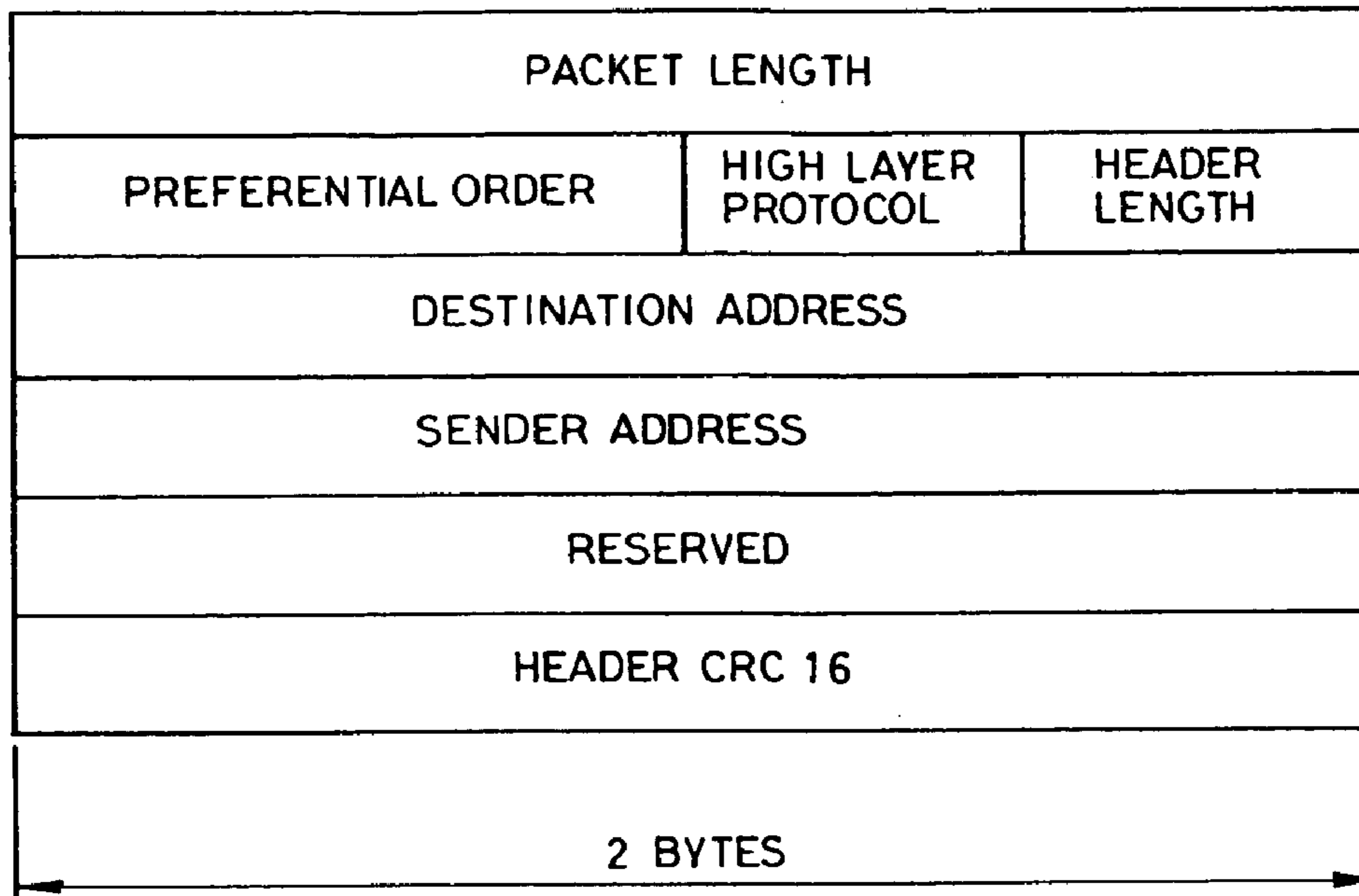
HEADER STRUCTURE IN CASE OF ATM
