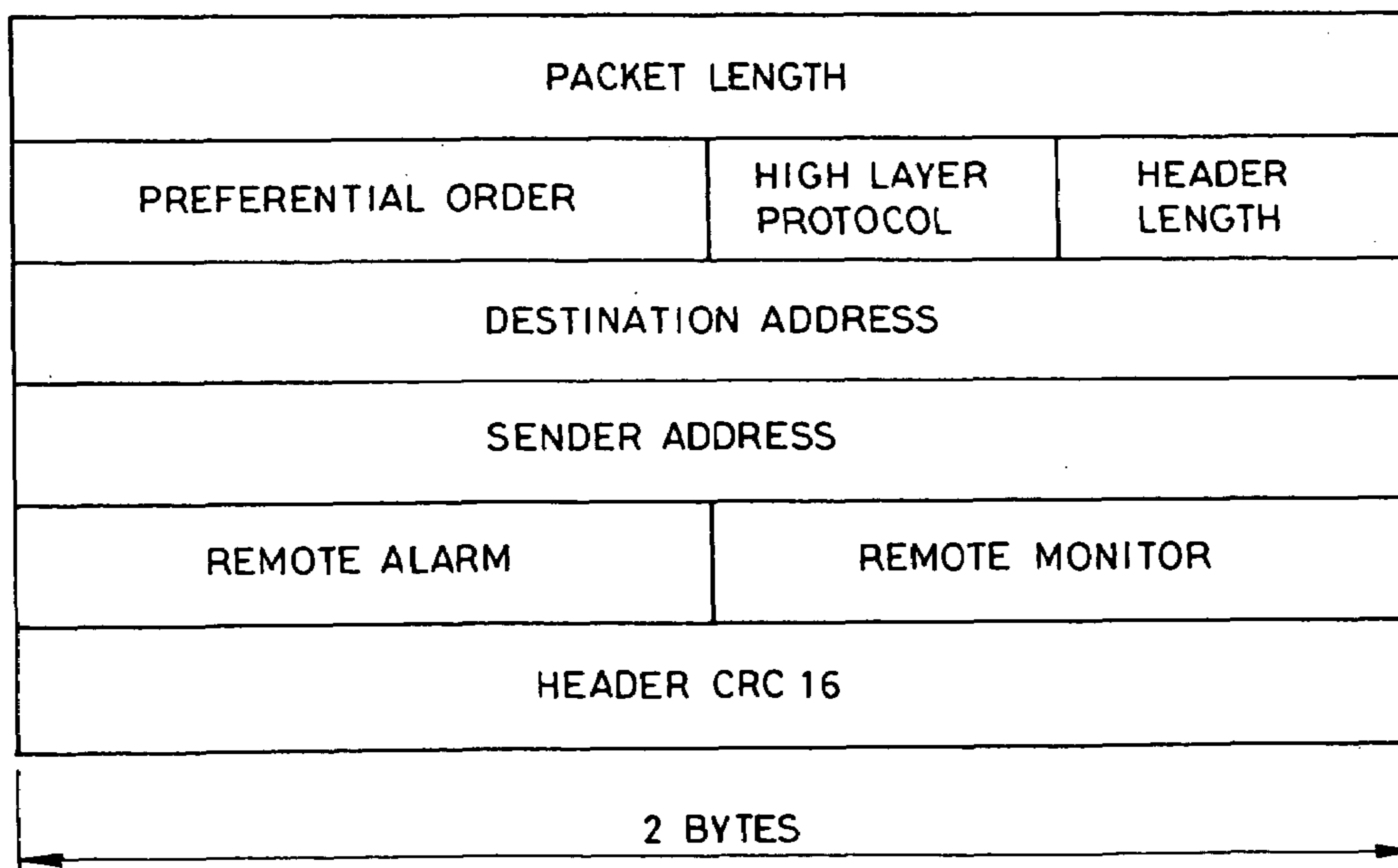
HEADER STRUCTURE IN CASE OF STM
