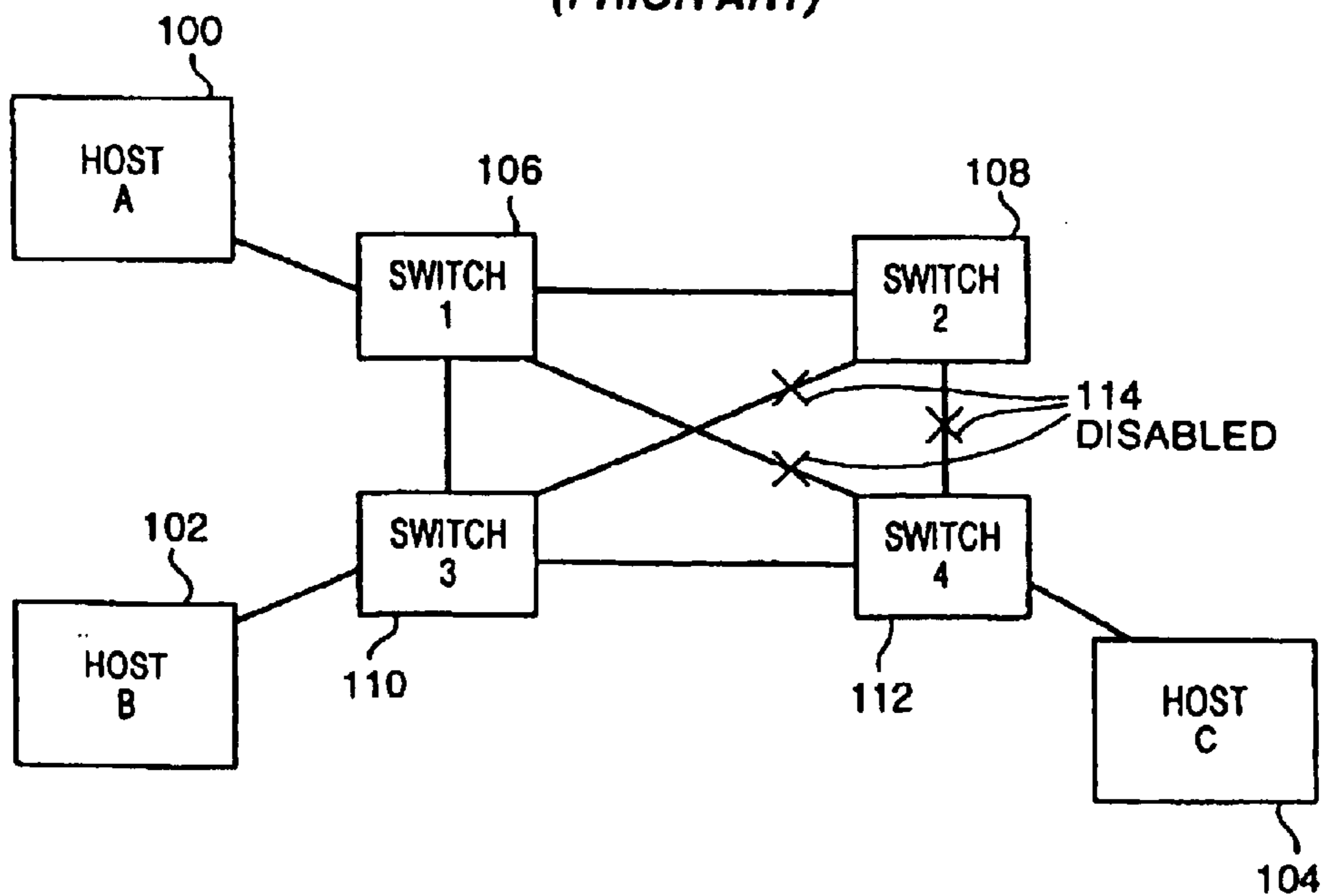
FIG. 2 (PRIOR ART)
