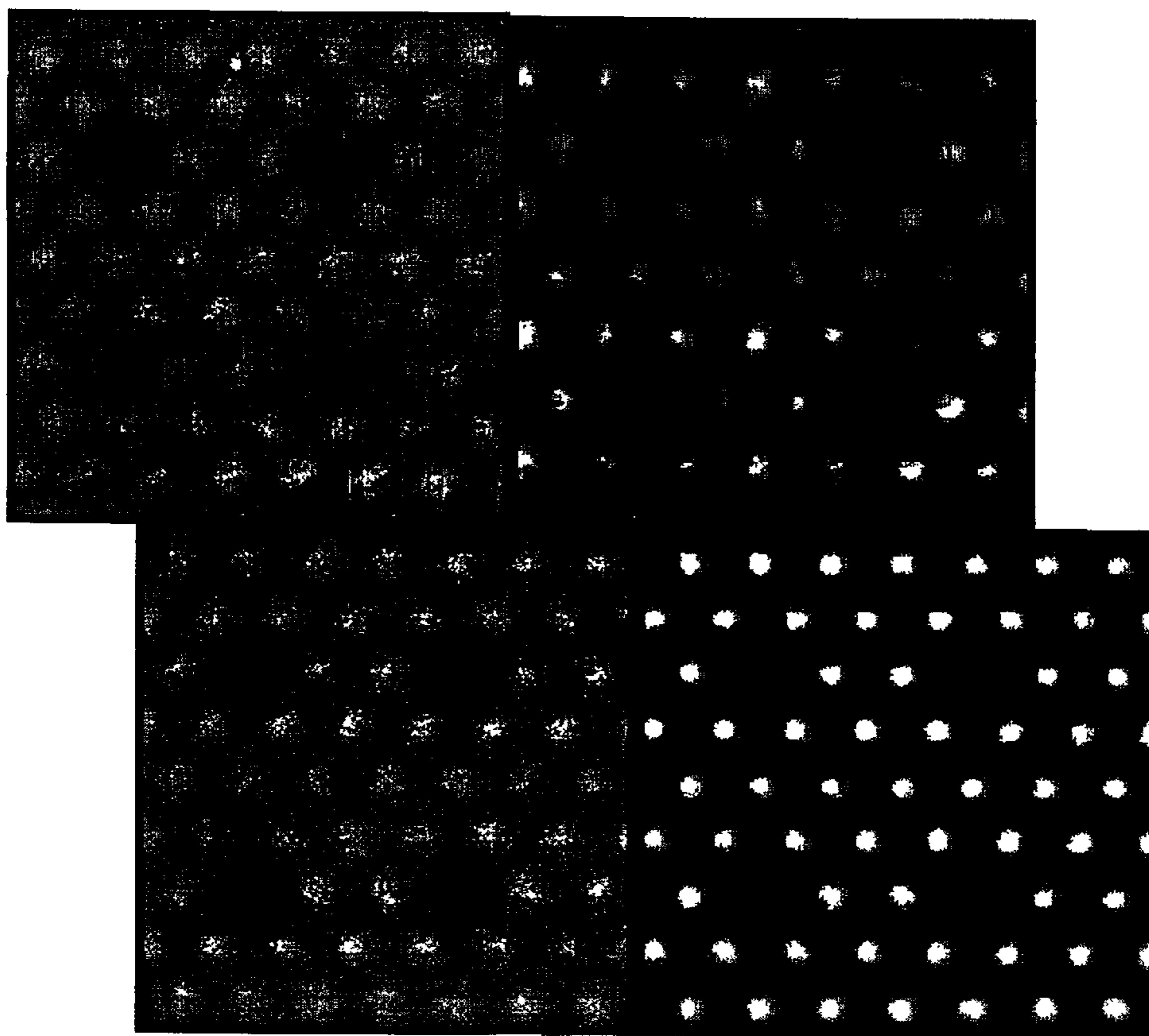
Figure 5 (top left ) Laser confocal fluorescent microscopy image of nano-particle array. 2 The bits have core diameter 650 \pm 20 nm and shell thickness 200 \pm 5 nm . \lambda_{\text{Fluorescence}} \sim 500 nm, \lambda_{\text{two-photon}} = 844 nm. Resolution is approximately 256x256 samples. A data pattern has been photo-bleached into material (top right) After filtering and deconvolution approximate Gaussian point spread function. (bottom right) simulation of equivalent data with a sine squared basis bit (bottom left) with simulated point-spread function of diameter, 750nm and signal to noise ratio of 10.
