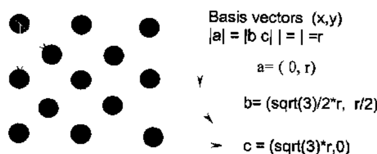
Basis vectors and the Lattice Translations
