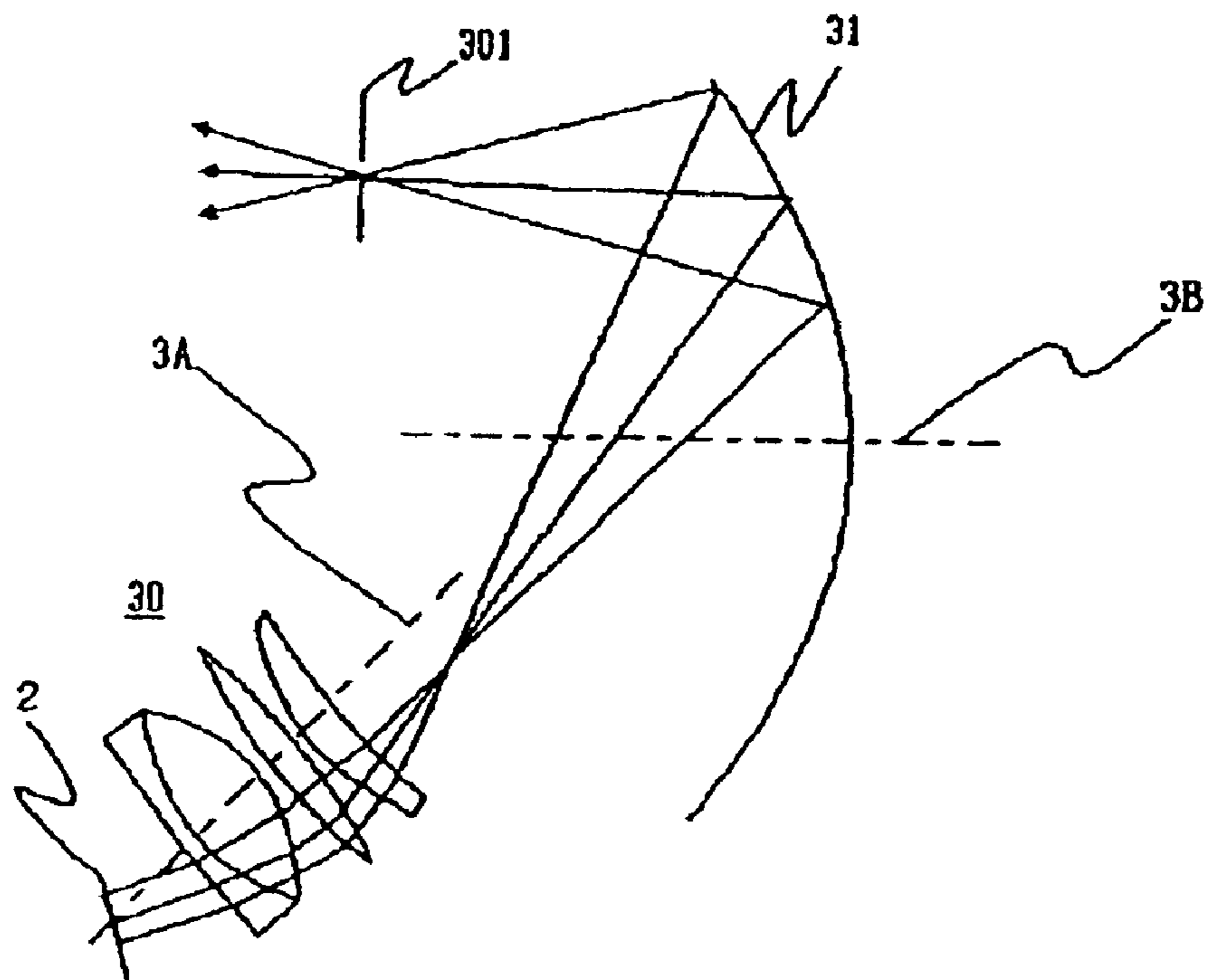
FIG. 41 (PRIOR ART)
