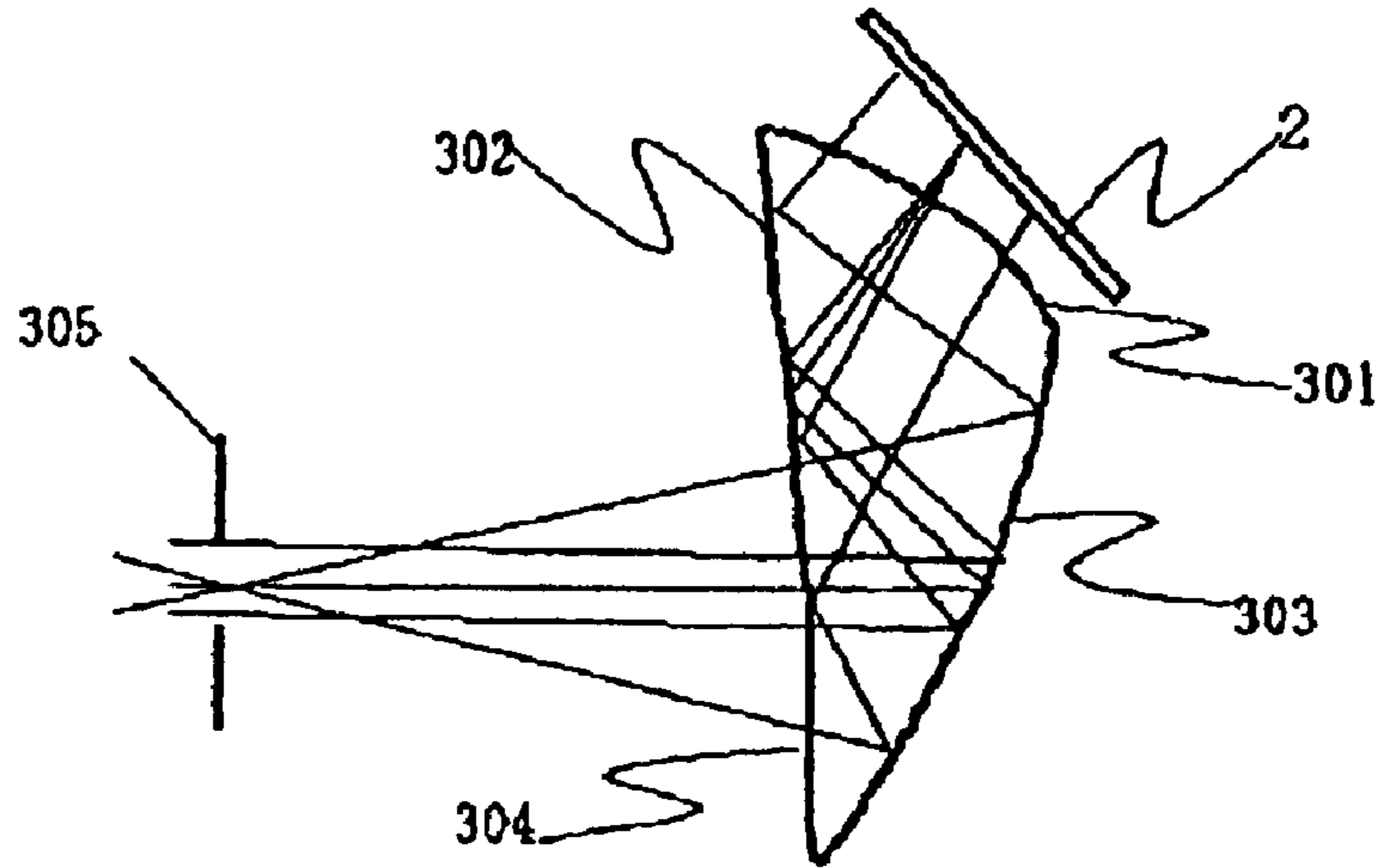
FIG. 45 (PRIOR ART)
