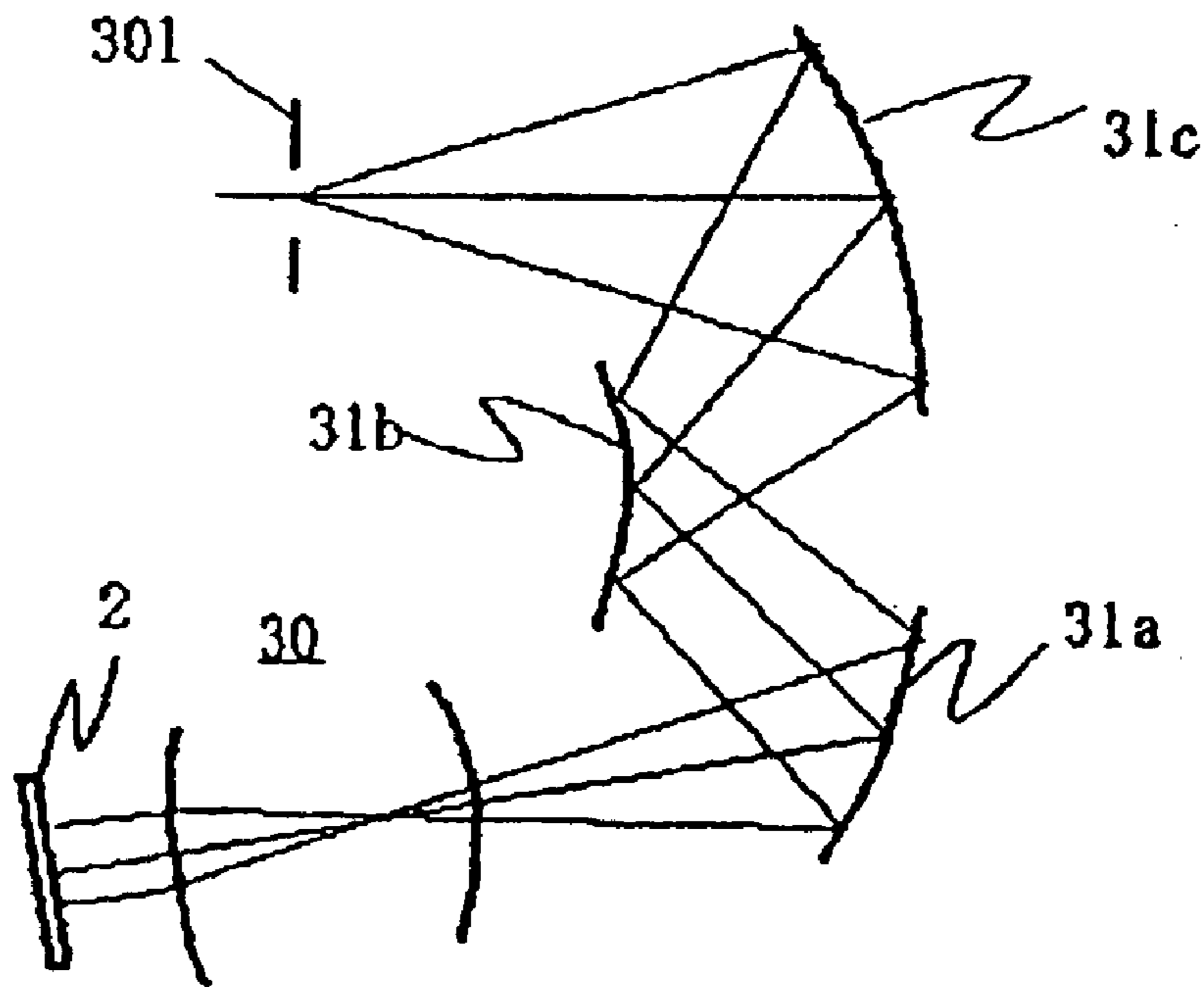
FIG. 44 (PRIOR ART)
