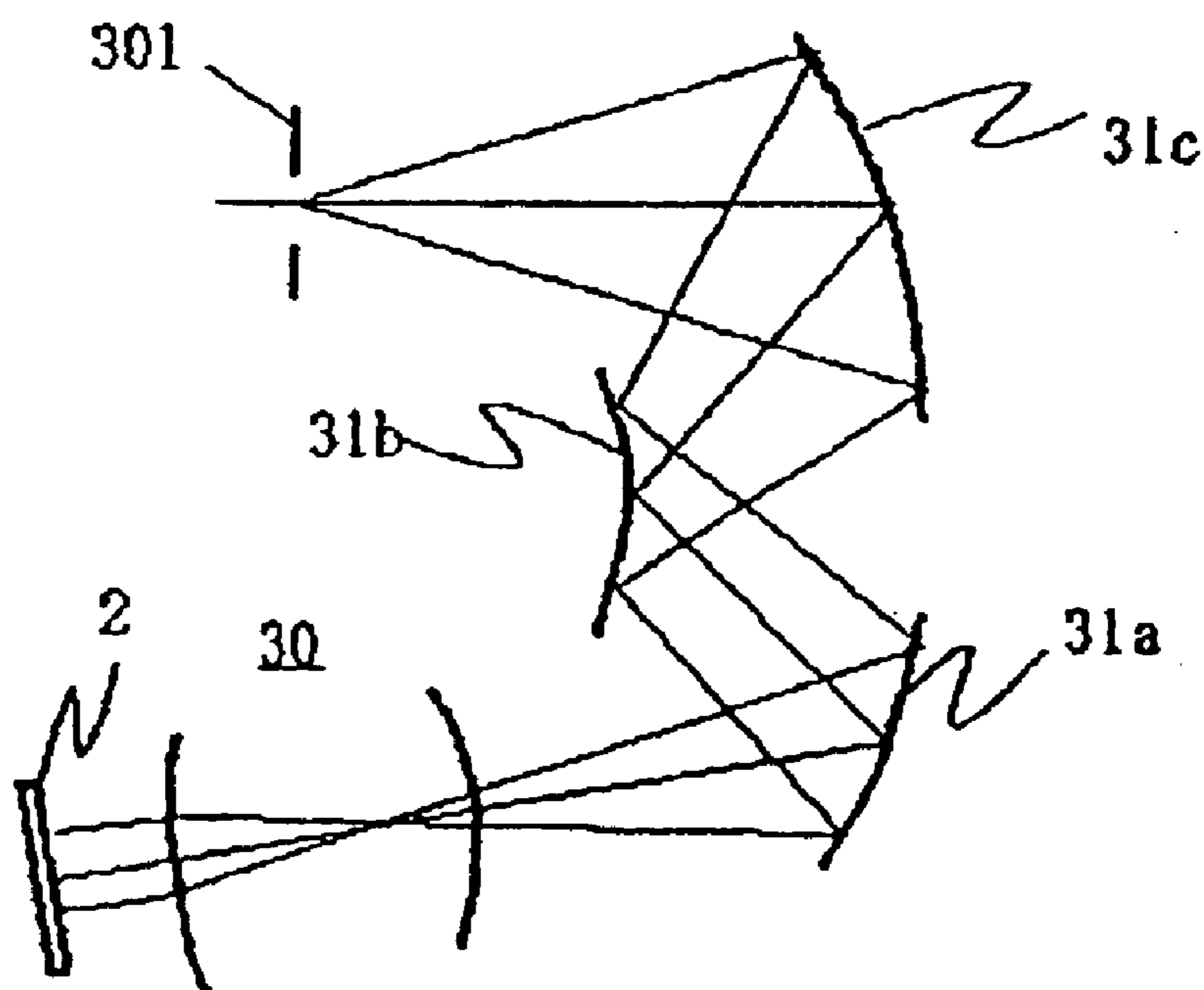
FIG. 44 (PRIOR ART)
