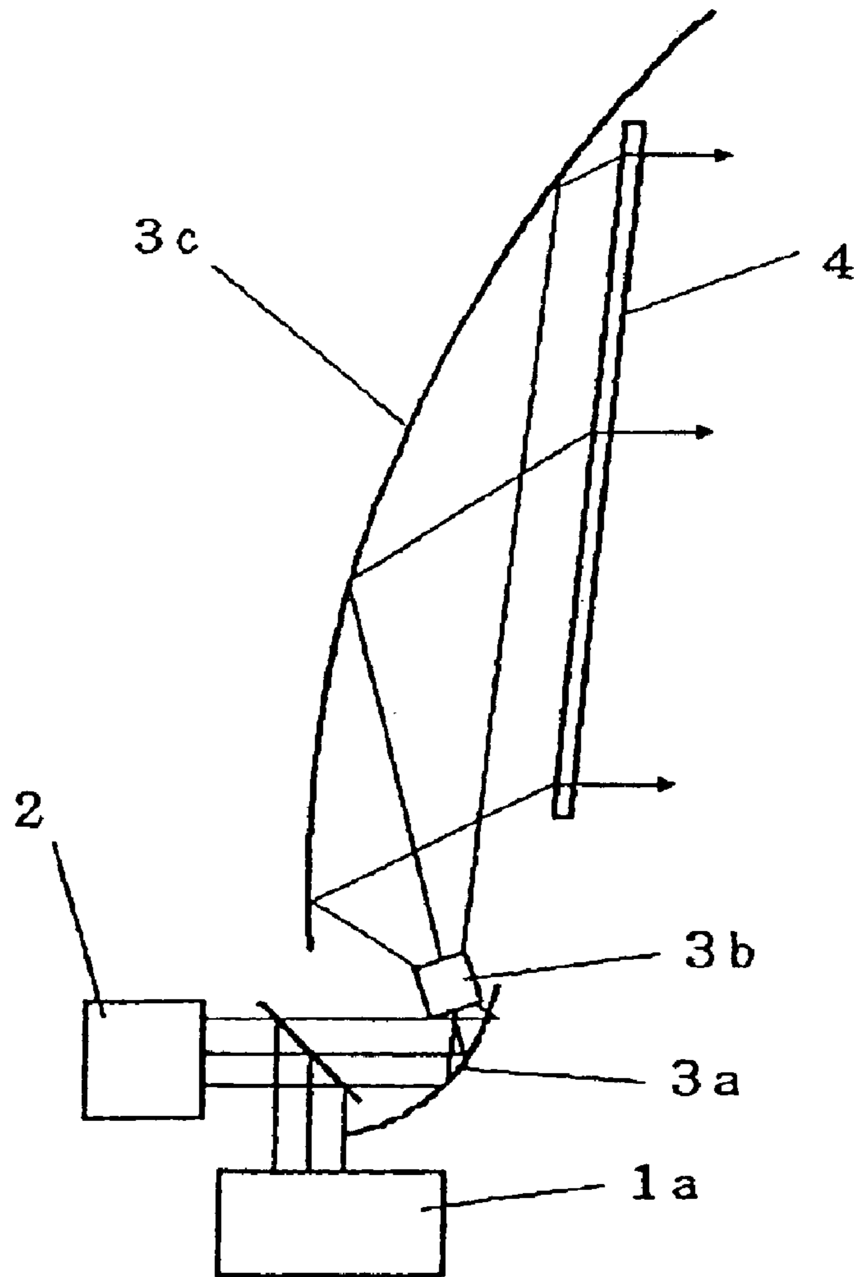
FIG. 37 (PRIOR ART)
