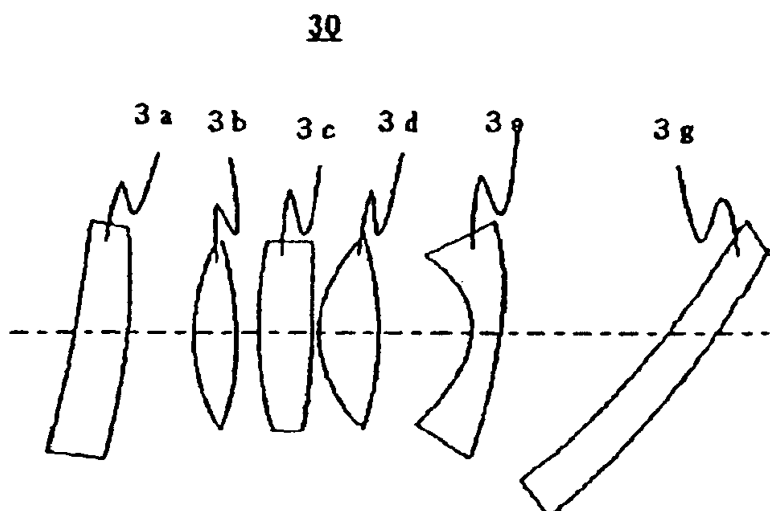
FIG. 39 (PRIOR ART)
