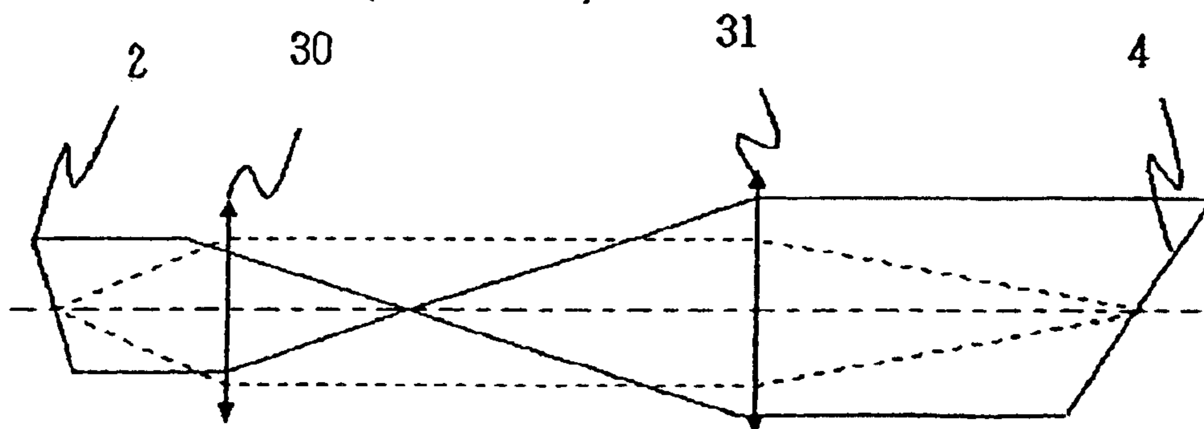
FIG. 39 (PRIOR ART)
