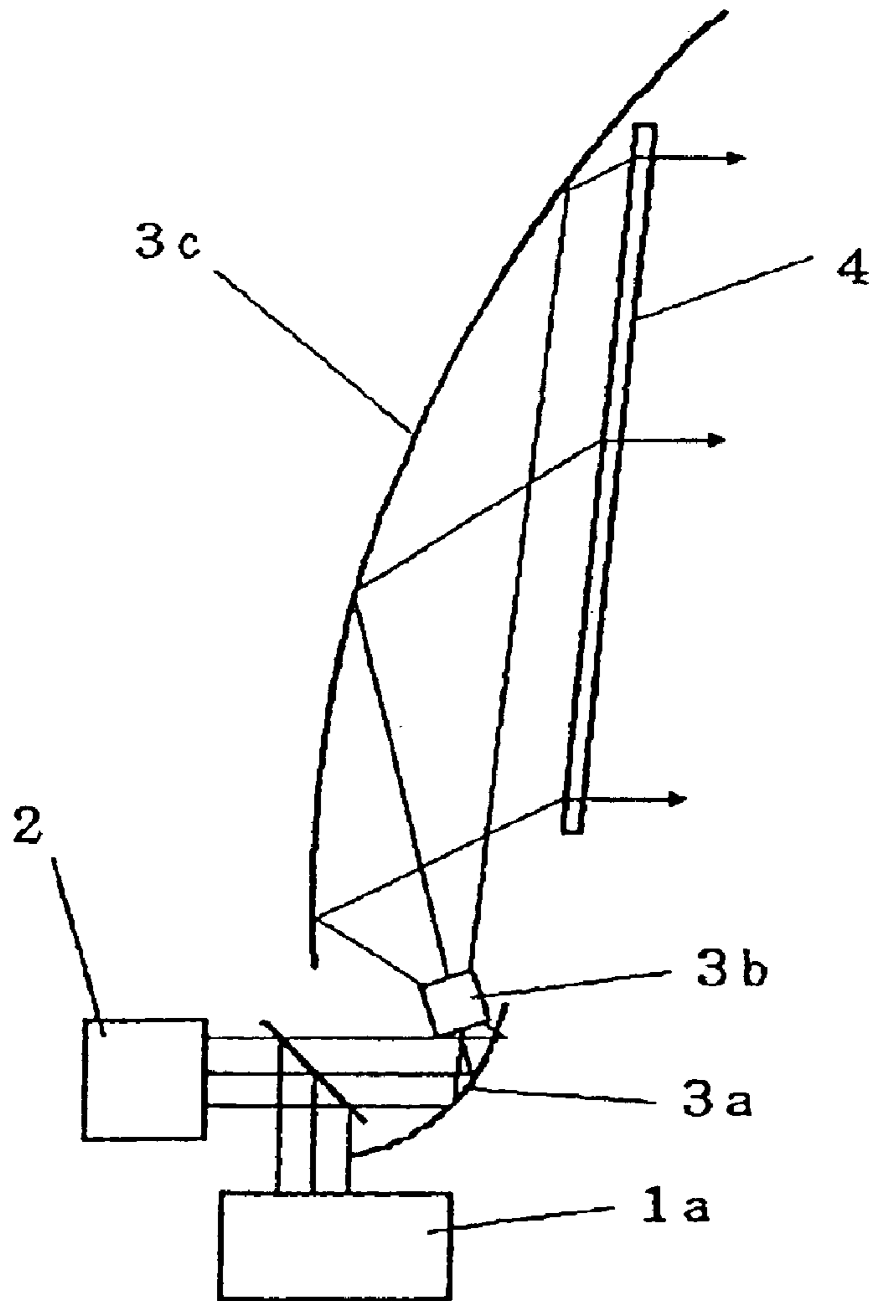
FIG. 37 (PRIOR ART)
