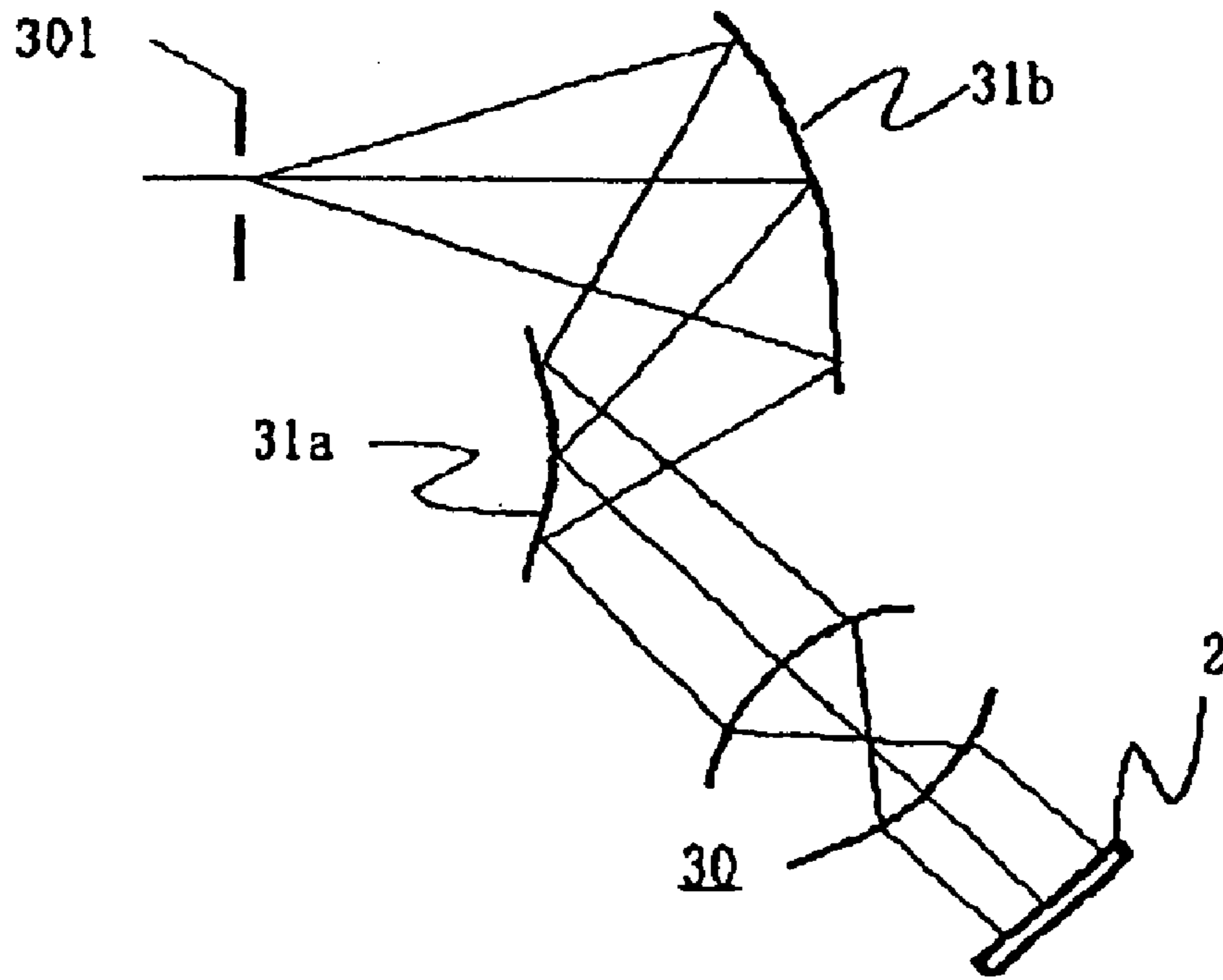
FIG. 43 (PRIOR ART)
