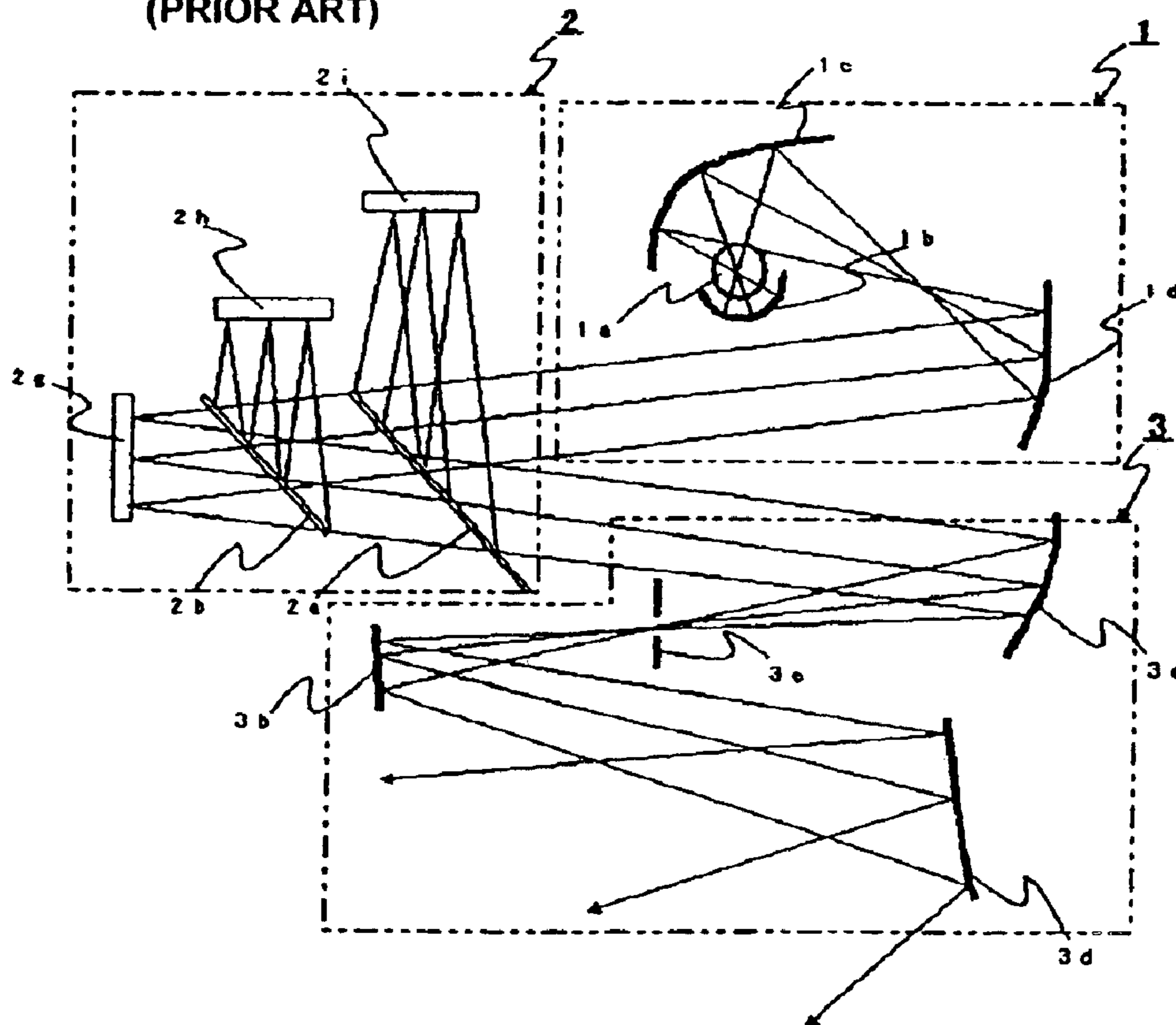
FIG. 28 (PRIOR ART)
