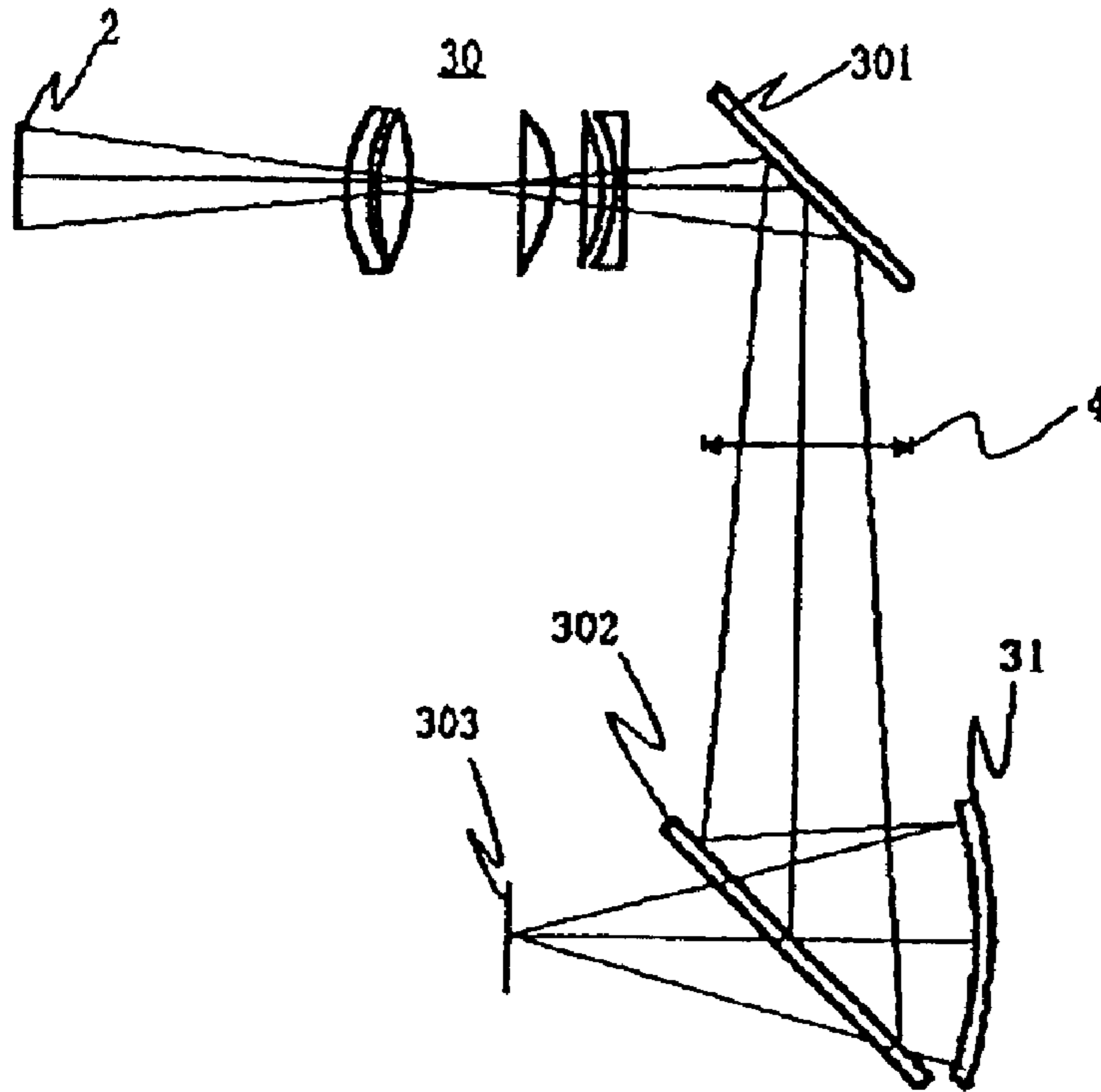
FIG. 41 (PRIOR ART)
