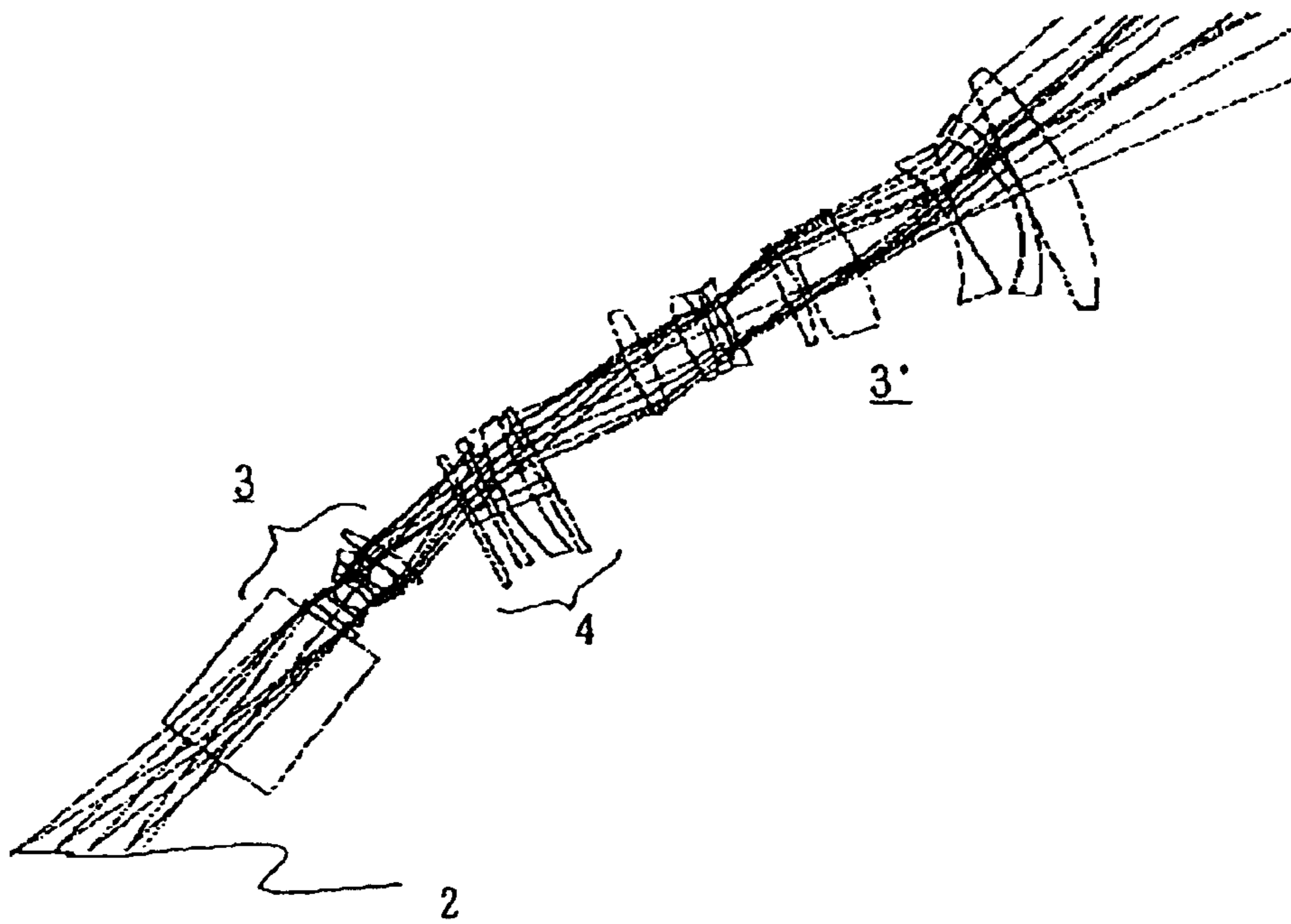
FIG. 34 (PRIOR ART)
