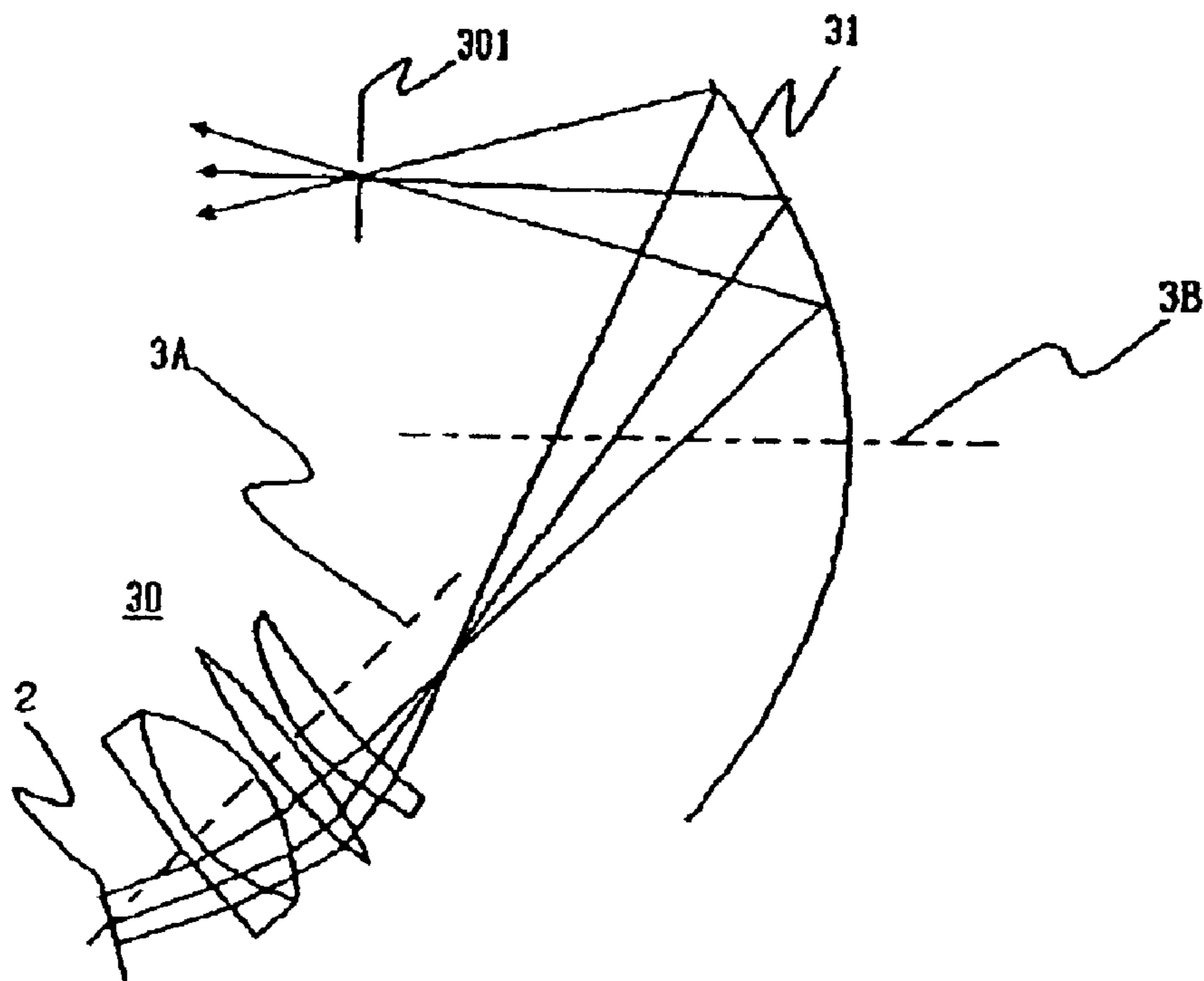
FIG. 41 (PRIOR ART)
