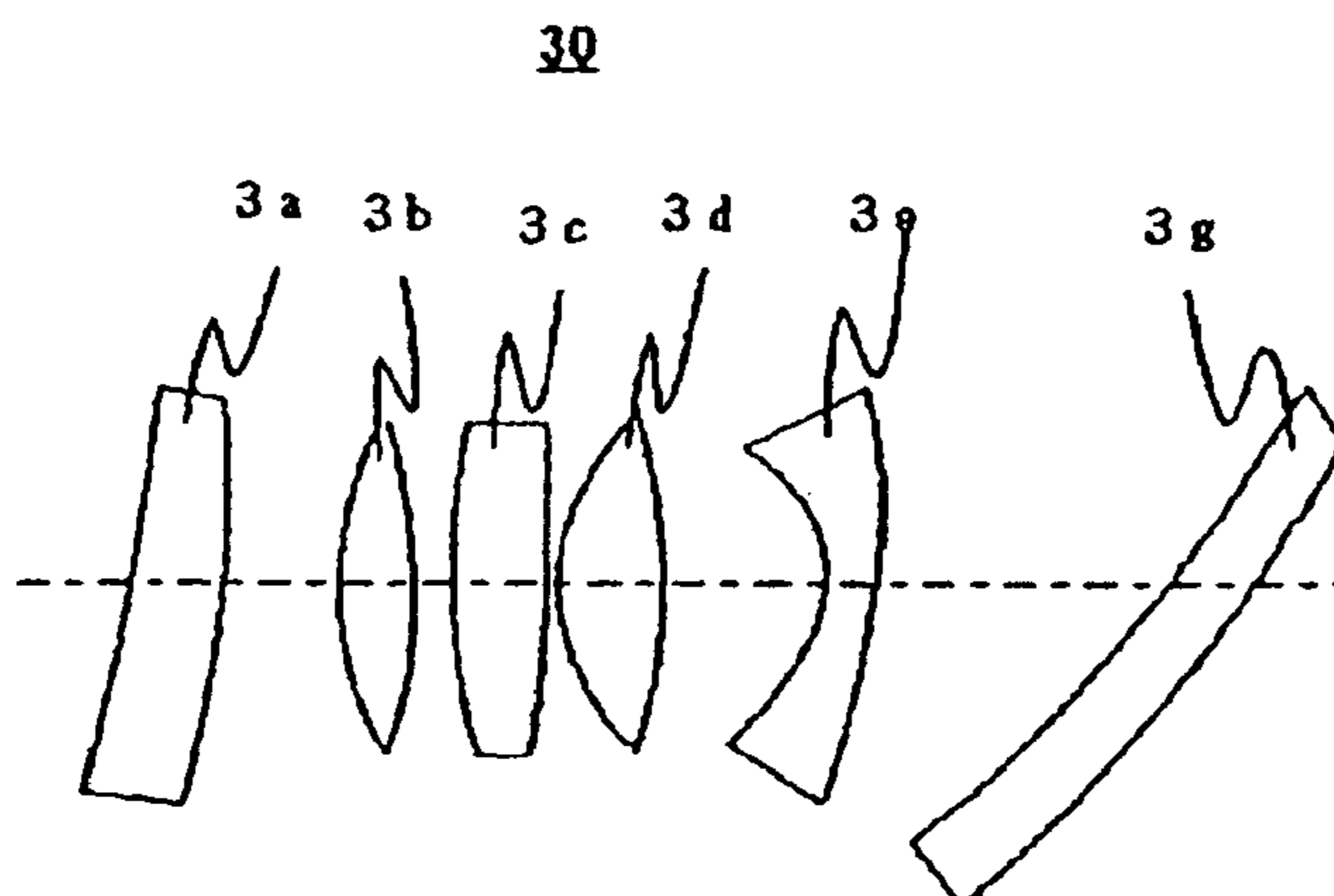
FIG. 39 (PRIOR ART)
