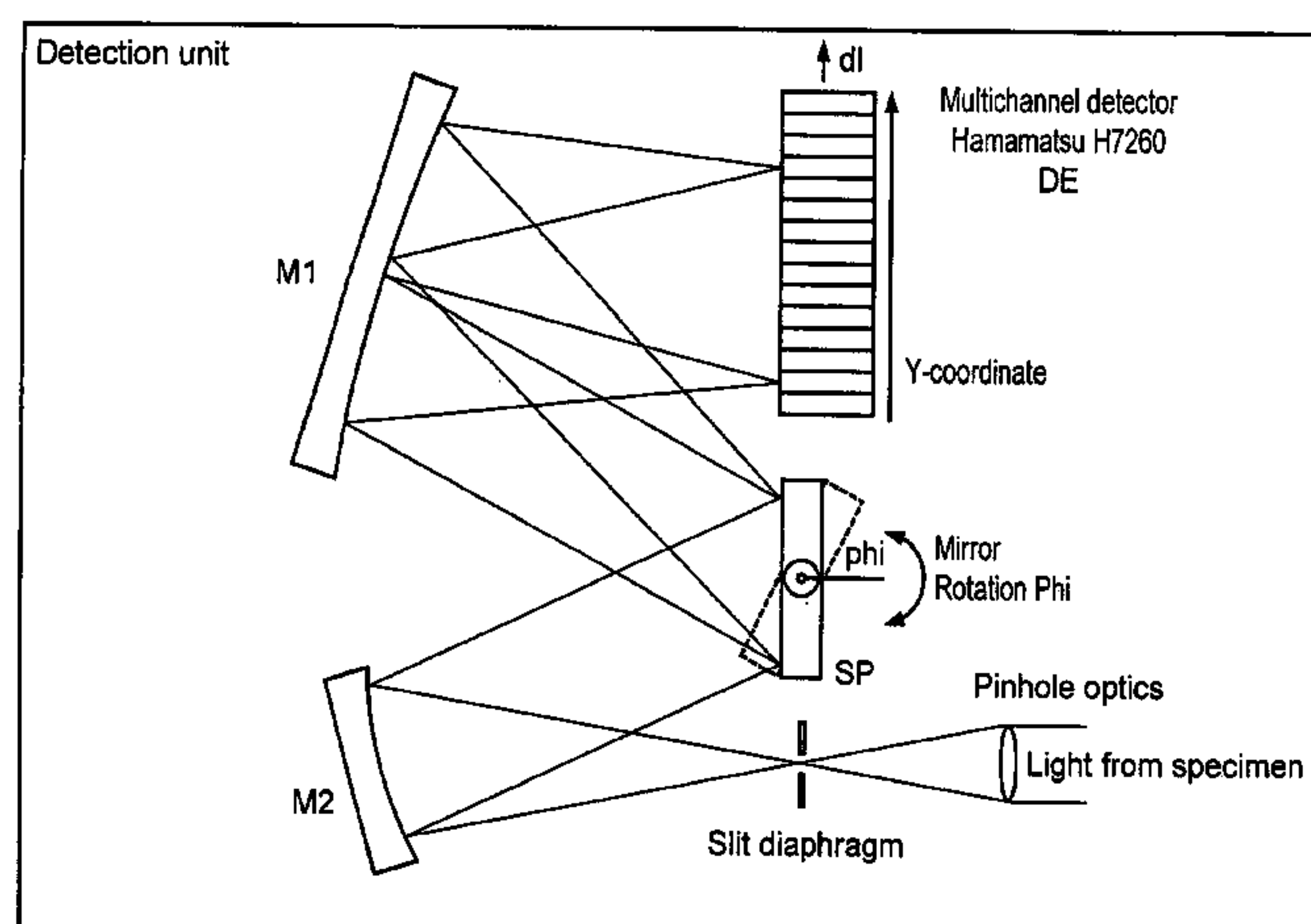
Example of detector unit / optics construction for line scanner
