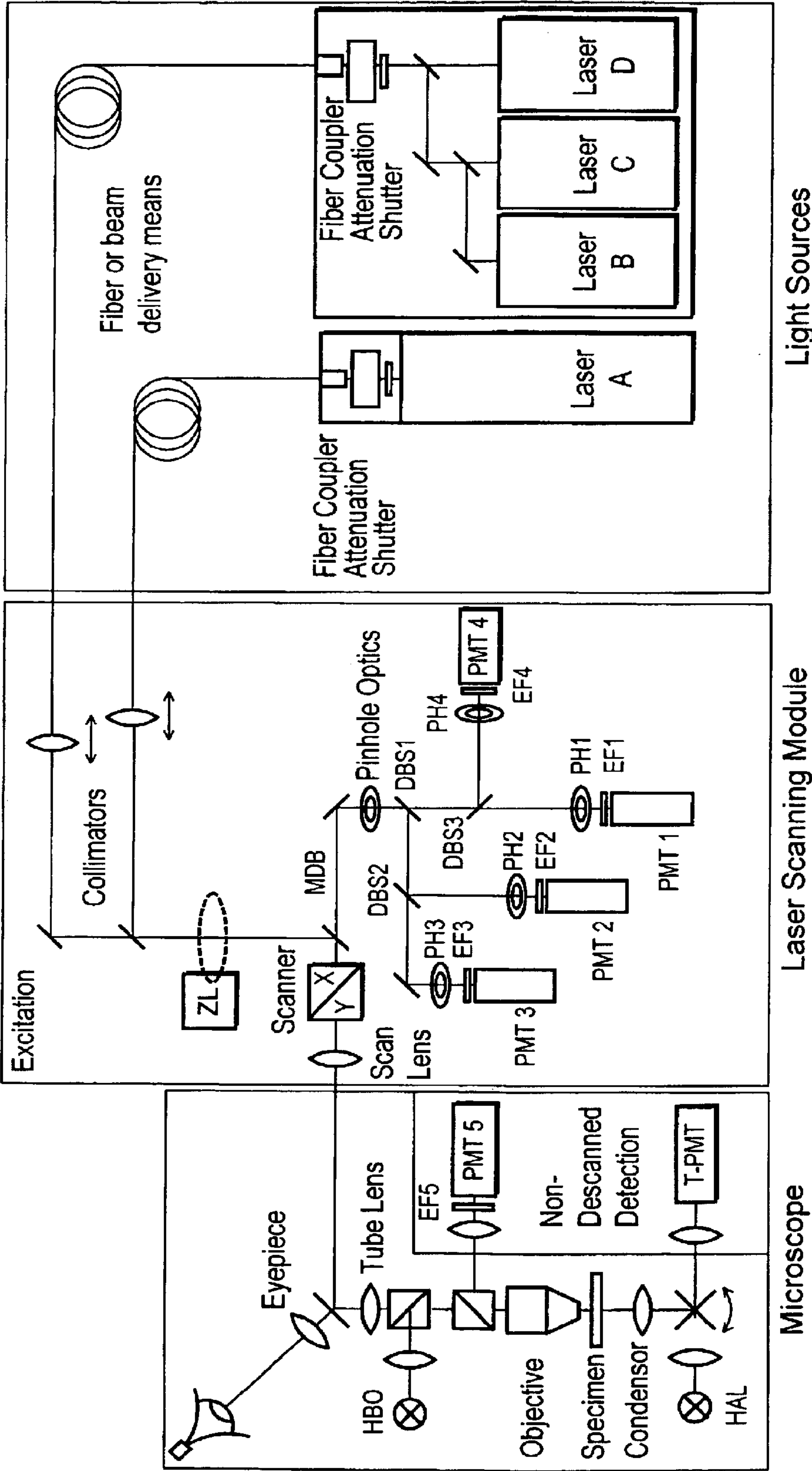
LSM Construction FIG. 2 PRIOR ART
