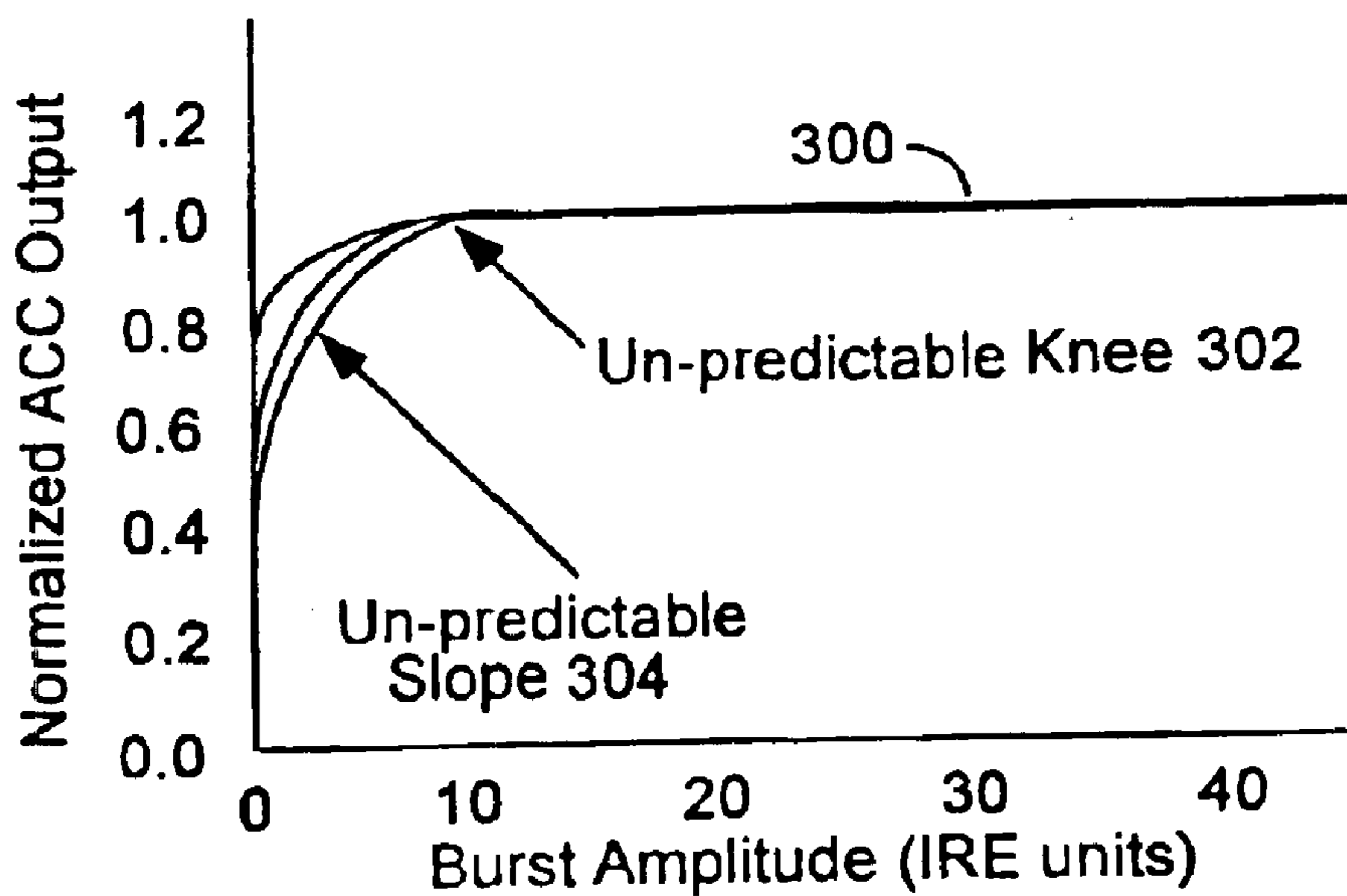
FIG. 3 (Prior Art)
