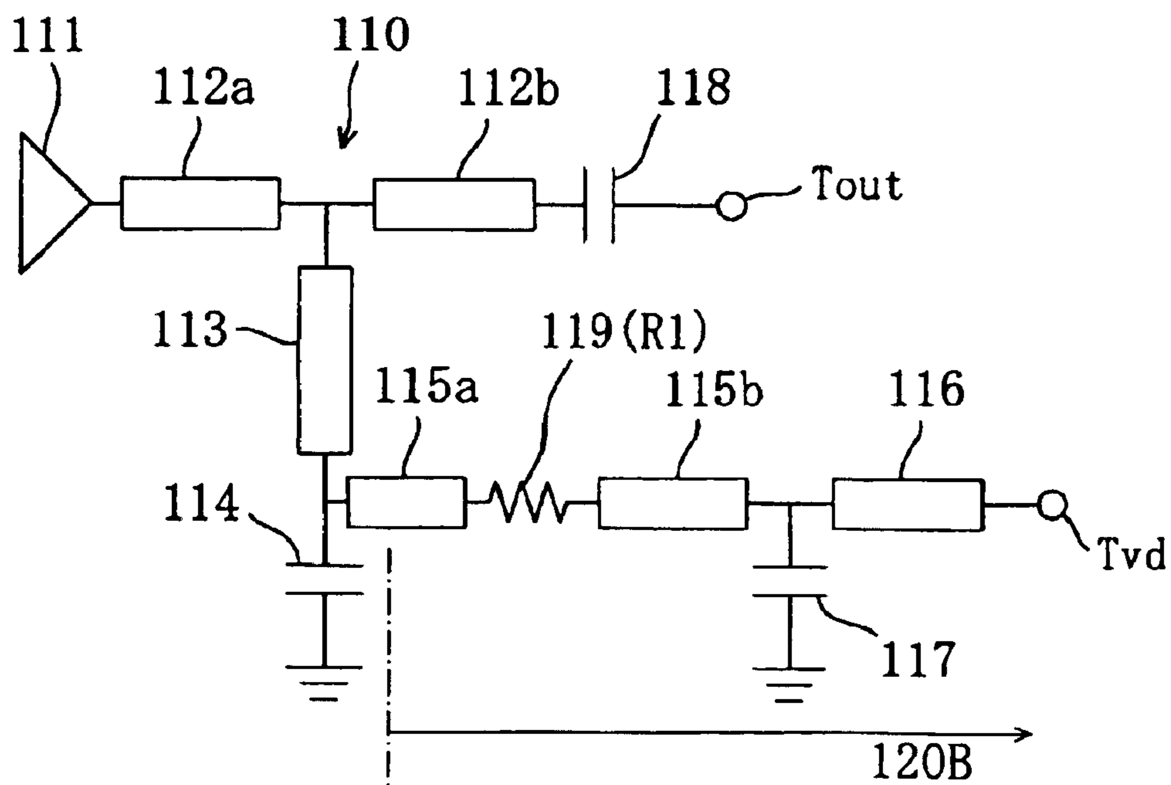
Fig. 24 PRIOR ART
