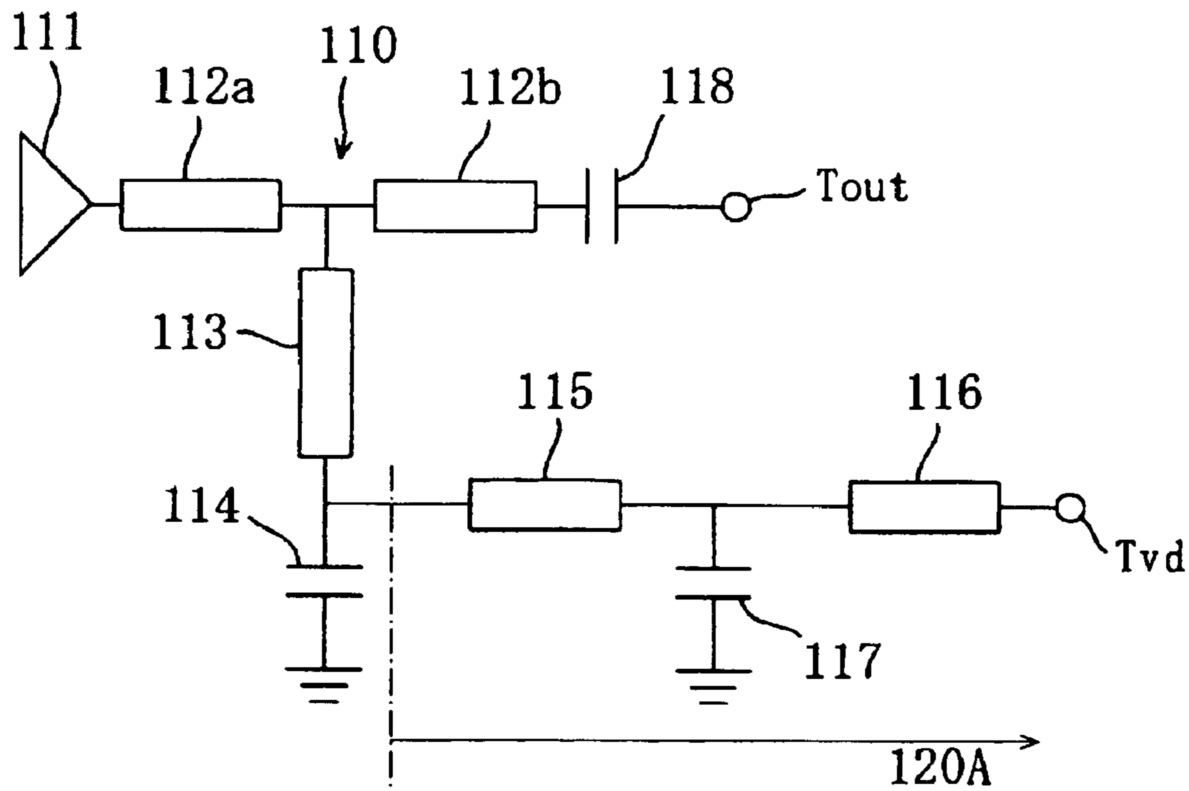
Fig. 23 PRIOR ART
