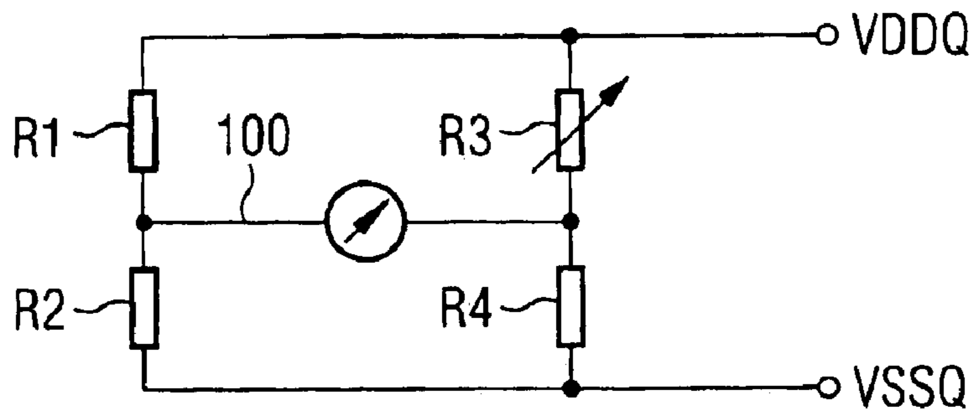
FIG 1 Prior Art
