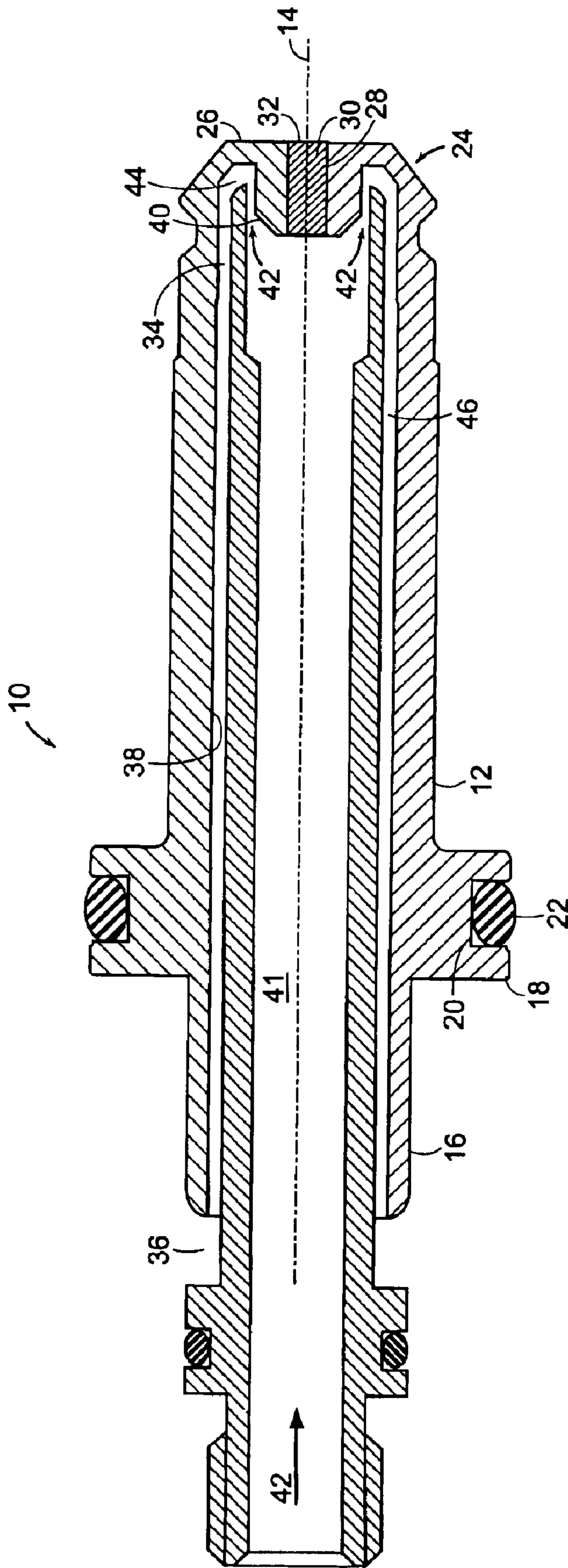
FIG. 1 PRIOR ART
