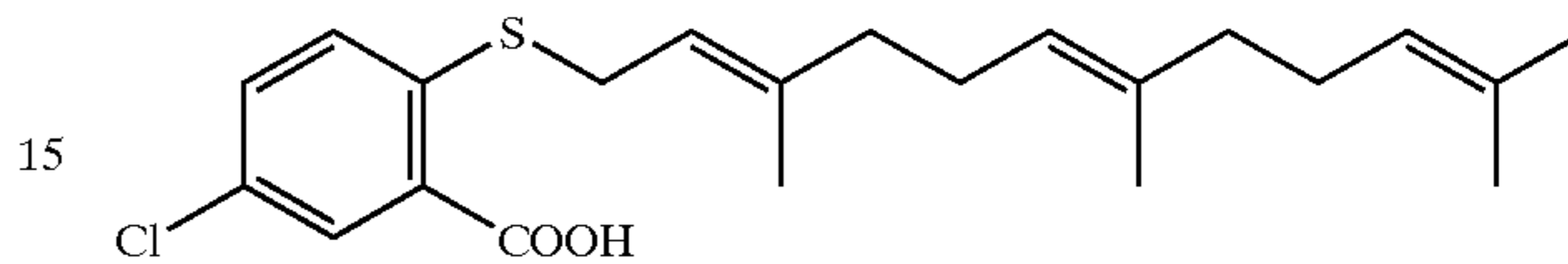
5-Cl-FTS
