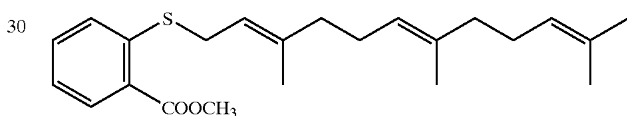
5-F-FTS
