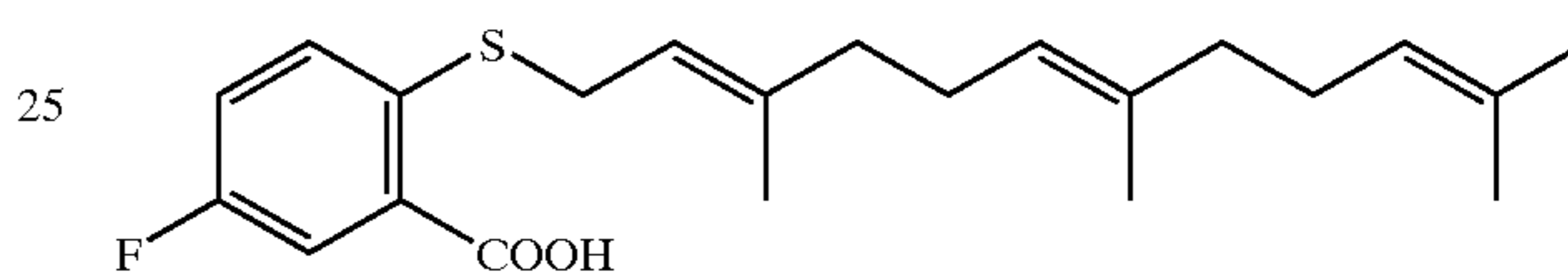
5-F-FTS
