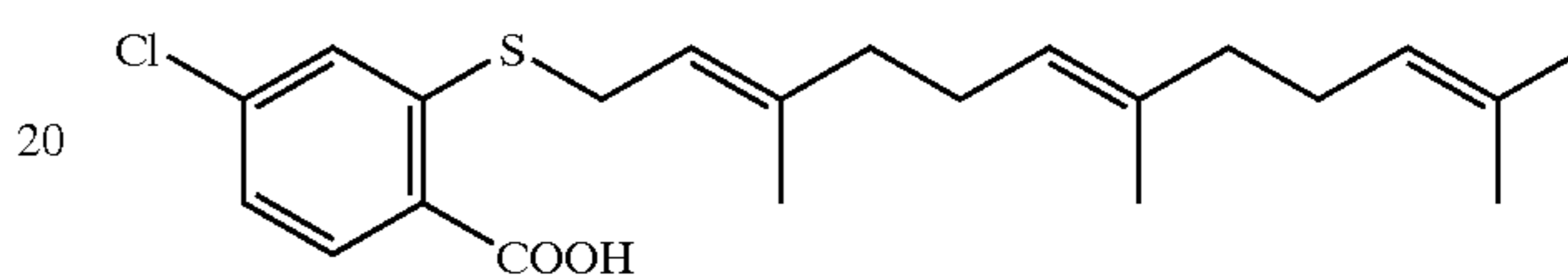
4-Cl-FTS
