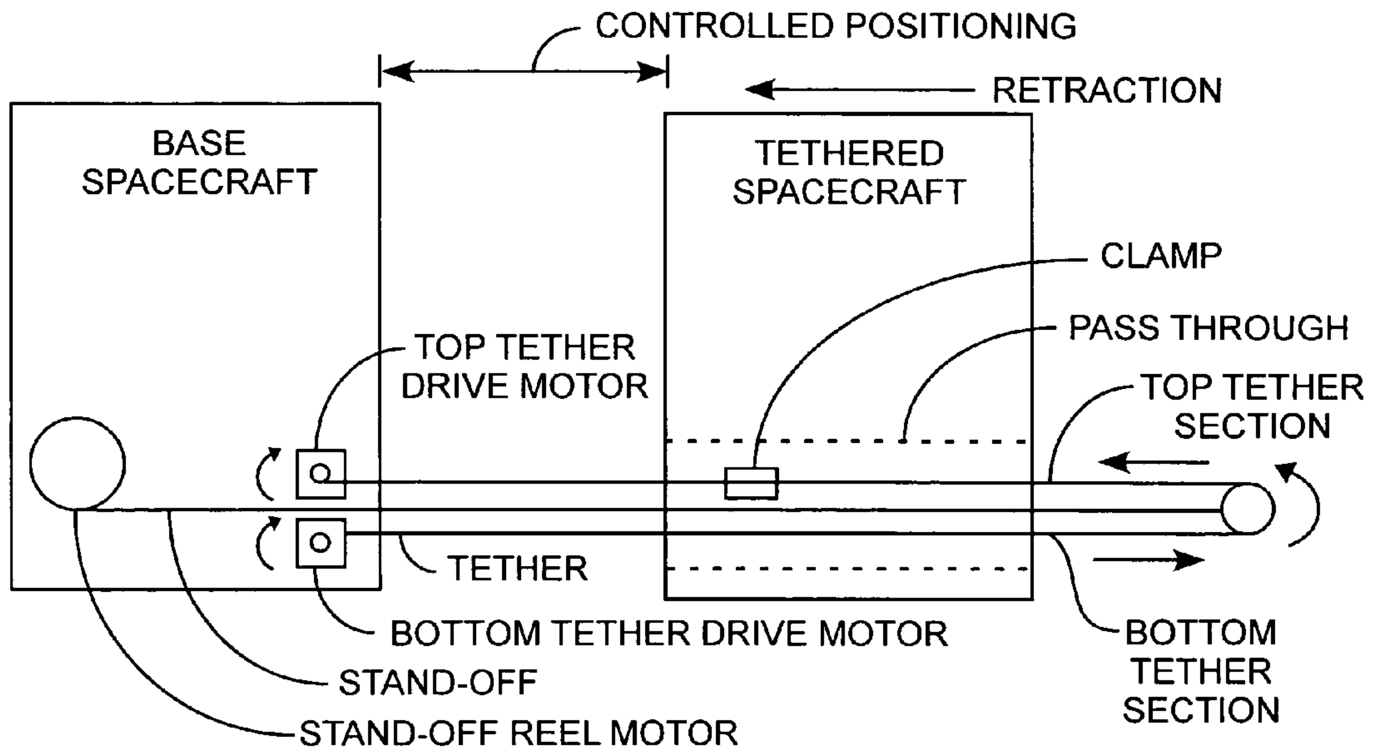
TETHERED SPACECRAFT RETRACTED POSITIONING
