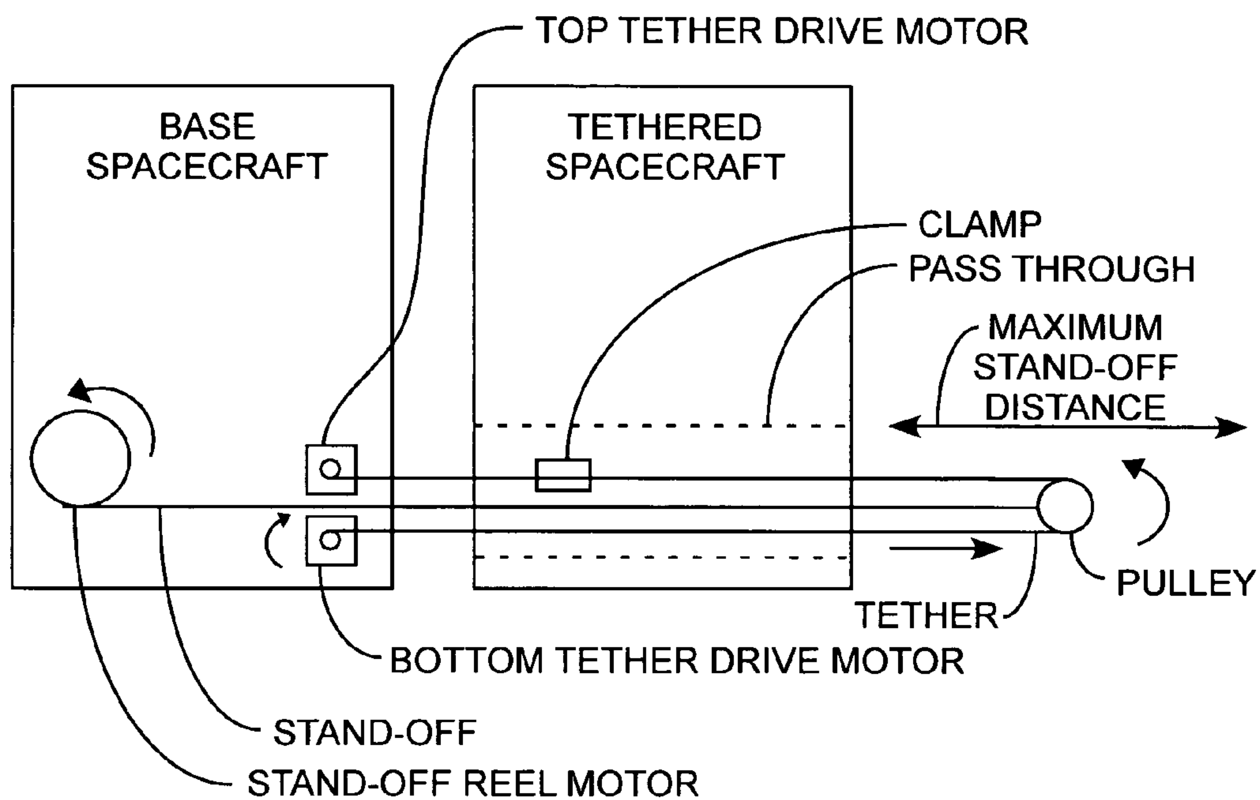
BASE SPACECRAFT AND TETHERED SPACECRAFT WITH EXTENDED STAND-OFF
