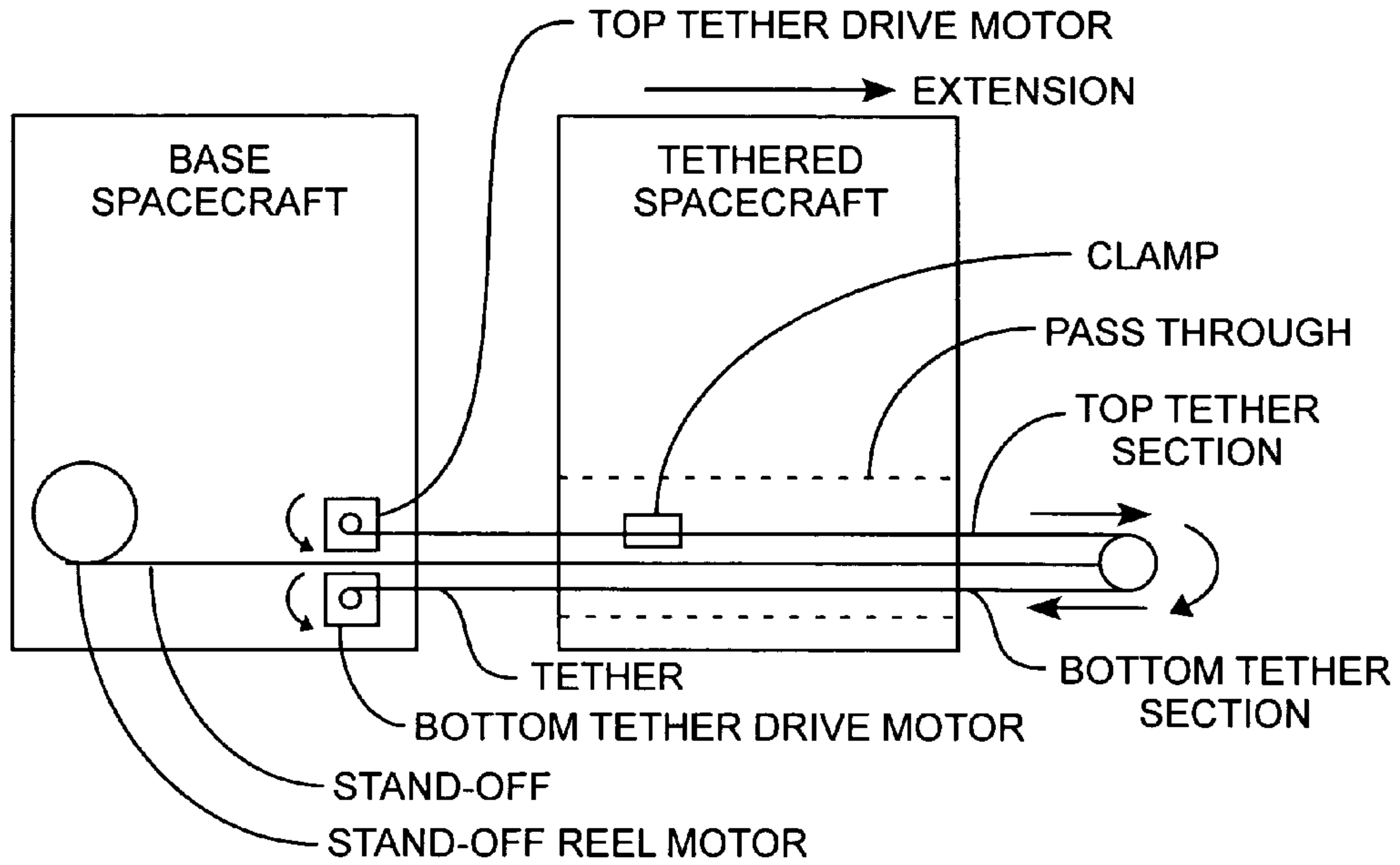
TETHERED SPACECRAFT EXTENDED POSITIONING
