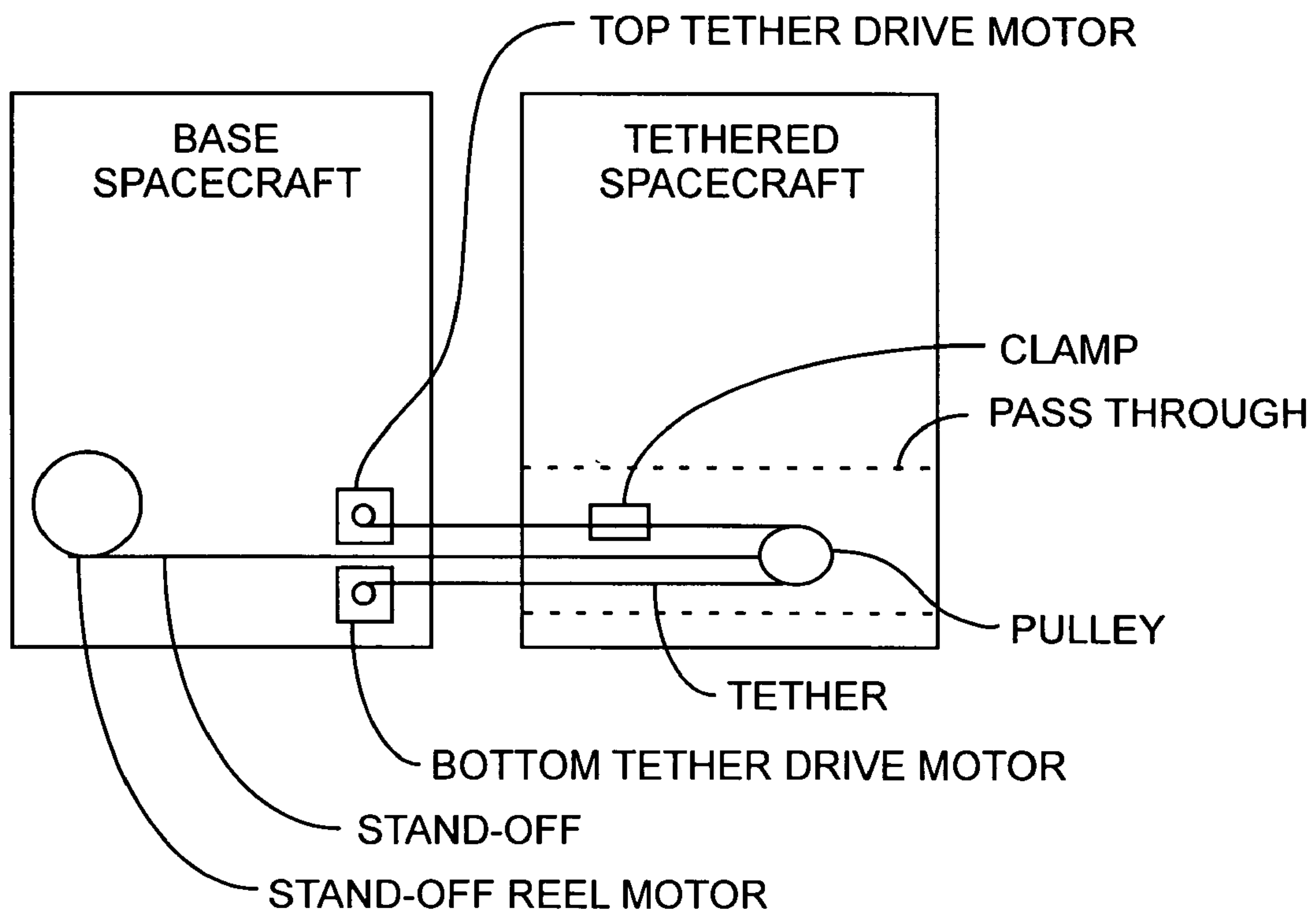
BASE SPACECRAFT AND TETHERED SPACECRAFT IN A STOWED RETRACTED POSITION
