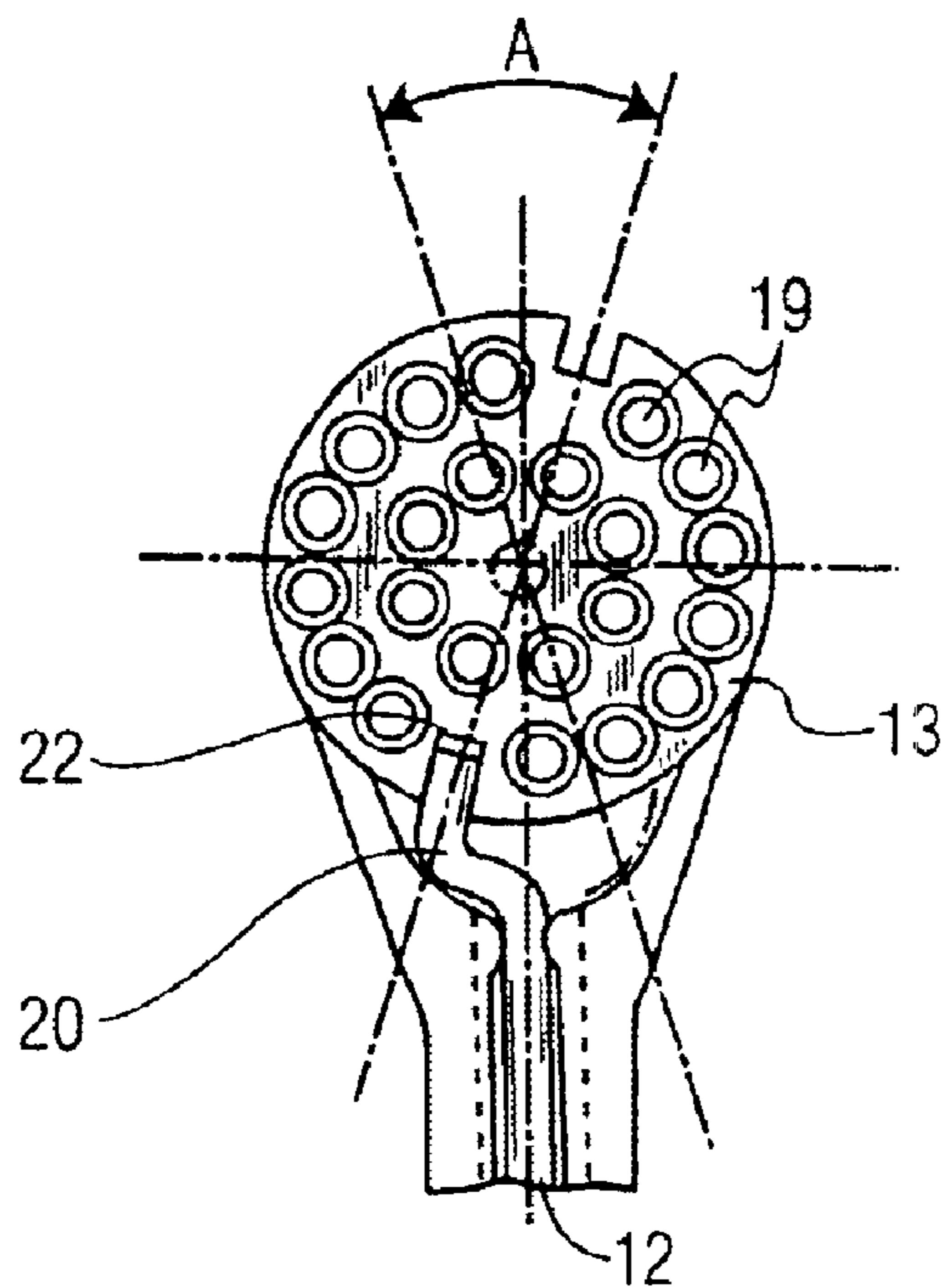
FIG. 1C PRIOR ART
