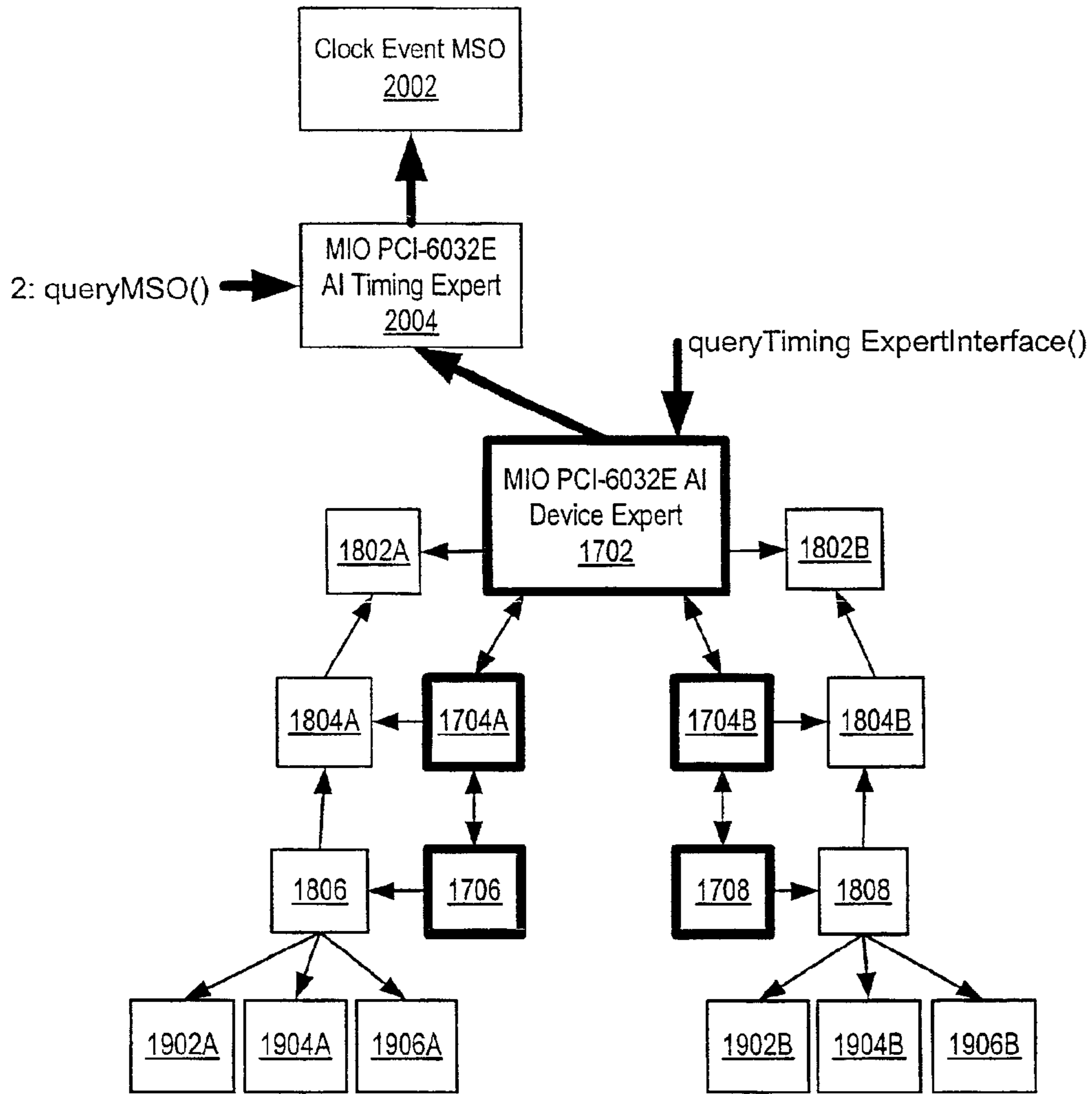
Configure Timing Experts
