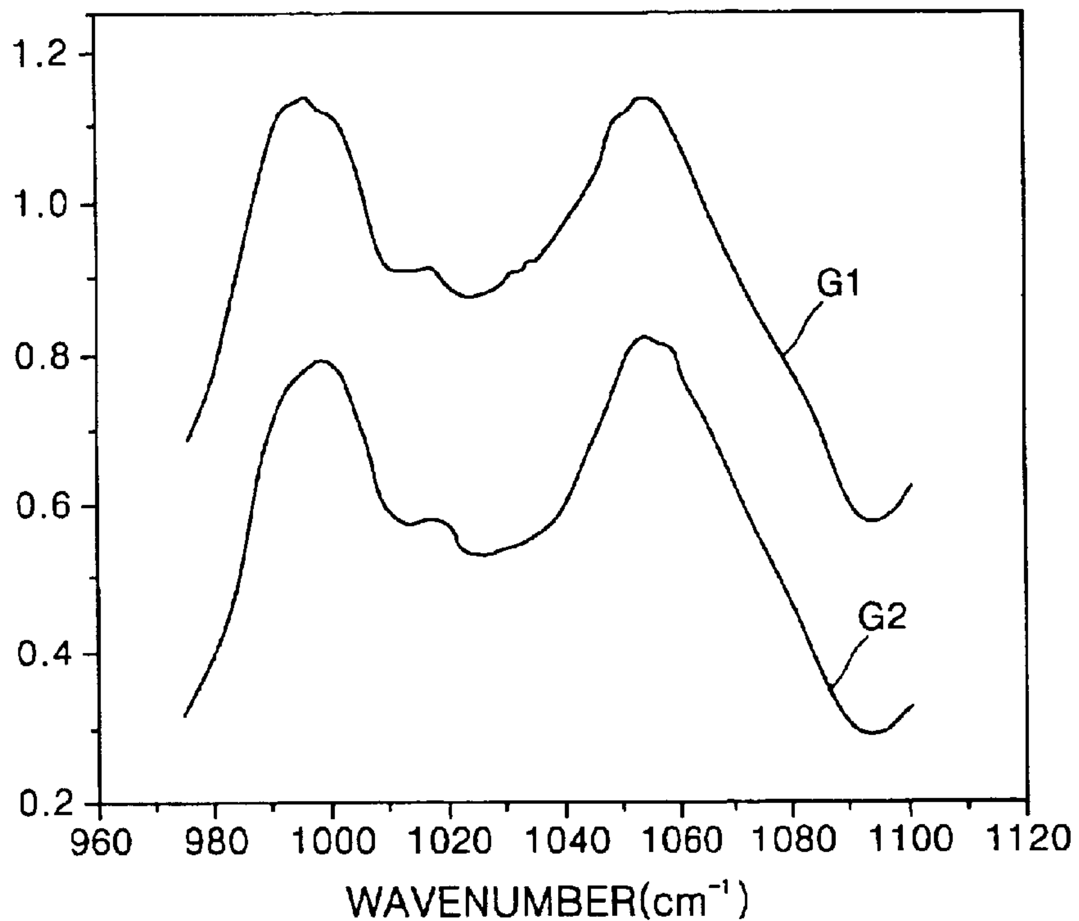
FIG. 5B GLUCOSE
