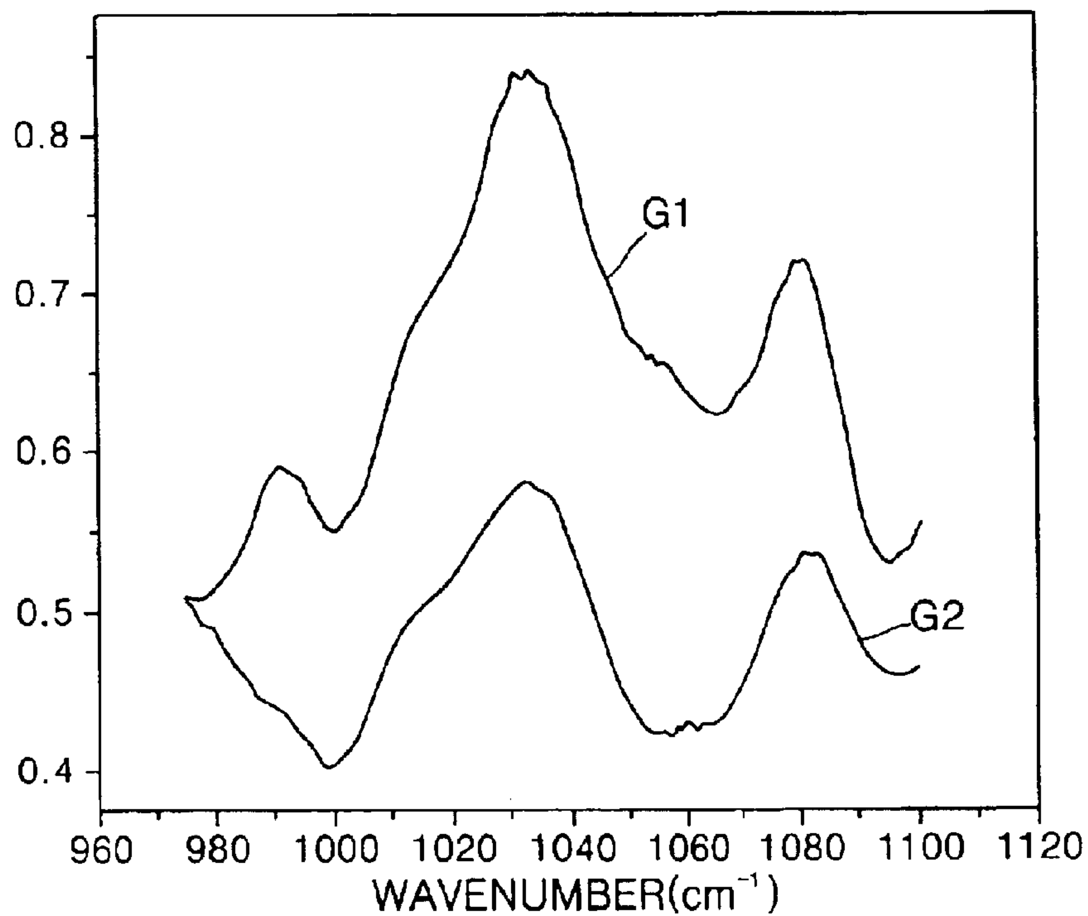
FIG. 5B GLUCOSE
