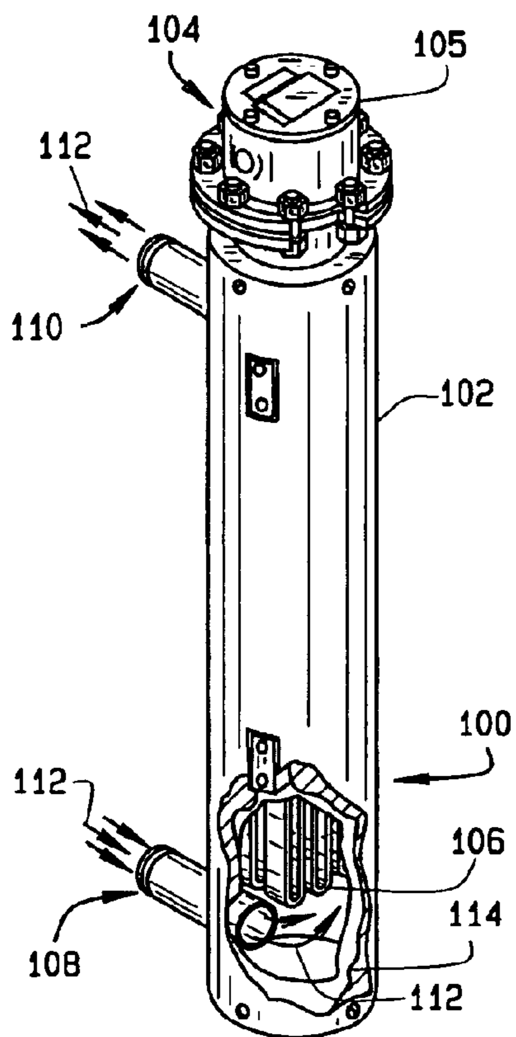
FIG. 9 PRIOR ART
