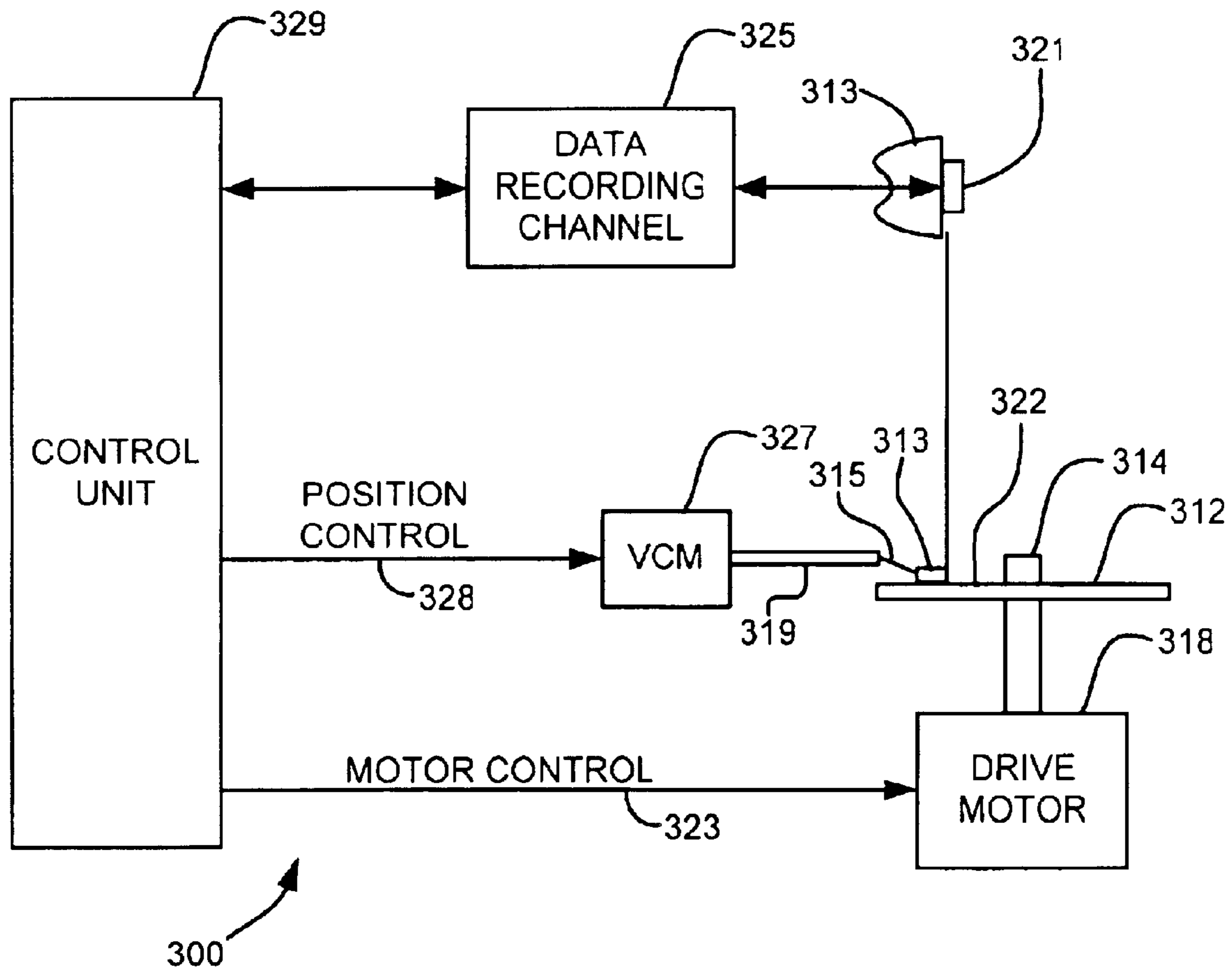
FIG. 3 (prior art)
