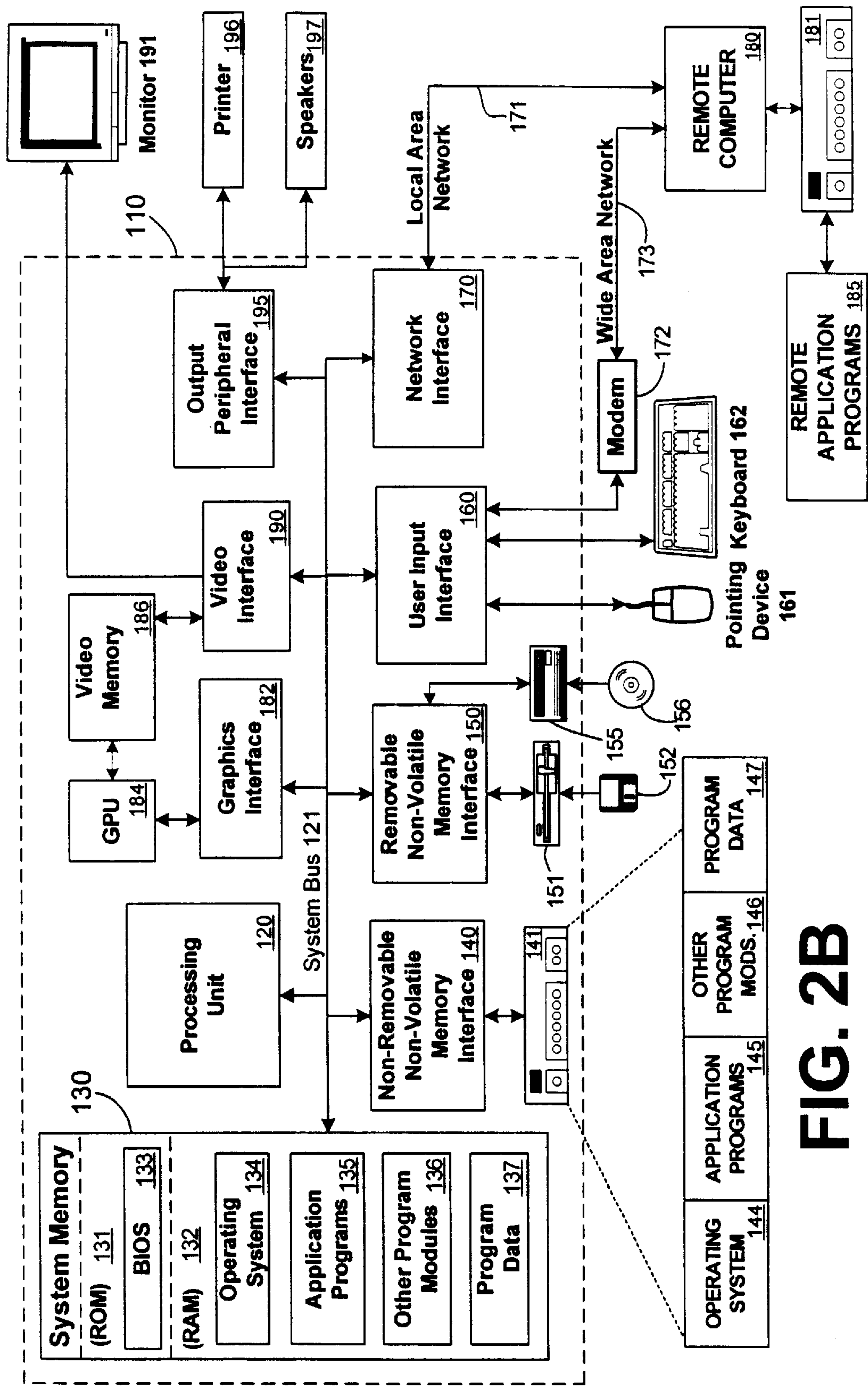
Computing Environment 100
