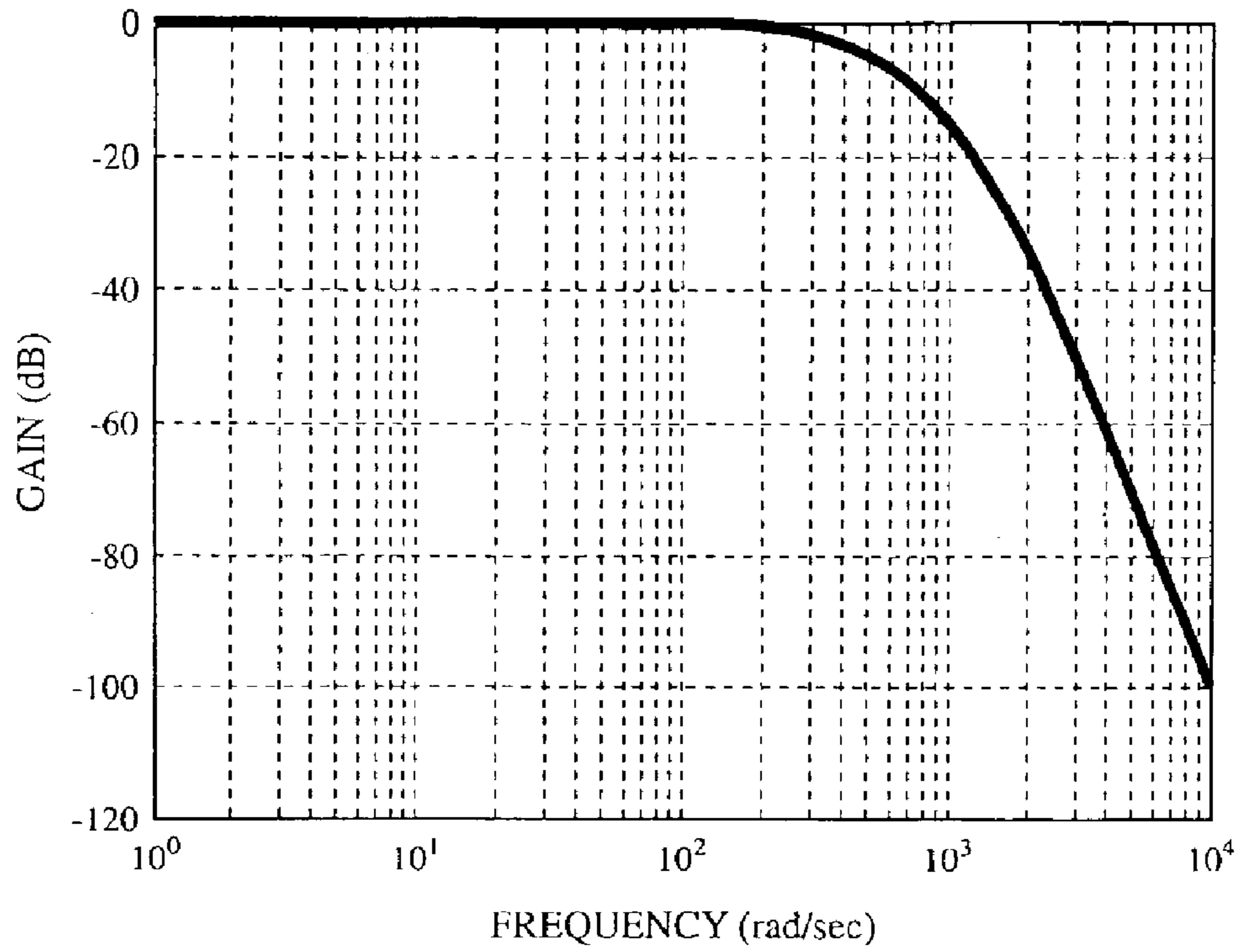
GAIN CURVE
