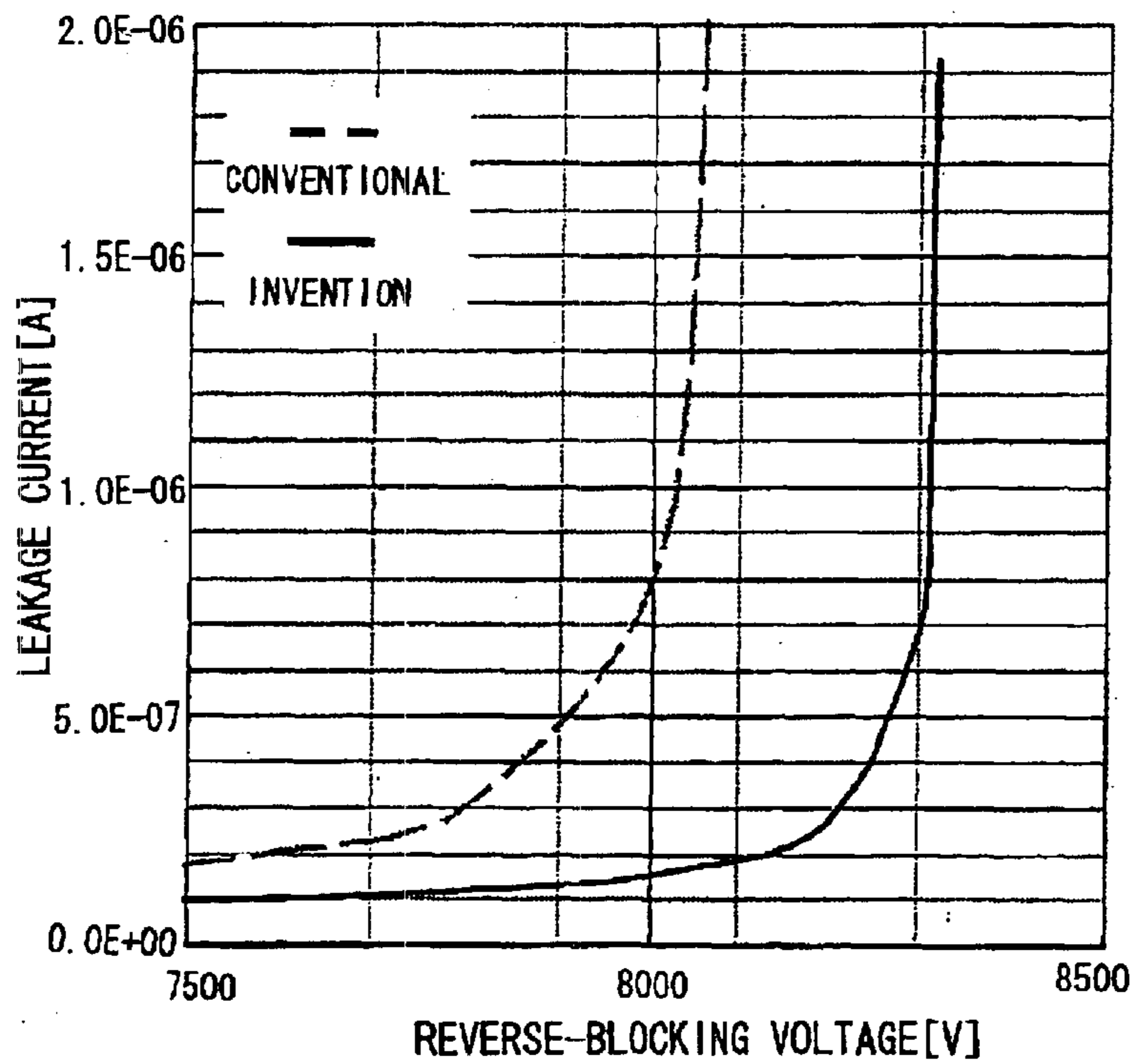
FIG. 9 REVERSE-BLOCKING VOLTAGE CHARACTERISTICS
