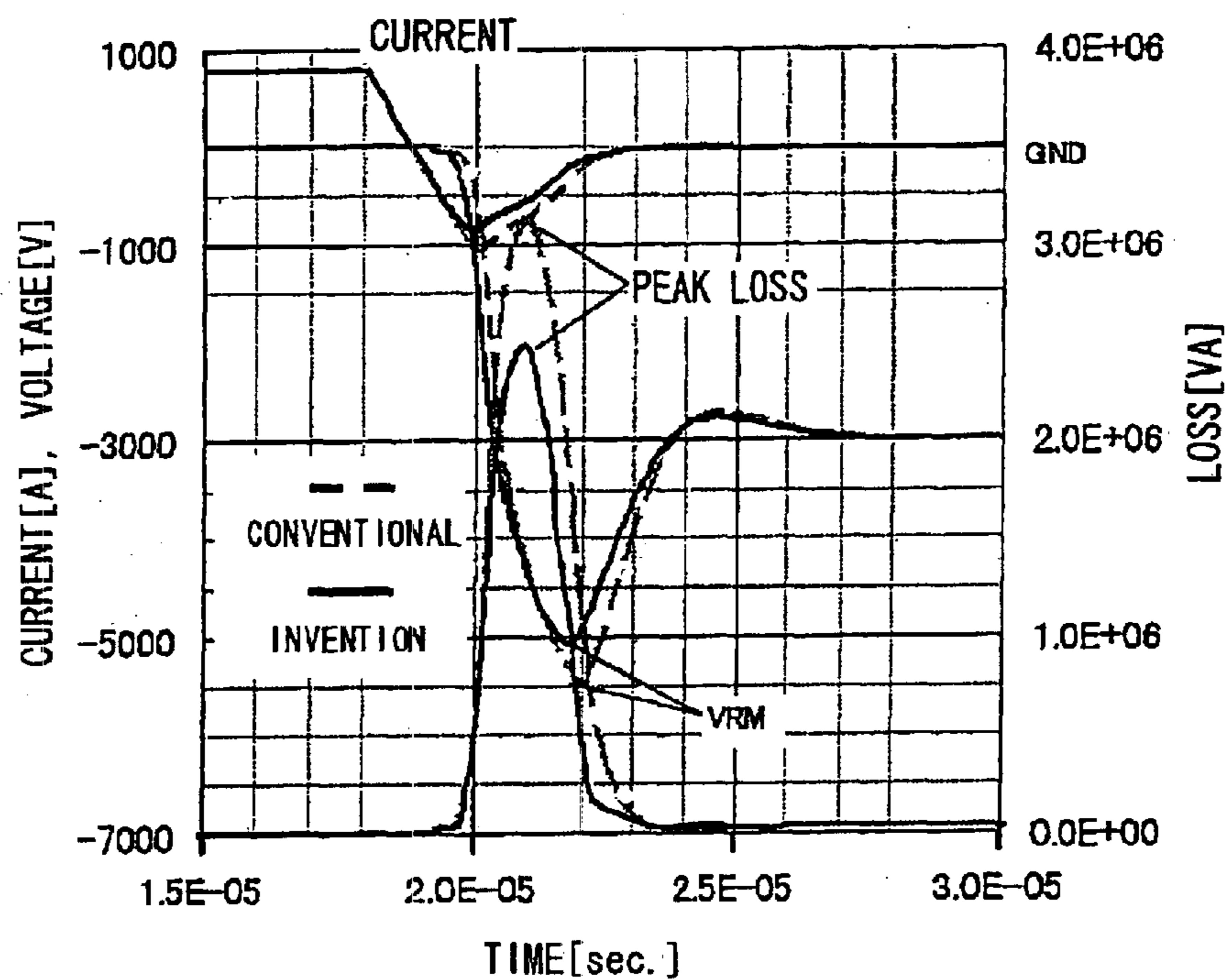
FIG. 8 REVERSE RECOVERY CHARACTERISTICS
