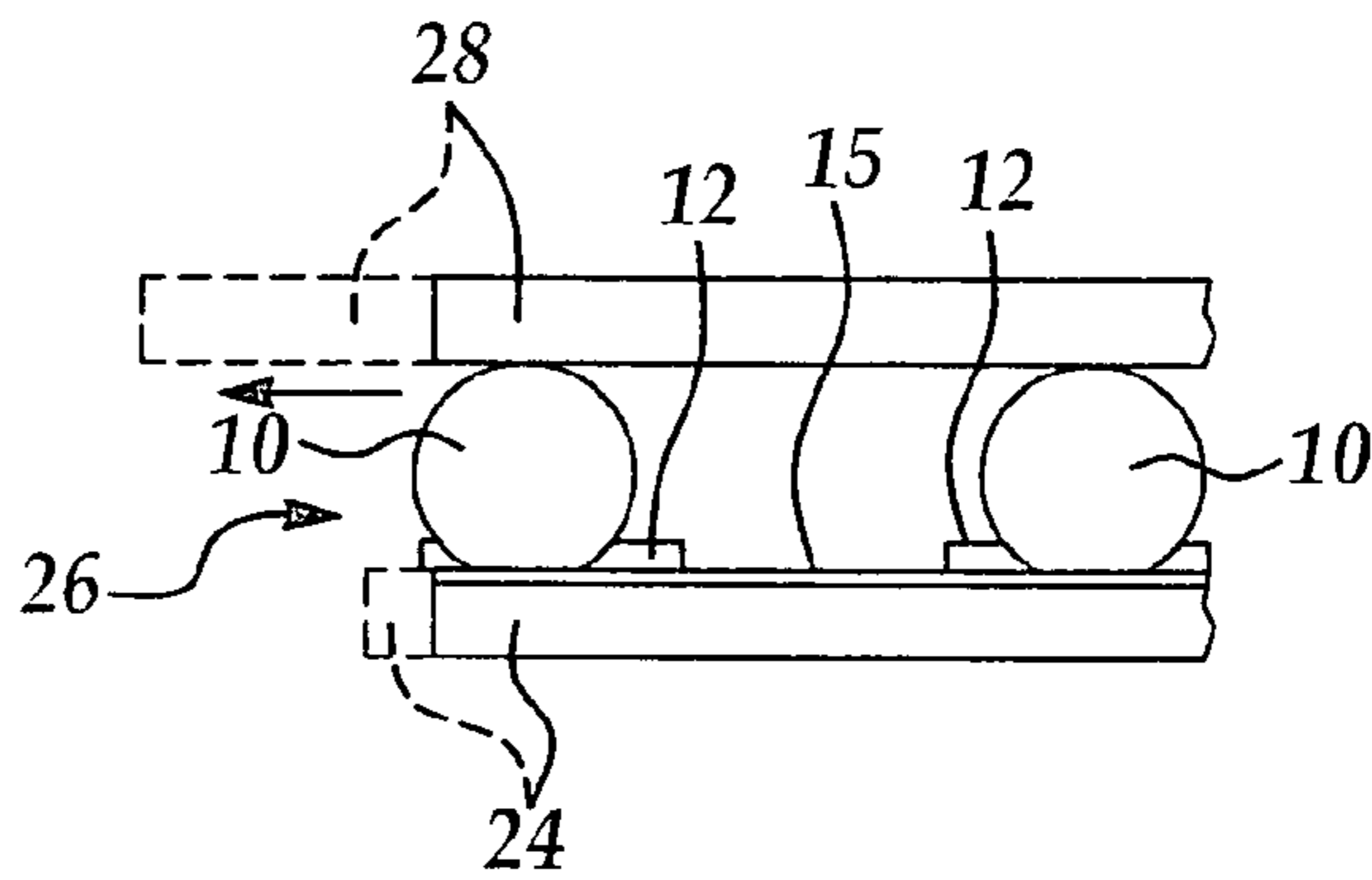
Figure 1C Prior Art
