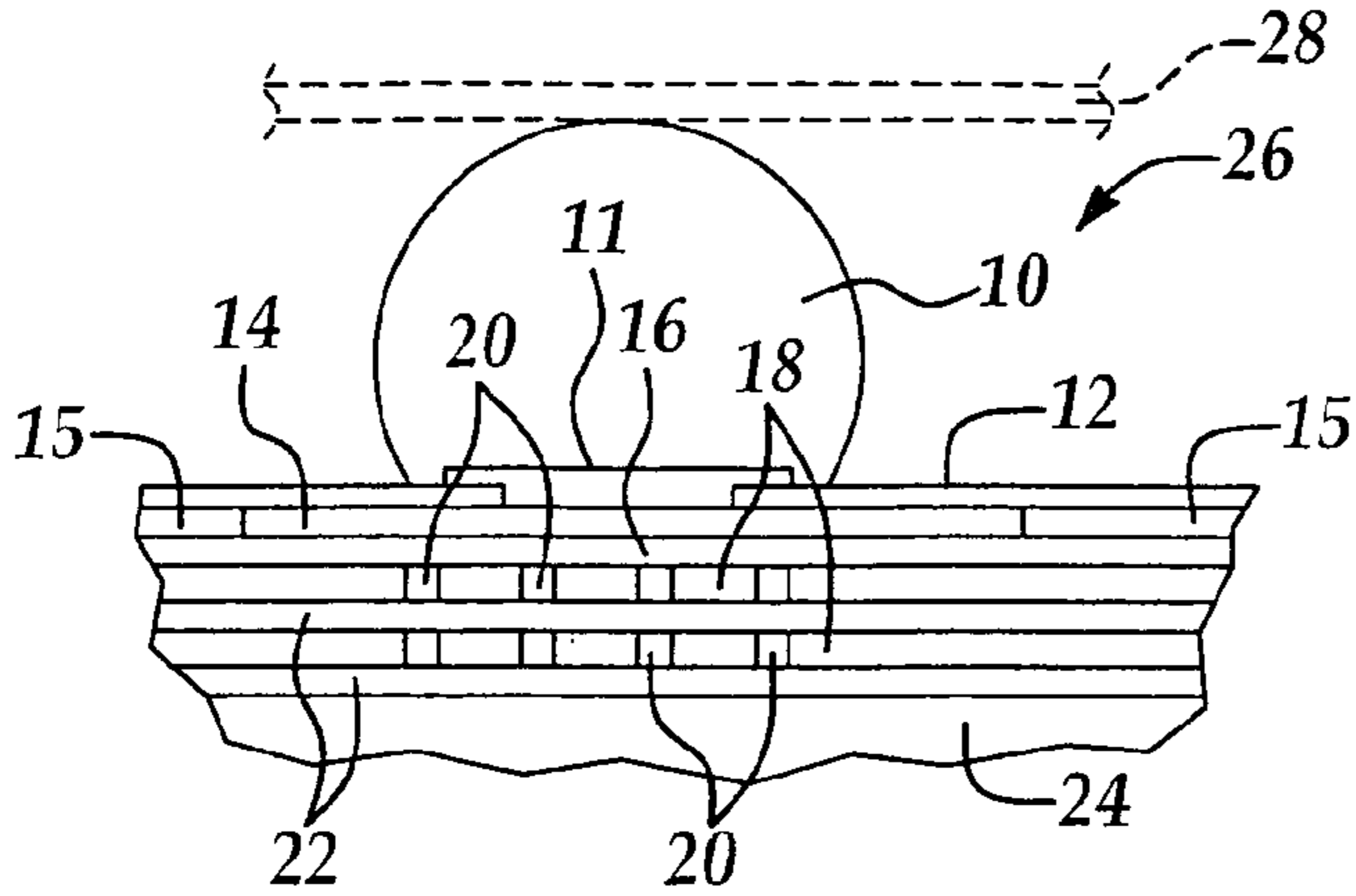
Figure 1 Prior Art
