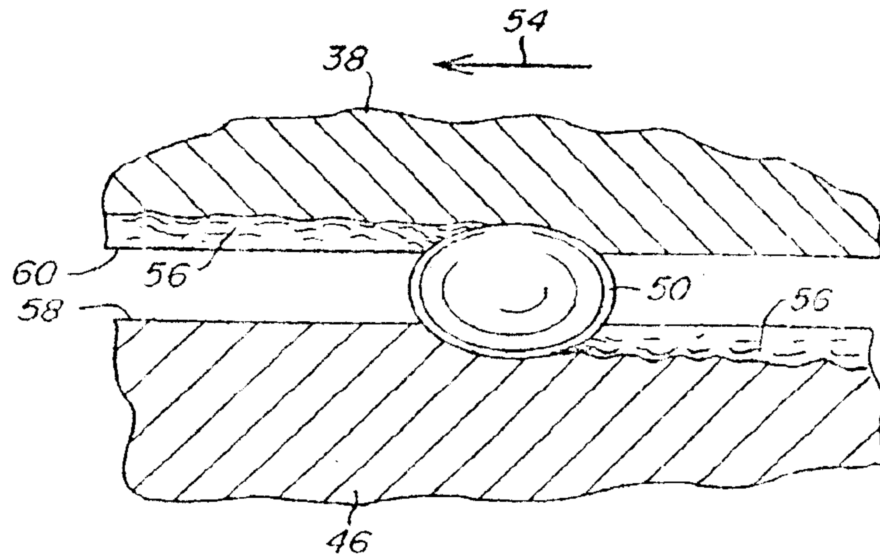
Fig. 5 (RELATED ART)
