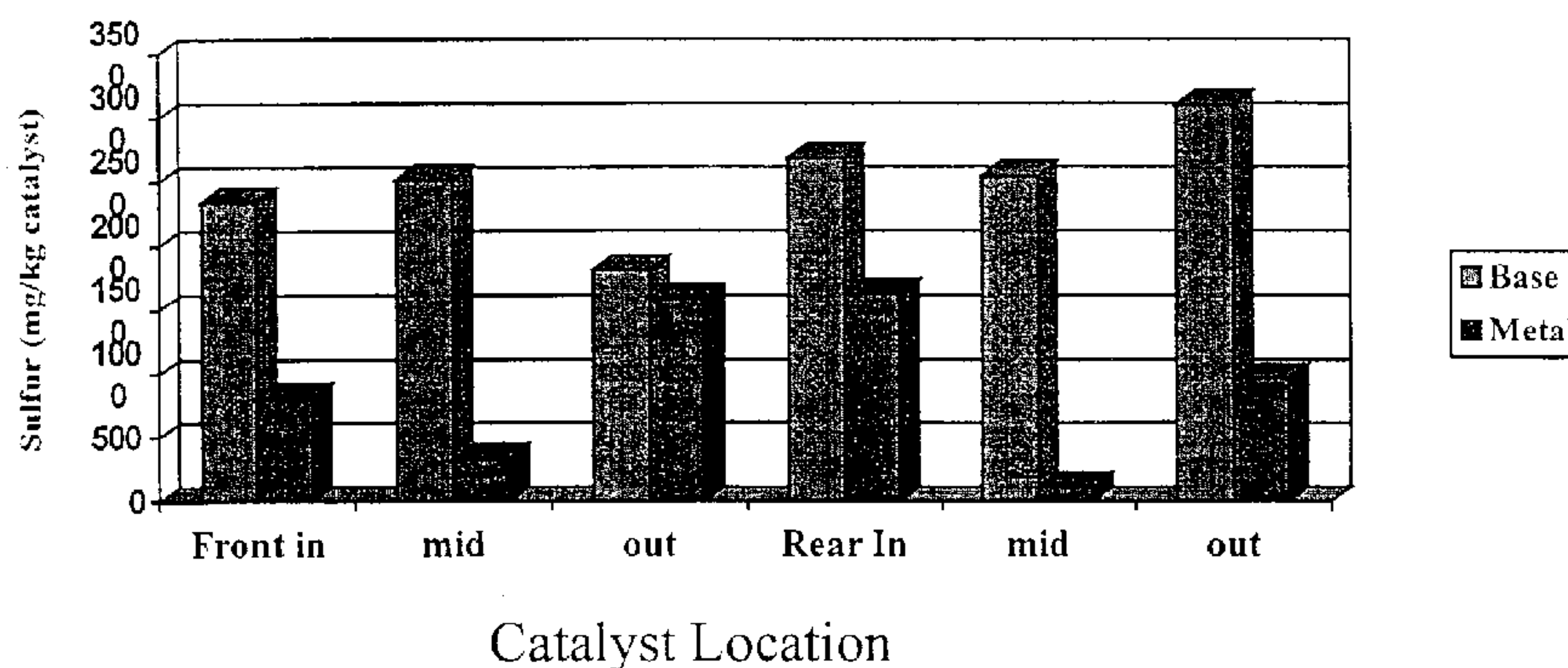
Sulfur Content on Diesel Oxidation Catalyst
