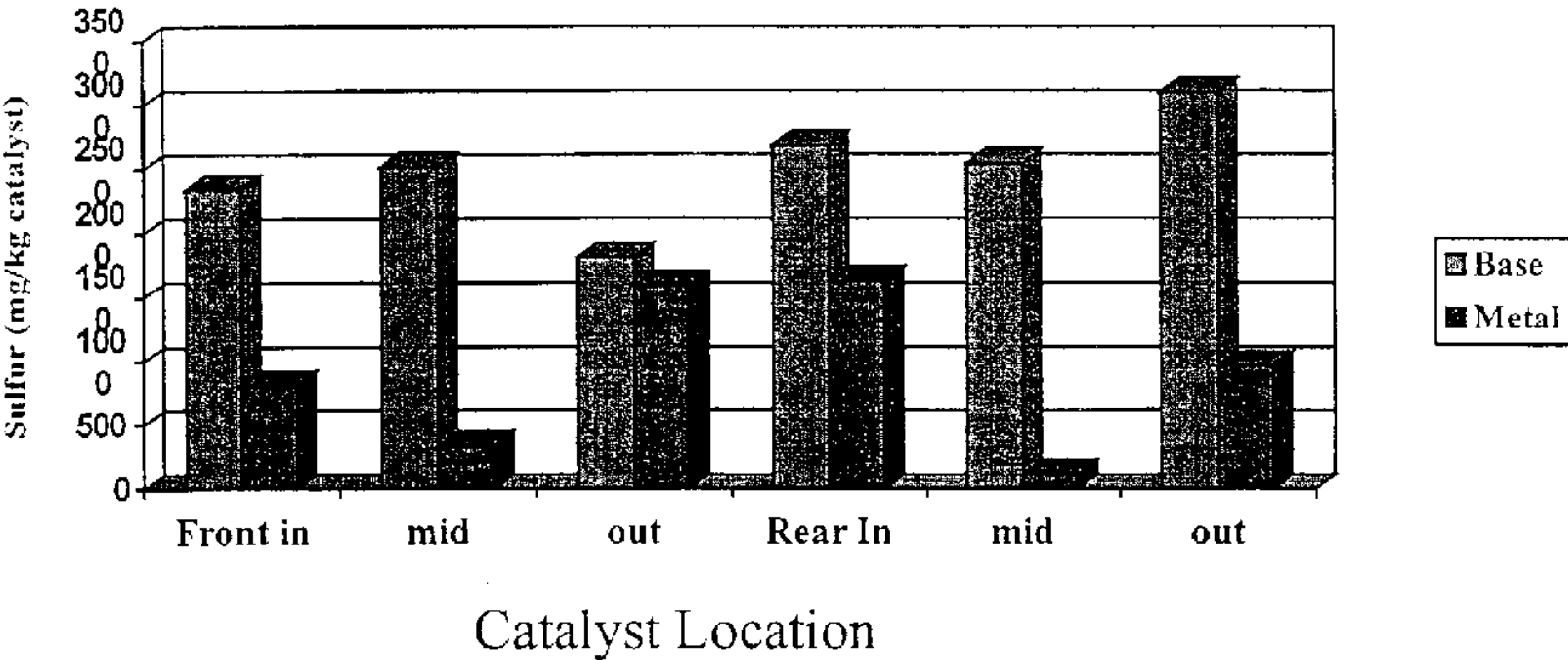
Sulfur Content on Diesel Oxidation Catalyst
