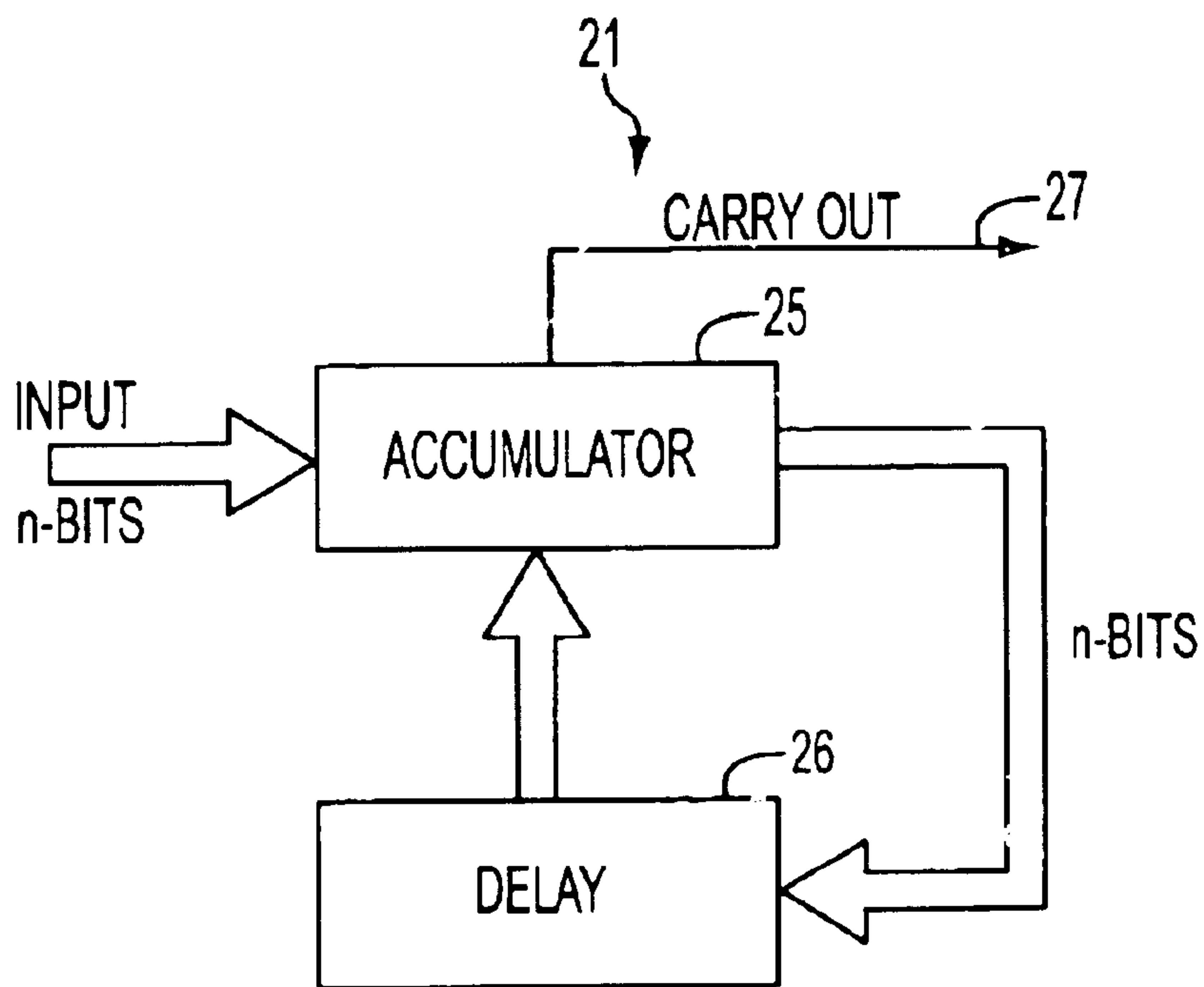
FIG. 2 (PRIOR ART)
