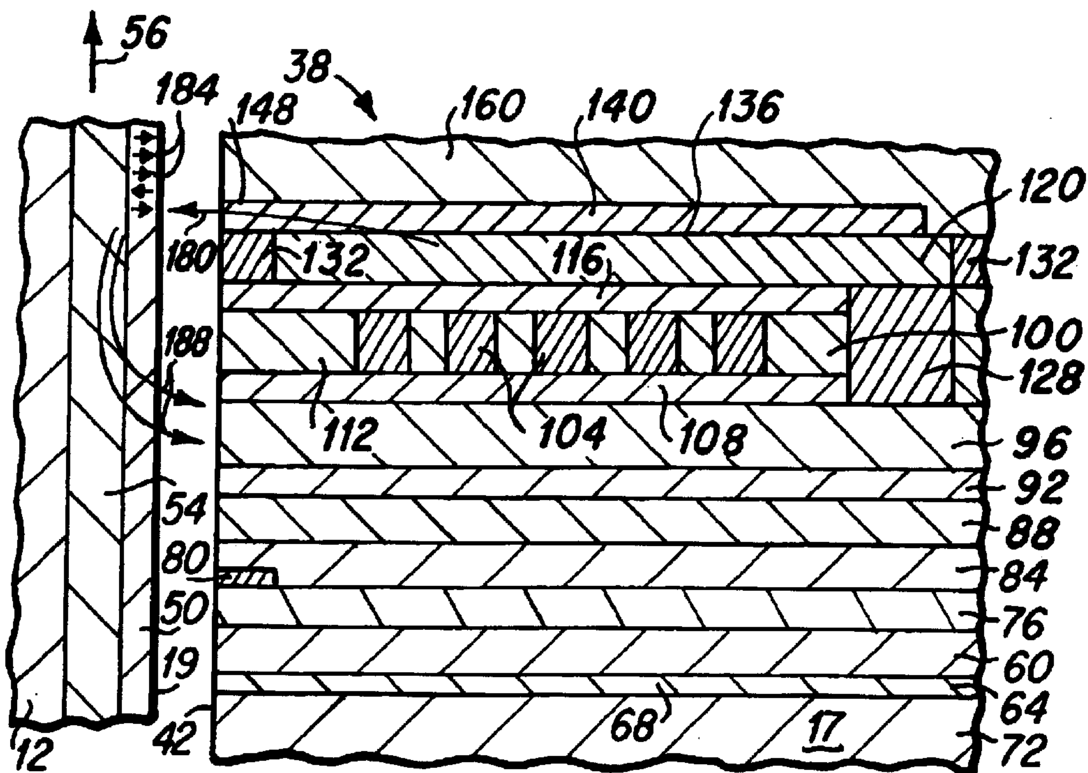
Fig. 2 (PRIOR ART)
