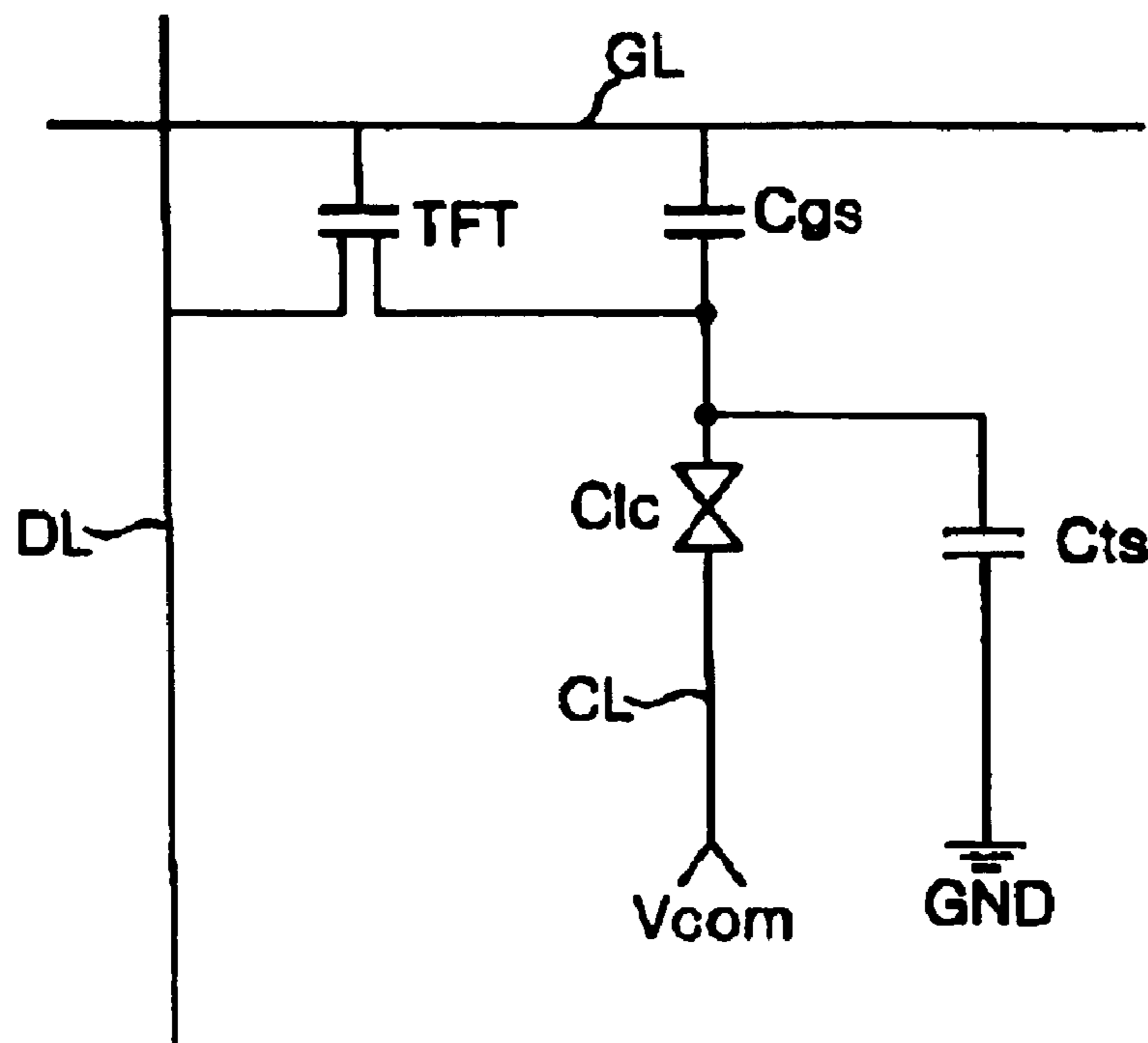
FIG. 6 CONVENTIONAL ART
