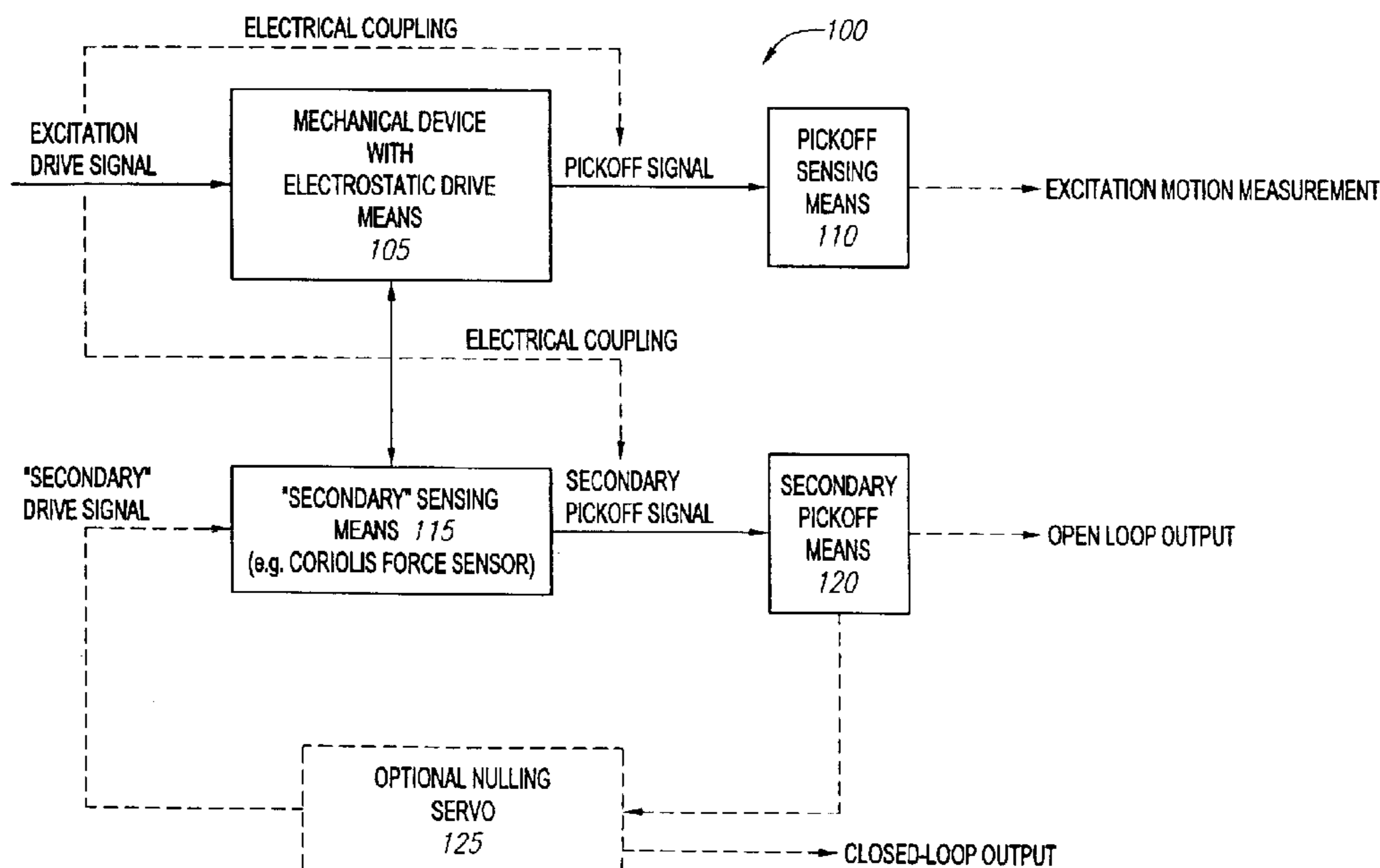
BLOCK DIAGRAM OF EXCITATION & SENSING
