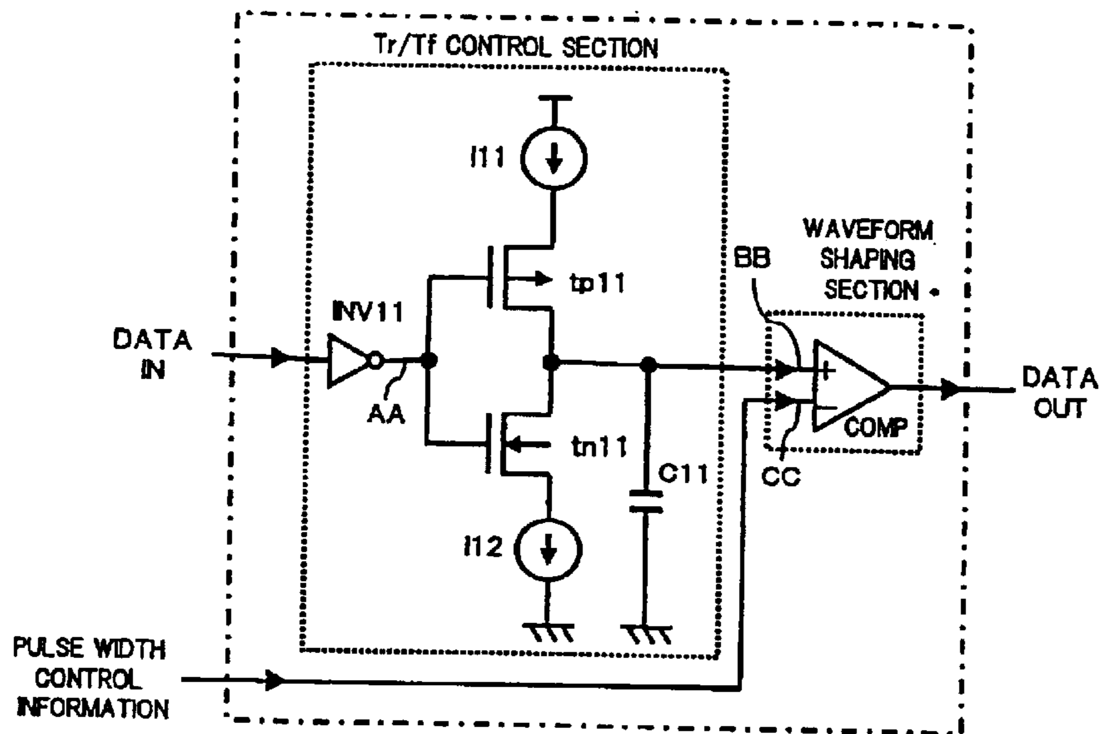
CONVENTIONAL PULSE WIDTH CONTROL CIRCUIT
