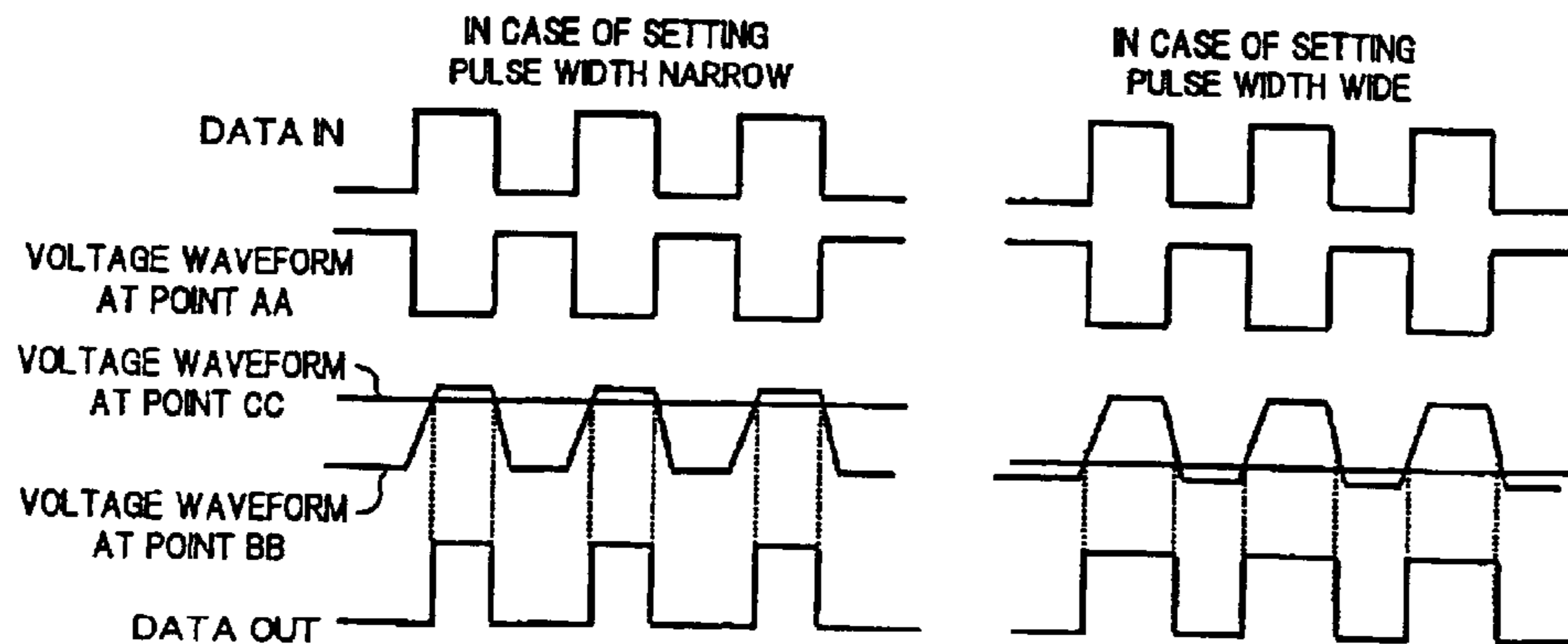
OPERATION OF CONVENTIONAL PULSE WIDTH CONTROL CIRCUIT
