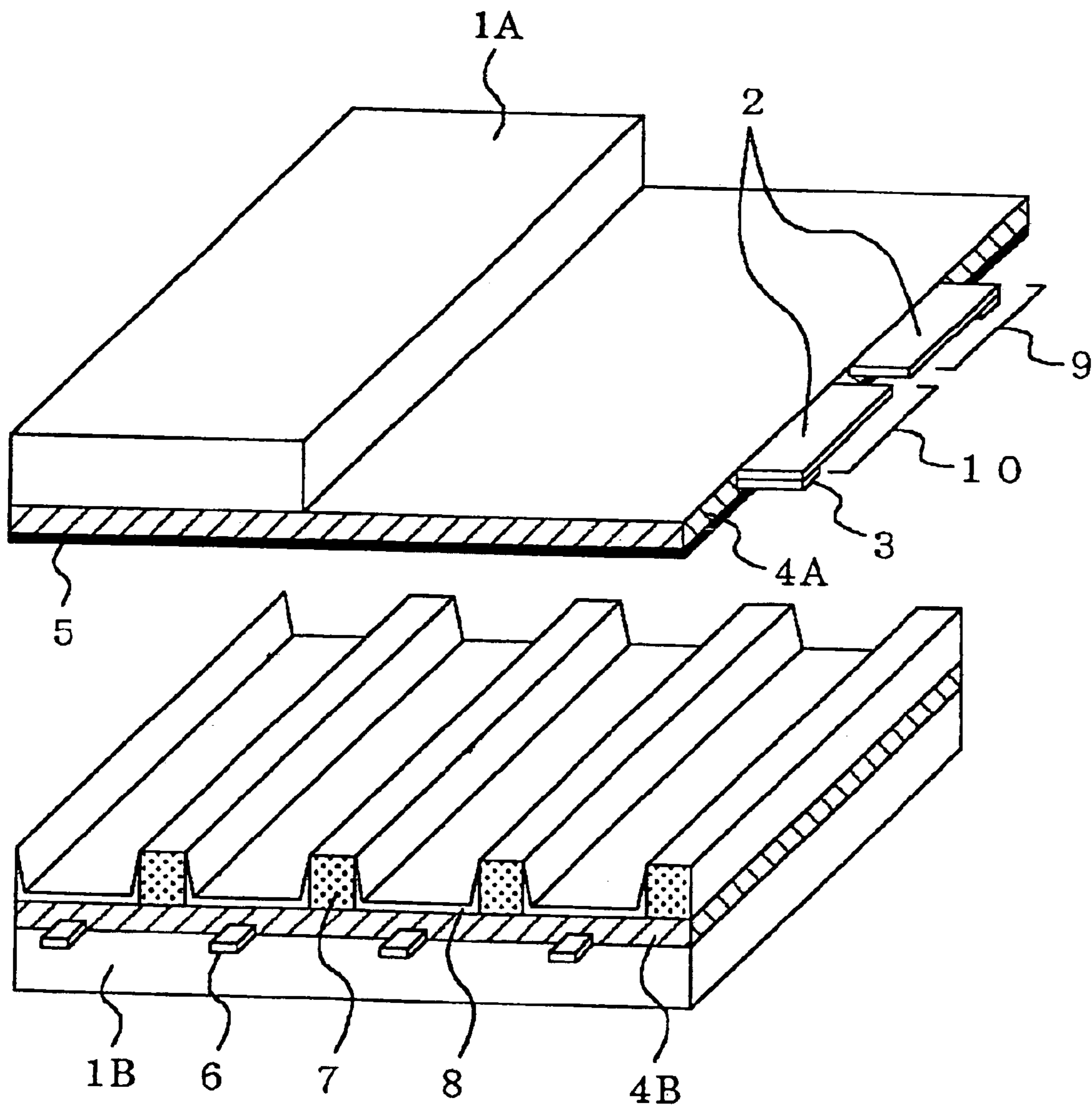
FIG. 1 PRIOR ART
