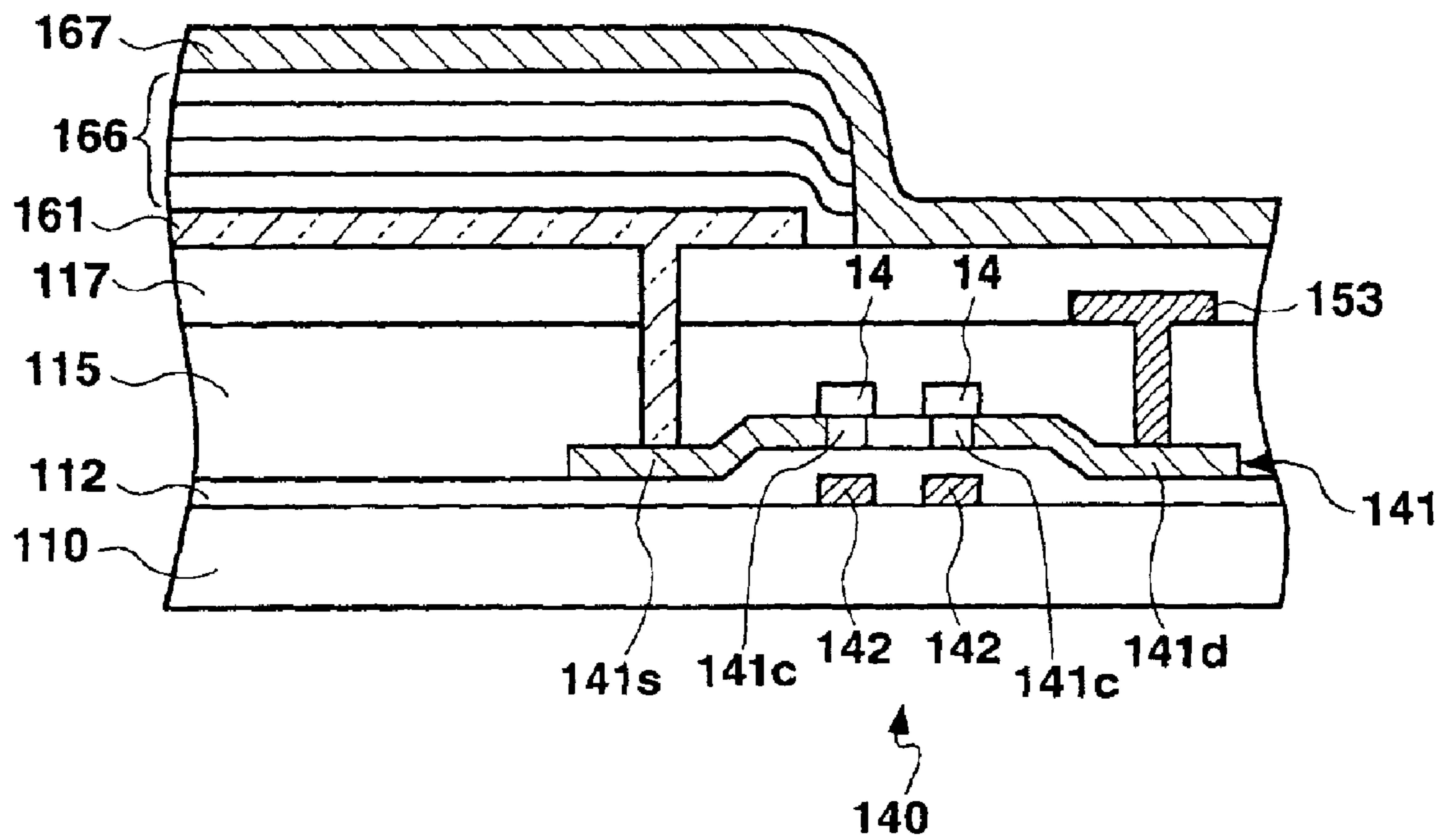
Fig. 3 RELATED ART
