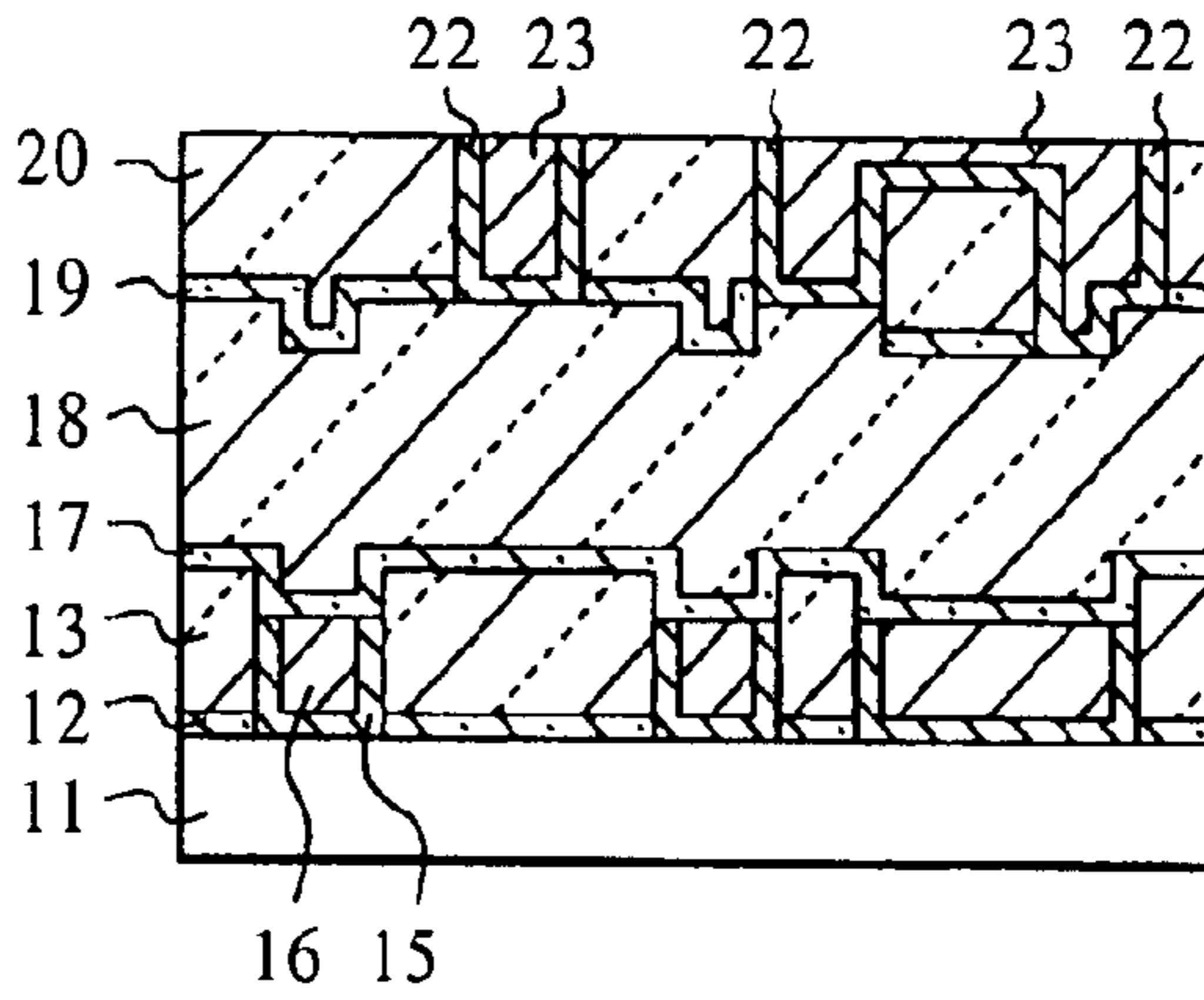
FIG. 13F PRIOR ART
