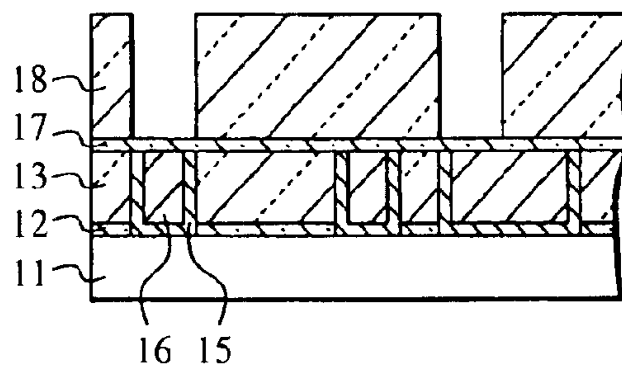
FIG. 14B PRIOR ART
