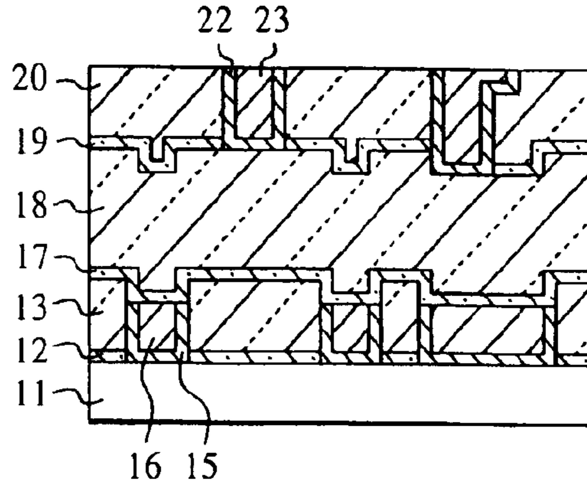
FIG. 13E PRIOR ART
