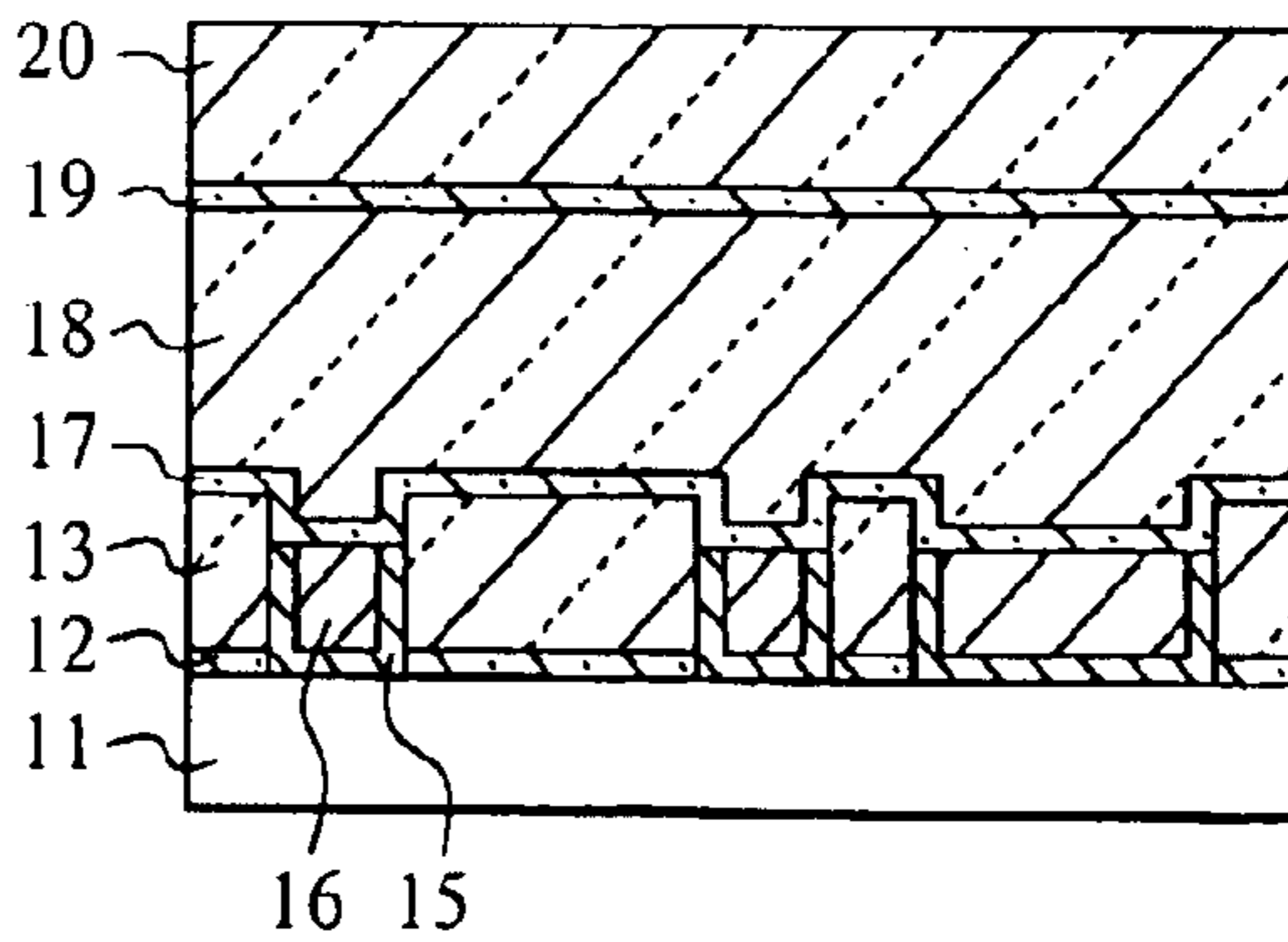
FIG. 13G PRIOR ART
