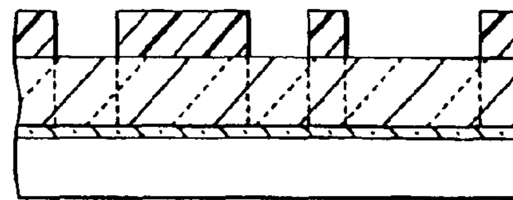
NONEFFECTIVE WAFER AREA (PERIPHERAL WAFER AREA)
