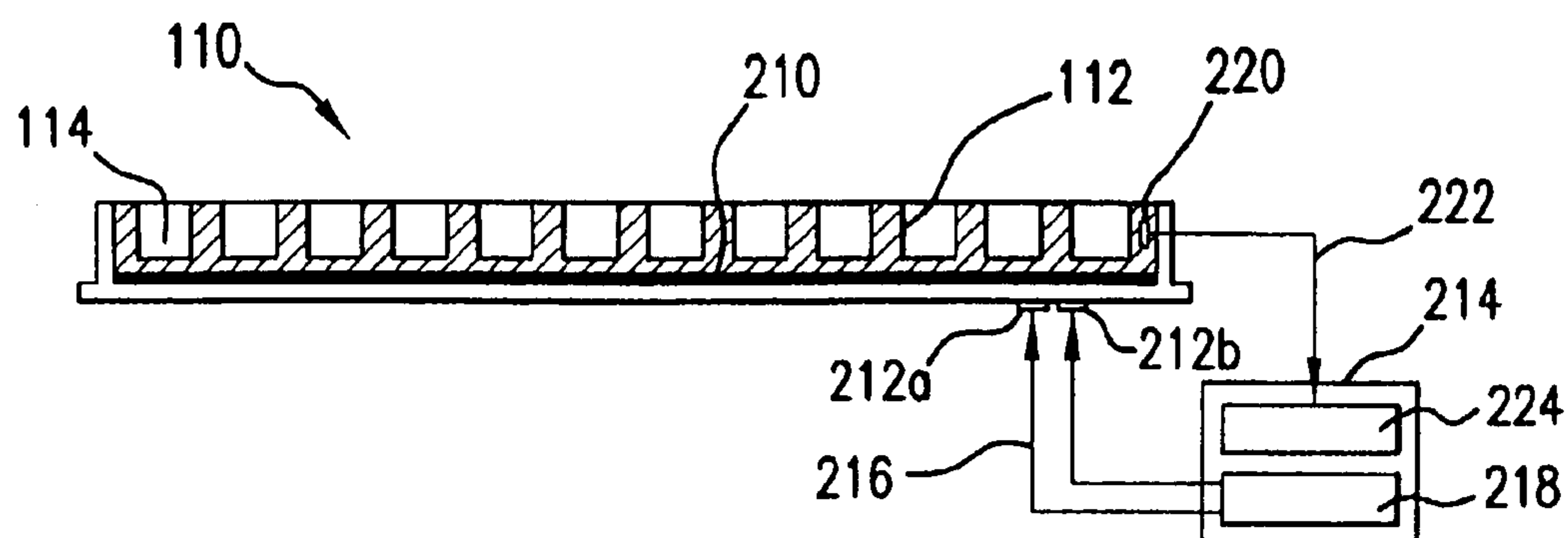
SECTION VIEW A-A' WITH CONTROLLER
