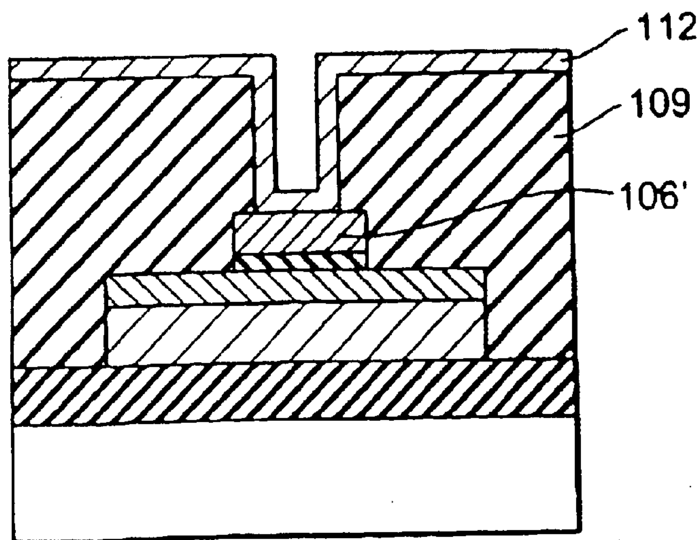
Fig.3I RELATED ART
