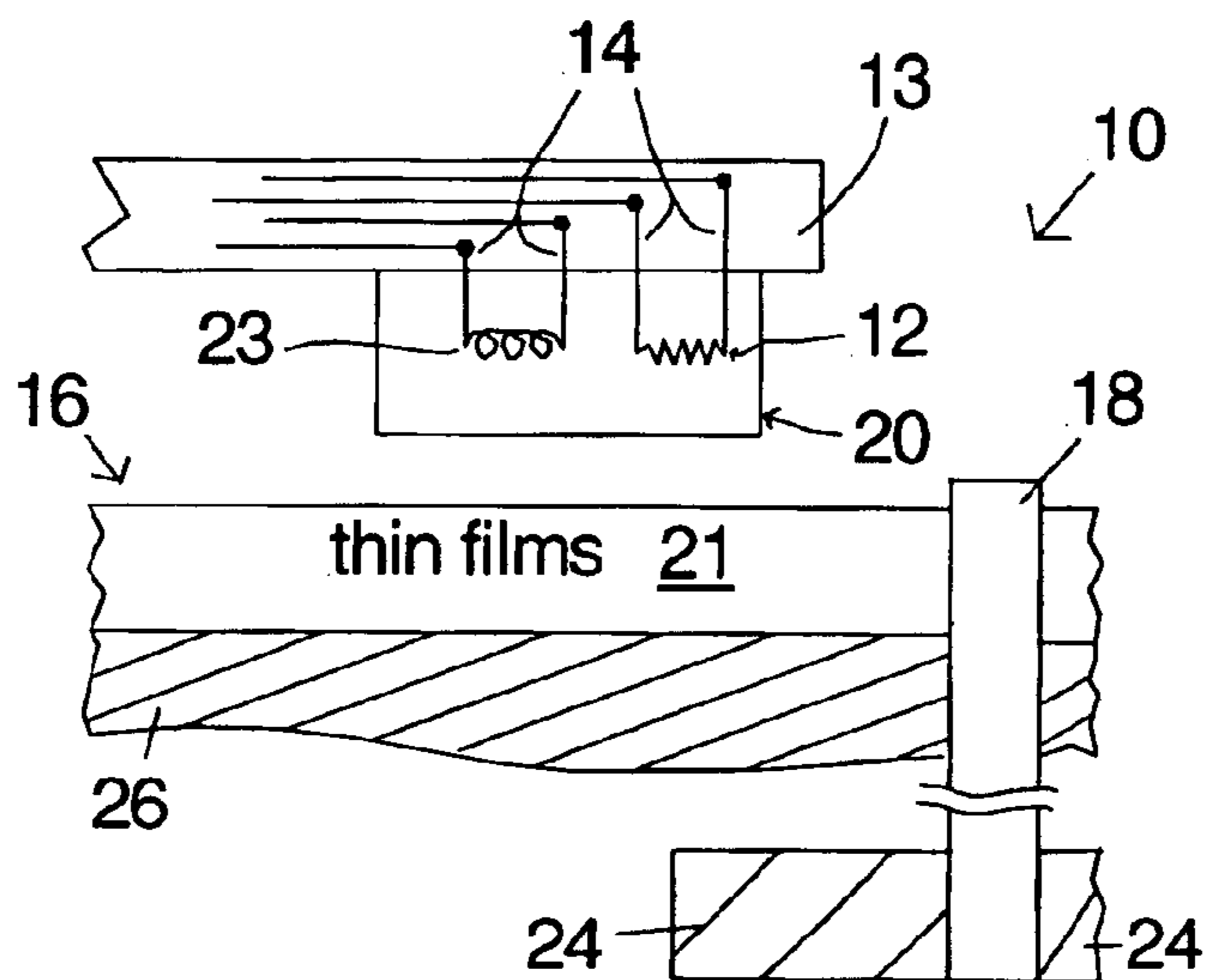
Fig. 1 (Prior Art)
