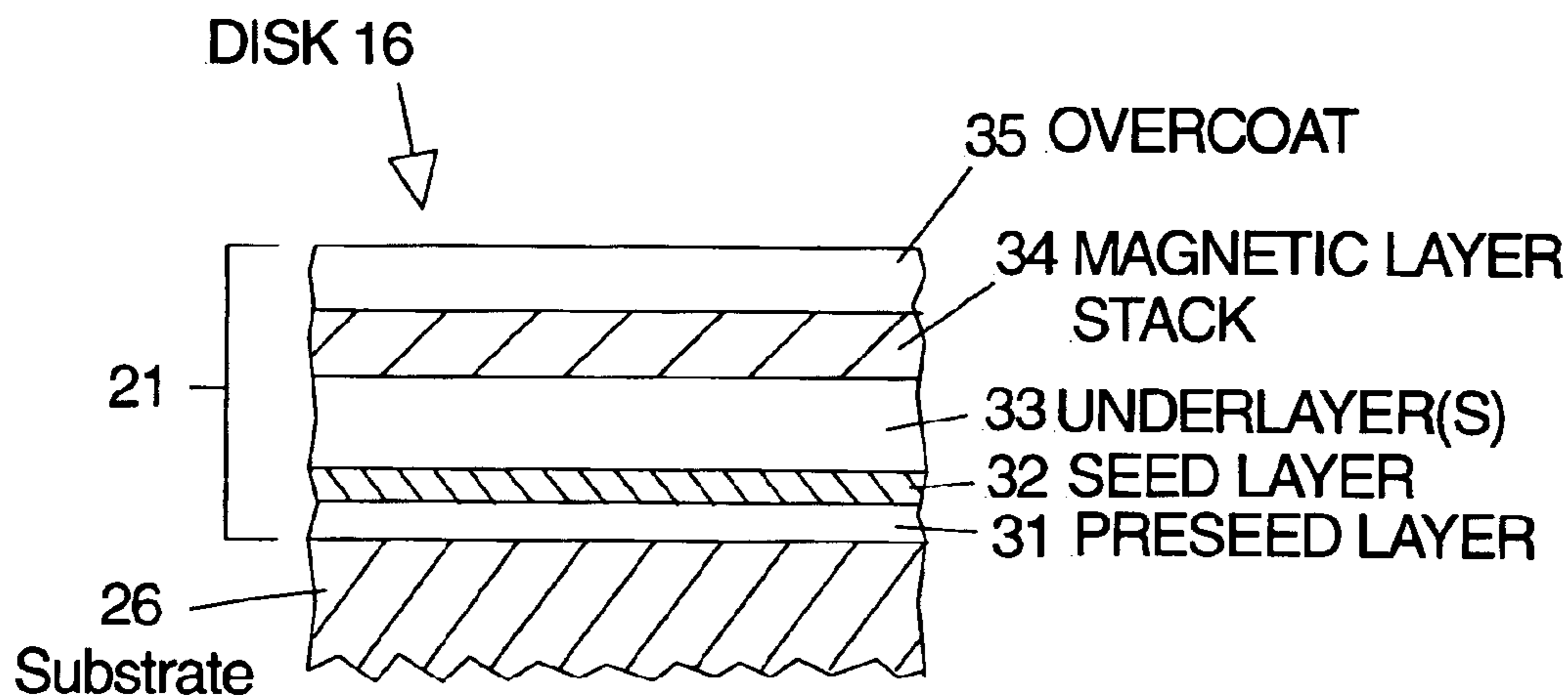
Fig. 2 (Prior Art)
