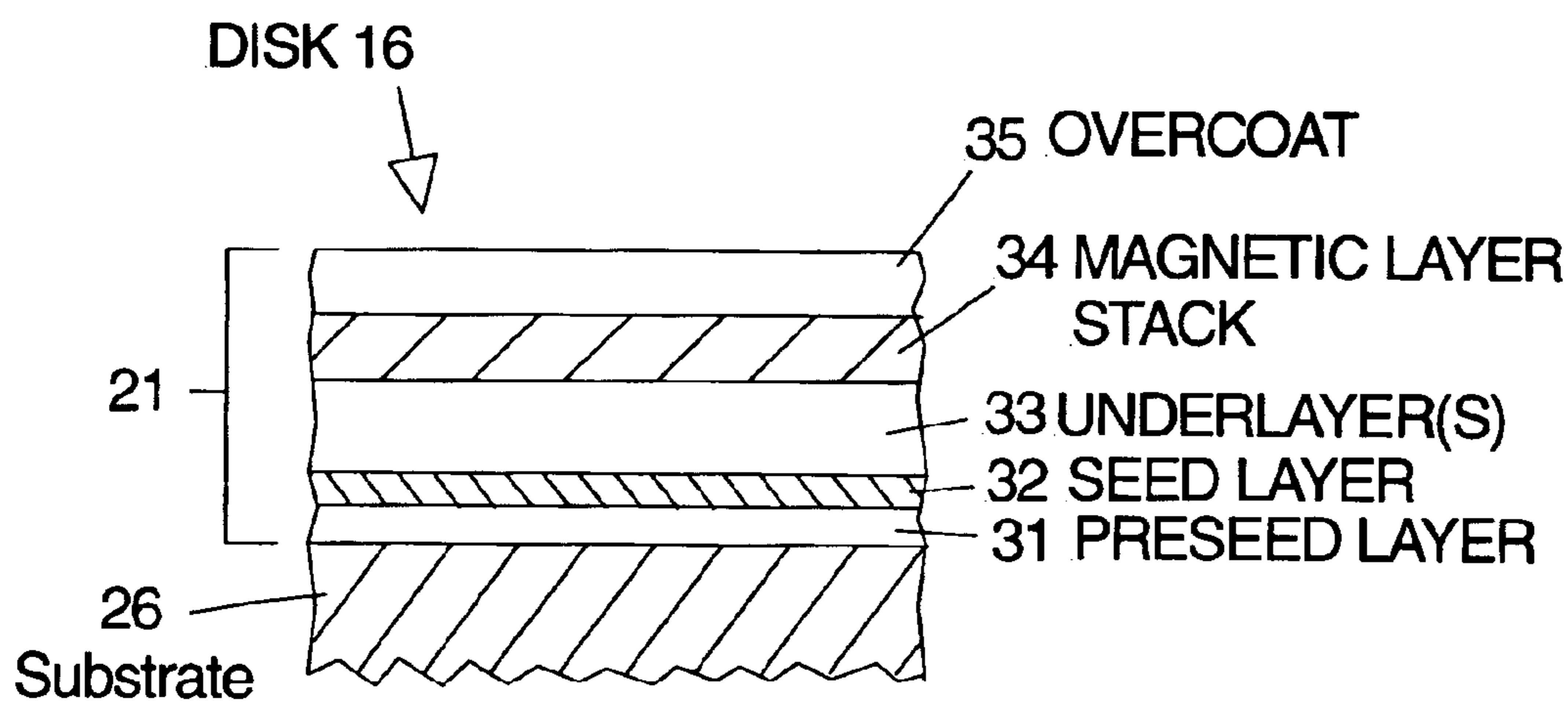
Fig. 2 (Prior Art)
