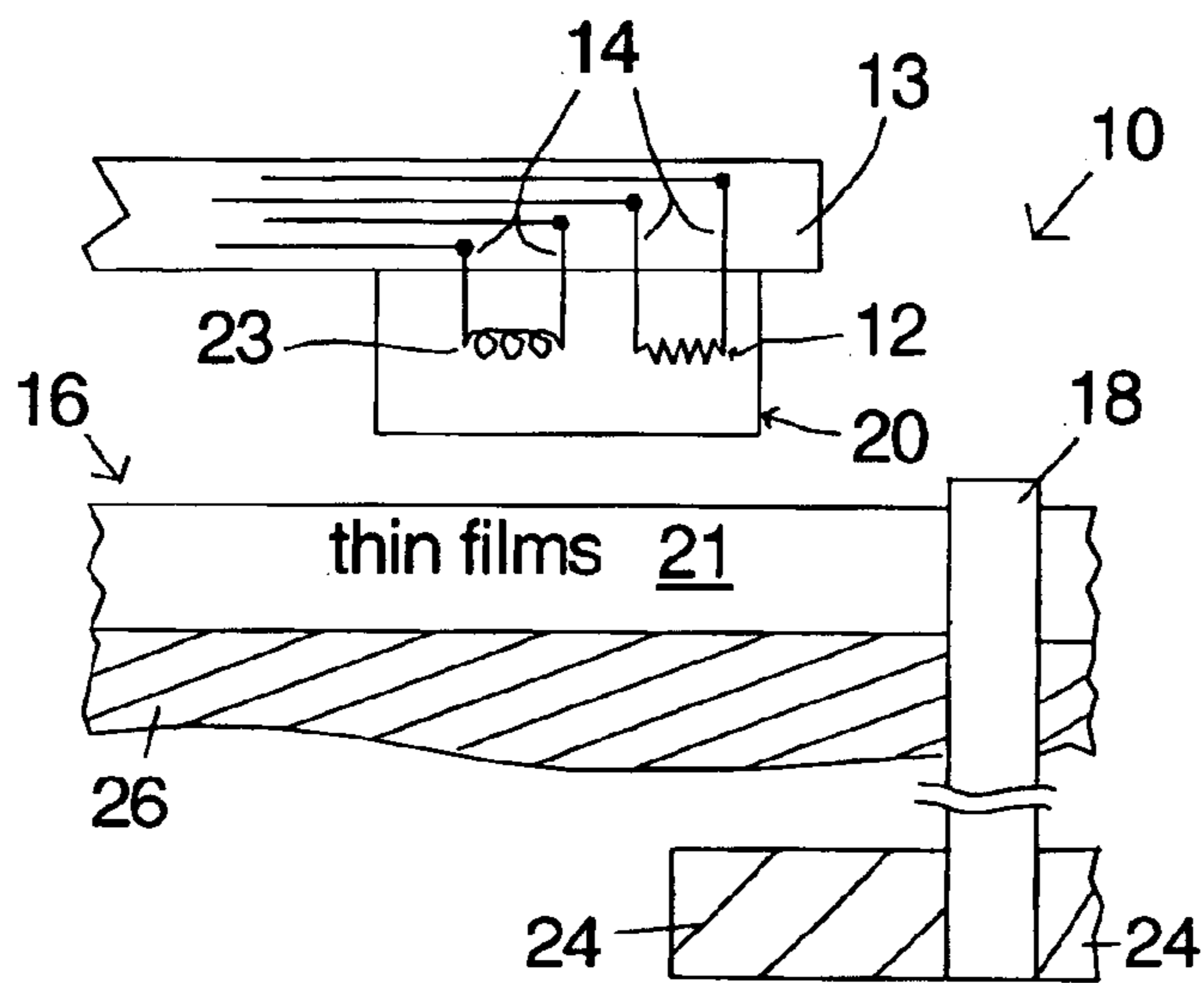
Fig. 1 (Prior Art)
