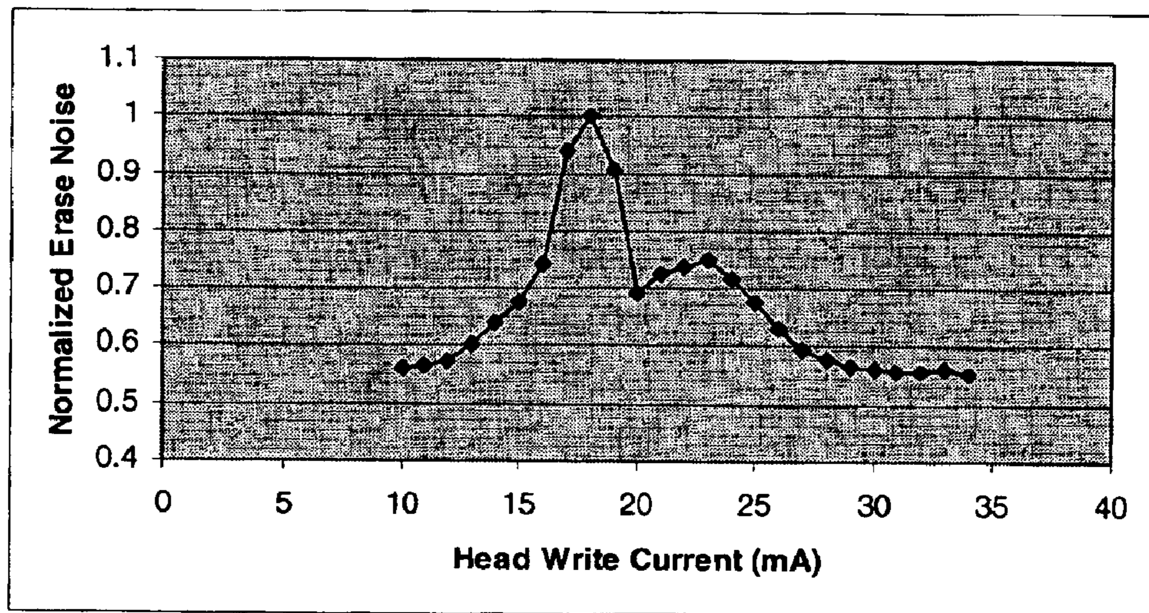
Fig. 6 (Prior Art)
