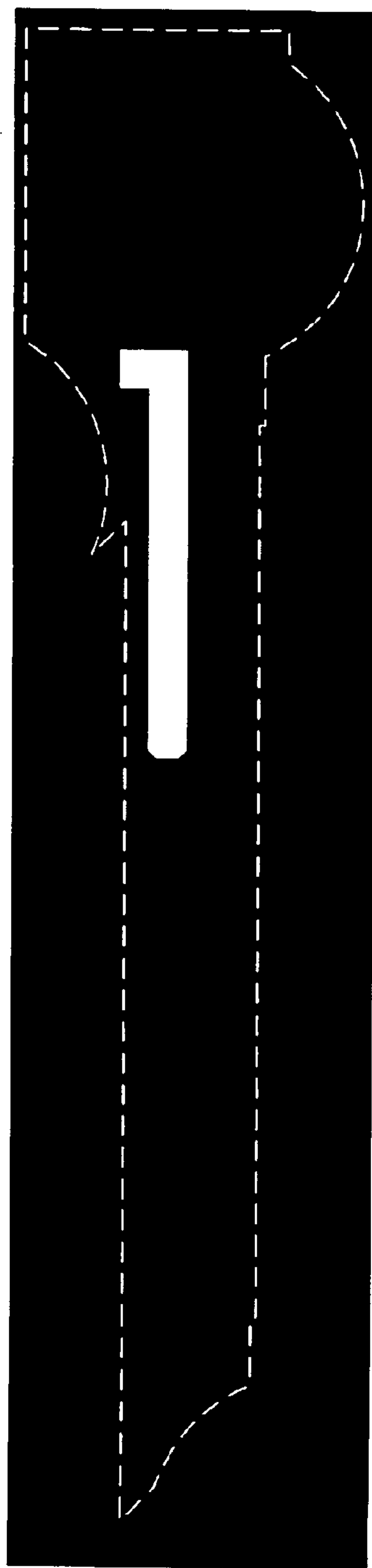
N-Well mask
