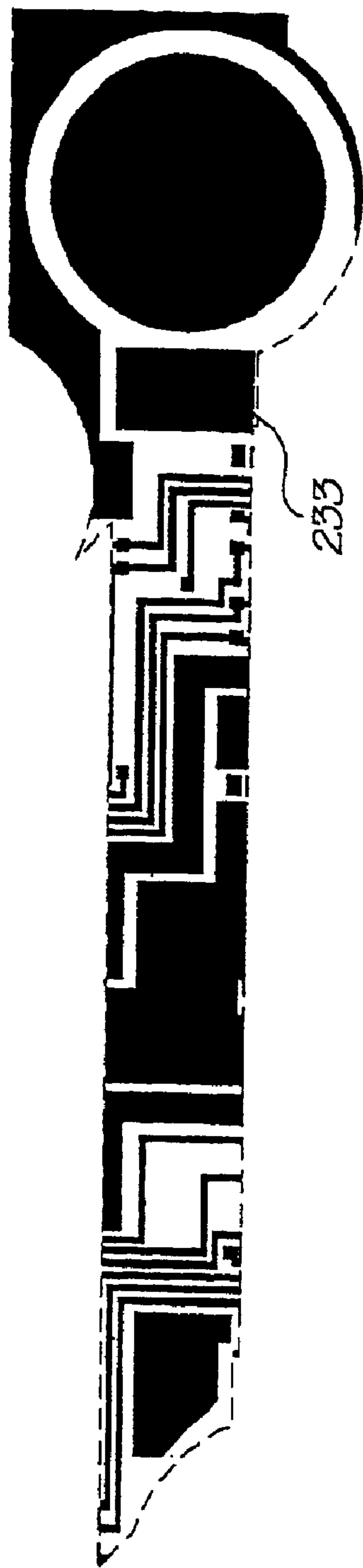
Metal 2 mask
