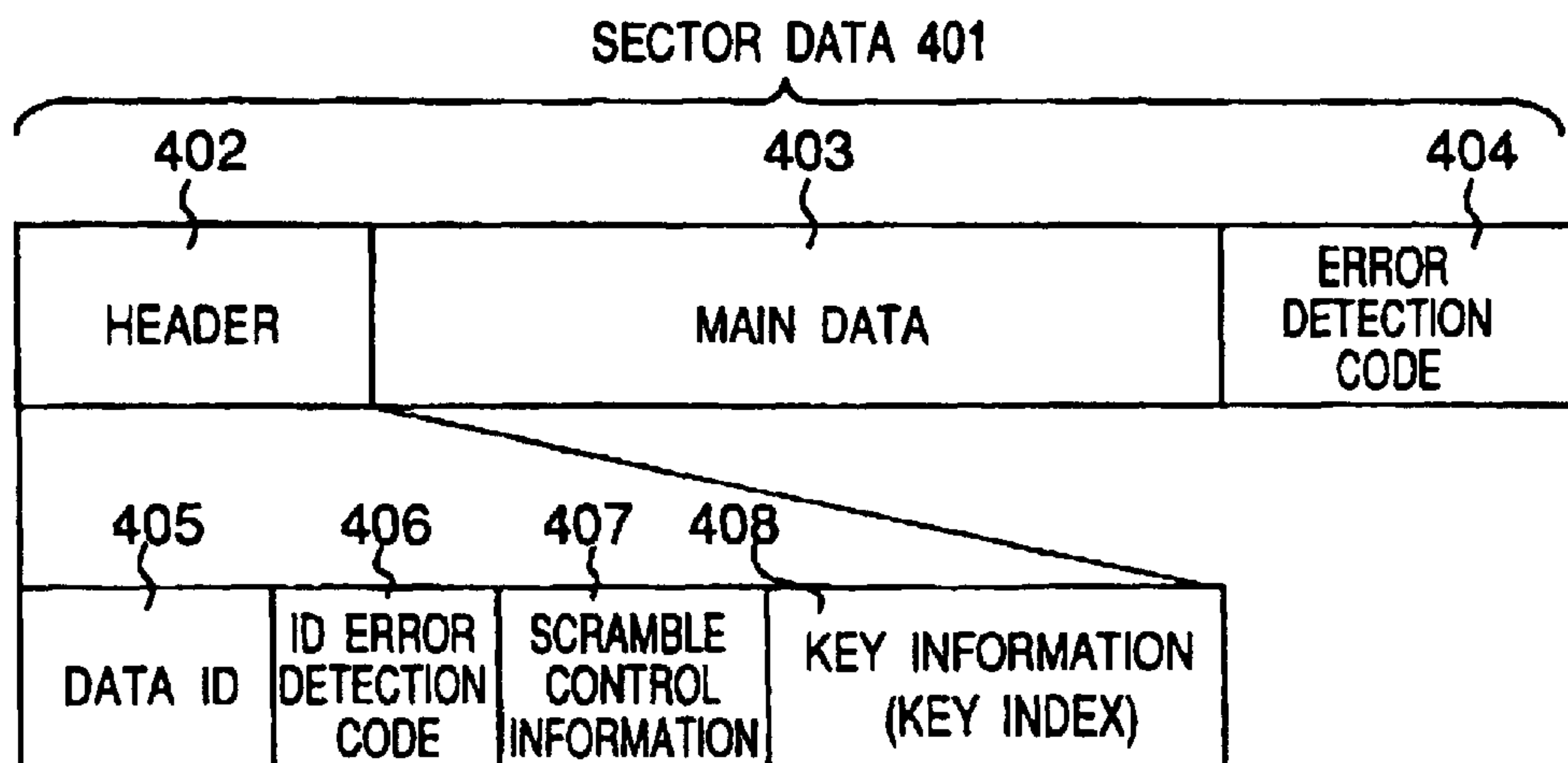
SECTOR STRUCTURE OF SECTOR DATA 401 IN USER DATA AREA 102
